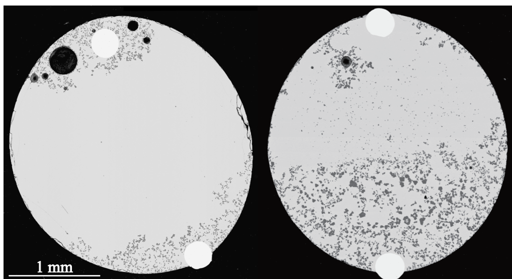
Fig. 3.2. Backscattered electron (BSE) images of the starting material heated at 1500°C for 18 hours in air ( left ) and of the samples heated at 1390°C for 5 hours at P_{\text{H}_2\text{O}} = 5 \times 10^{-2} \text{ Pa} ( right ). The regions with brighter and darker contrasts are glass and spinel, respectively.
