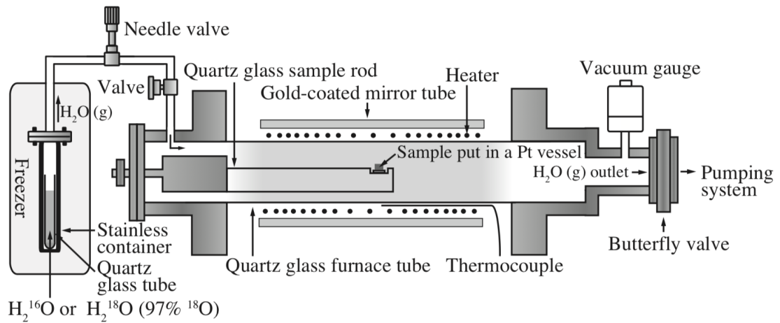
Fig. 2.1. A schematic illustration of the vacuum furnace configuration.
