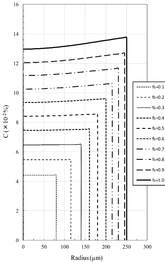
Fig. 3.10 Transition of C in the solid during the growth of a dendrite. C in the liquid was increased according to the model predictions. ( C^o/0.15\% , C_s^*/0.138\% , D = 6.6 \times 10^{-10} \text{ m}^2/\text{s} , solidification time = 213 s, dendrite diameter = 500 \mu\text{m} ).
