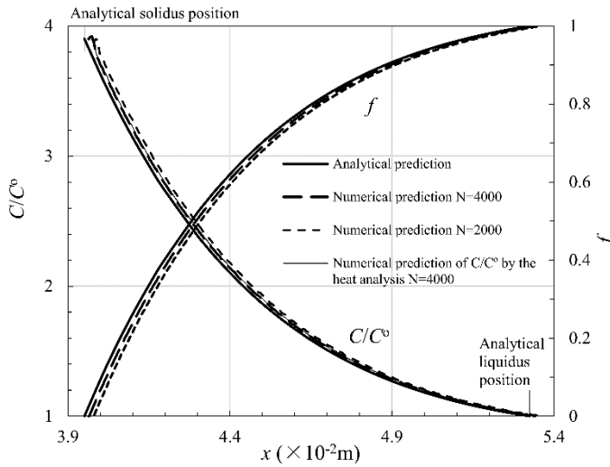
Fig. 3.3 Solute concentration C/C^0 and liquid fraction predicted by the model and numerical analysis of a continuously cast steel. (0.15% C, T^s = 1423 \text{ K} (1150 °C), \Delta T = 15 \text{ K} (15 °C), t = 240 \text{ s} , slab thickness = 0.22 m, N = partitioning number of the half thickness of a slab).
