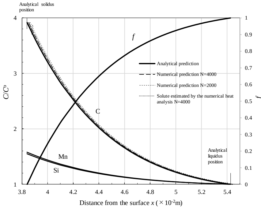
Fig. 4.4 Solute concentration and liquid fraction predicted by the model and numerical analysis of the continuously cast steel K ( T^s = 1423 K, \Delta T = 15 K, t = 240 s, slab thickness = 22 \times 10^{-2} m, and N = partition number of the half thickness of a slab. In this figure, [P] is accounted for but not [S]).
