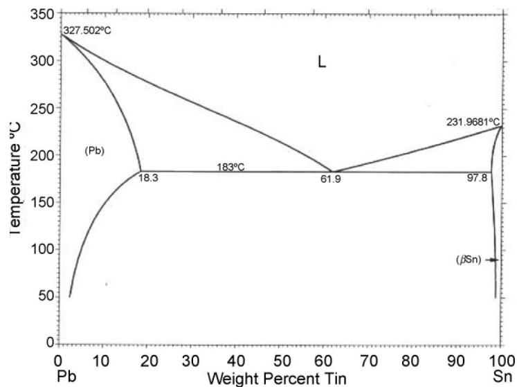
Fig. 5.8. Phase diagram of Pb-Sn binary alloy [8].
