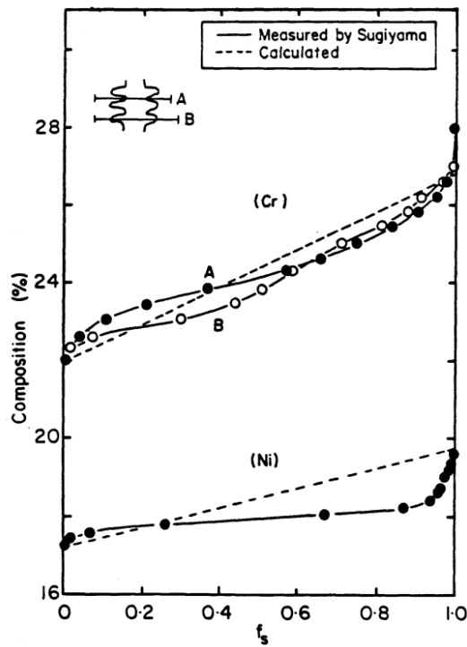
Fig. 2.6 Measured [29] and calculated Cr and Ni compositions as a function of fraction solid in stainless steel(0.08%C,25.6%Cr,19.1%Ni). (A: Section between neighboring secondary dendrite arms. B: Section close to the axis of the secondary dendrite arm.)
