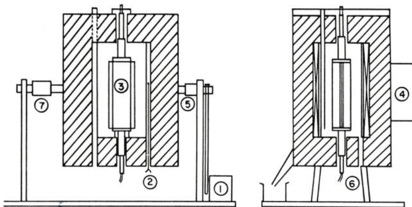
Fig. 5.6 Schematic diagram of rotary furnace: (1) motor (2) chromel-alumel thermocouple (3) mould (4) ice cold junction (5) water inlet (6) water outlet (7) slip ring for thermocouple and power supply [5].
