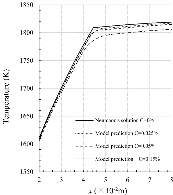
Fig. 3.4 Transitions of temperature predicted by the model and the Neumann' solution ( C=0\% ) of a continuously cast steel. ( C=0\%–0.15\% , T^s = 1423 K (1150 °C), \Delta T = 15 K (15 °C), t = 240 s, slab thickness = 0.22 m).
