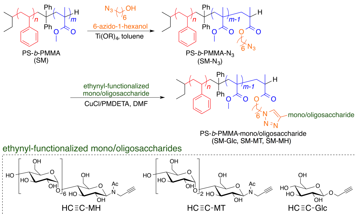
Scheme 4.1. Synthesis of PS- b -PMMA bearing mono/oligosaccharides at their PMMA chain ends by terminal-selective transesterification and click chemistry
