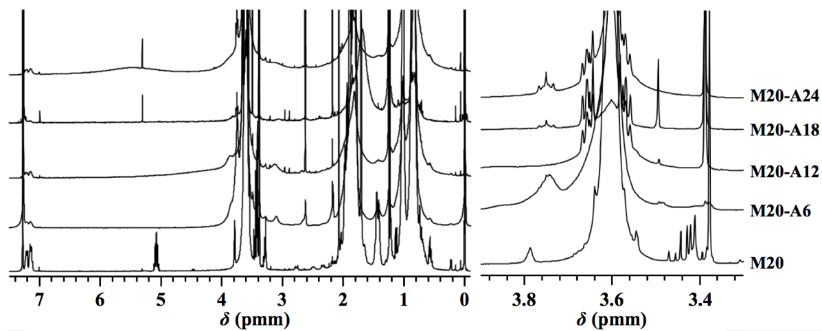
Figure S2.19. 1 H NMR spectra of M20, M20-A6, M20-A12, M20-A18, and M20-A24 in CDCl 3 (400 MHz).
