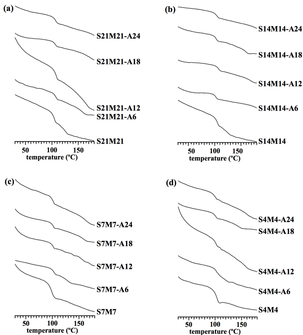
Figure S2.10. DSC curves of the ethanolamine-modified PS- b -PMMA (a: S21M21-AY , b: S14M14-AY , c: S7M7-AY , and d: S4M4-AY ) during second heating under a nitrogen atmosphere at heating rate of 10 °C min -1 .
