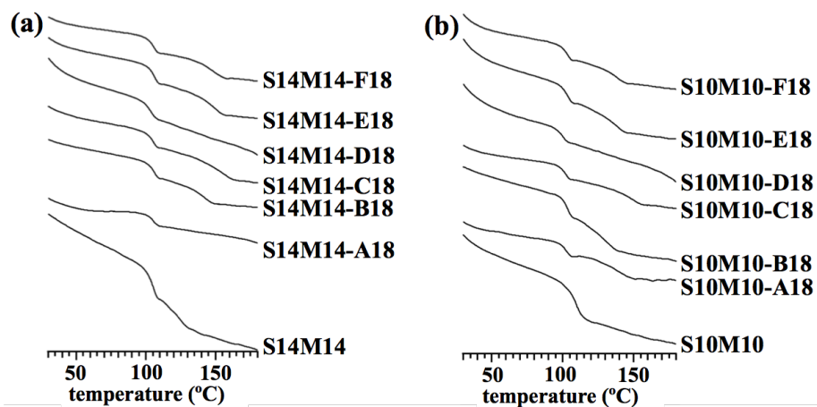
Figure S2.16. DSC curves of the various amine-modified PS- b -PMMAAs (a: S14M14-X18 and b: S10M10-X18) during second heating under a nitrogen atmosphere at heating rate of 10\text{ }^\circ\text{C min}^{-1} .
