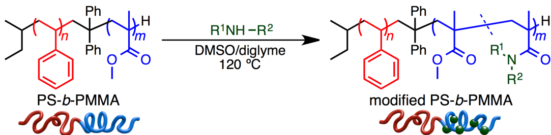
Scheme 2.1. Ester-amide exchange reaction of PS- b -PMMA with various amines
