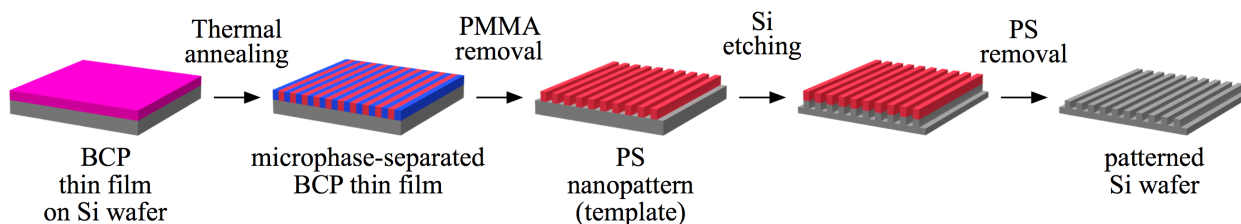
Figure 1.4. Schematic illustration of the BCP lithography process.
