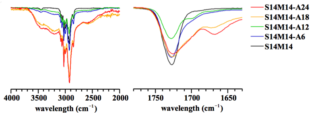
Figure S2.3. FT-IR spectra of S14M14 (black), S14M14-A6 (blue), S14M14-A12 (green), S14M14-A18 (yellow), and S14M14-A24 (red).
