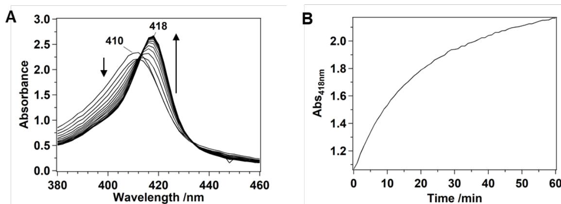
Fig. 10. Determination of the reduction rate of heme. (A) Absorption spectra of heme-K164H after the addition of 1 mM ascorbic acid at pH 8.0 under a CO atmosphere. (B) Time course of absorbance changes at 418 nm.
