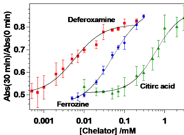
Fig. 3 Changes in absorbance at 406 nm during heme degradation by HutZ in the presence of DFO, citric acid, or ferrozine. The data points in UV-vis spectra were obtained before addition of ascorbic acid (1 mM) and 30 min after addition. Abs(30 min)/Abs(0 min) values are plotted against iron chelator concentration, and the data were fit to the Hill equation.
