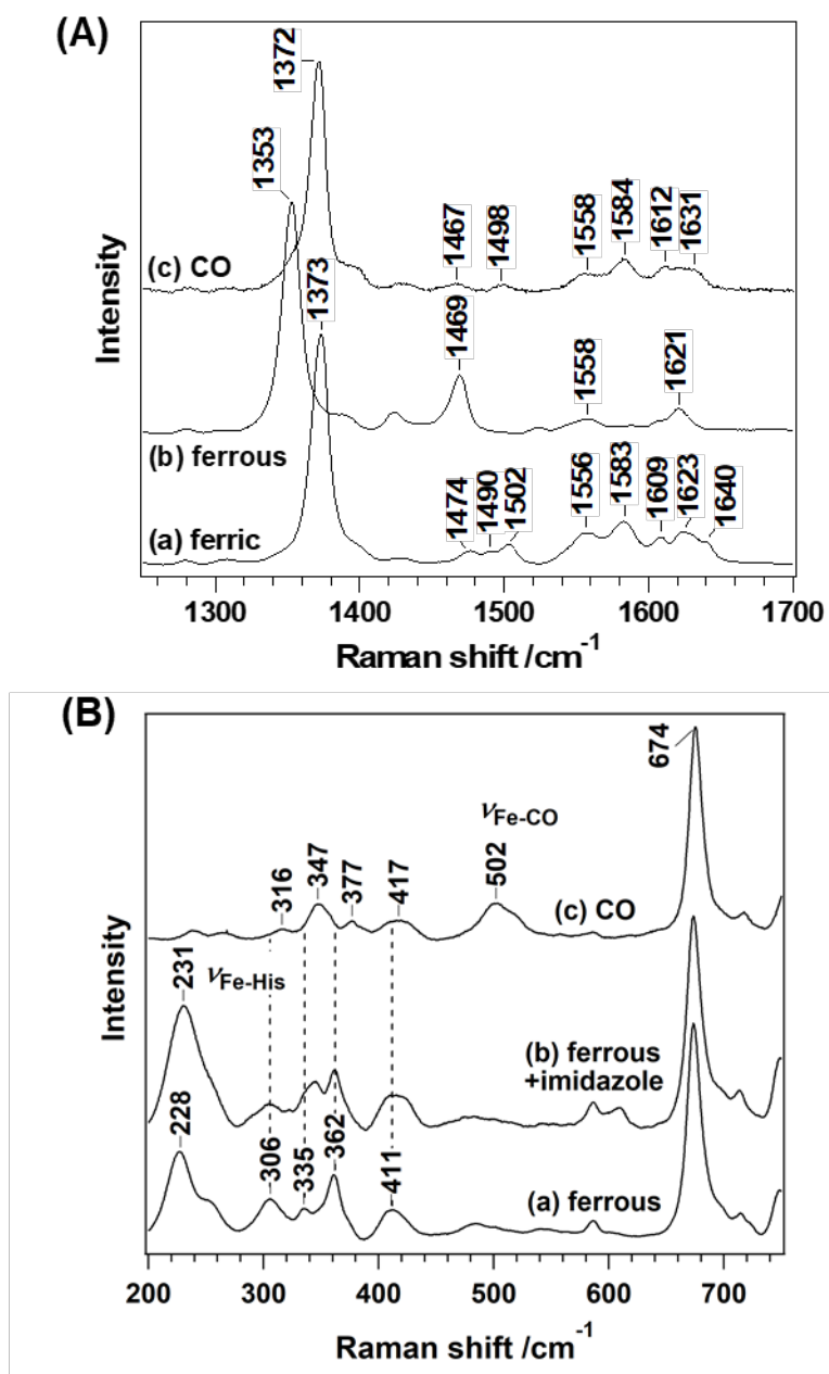
Fig. 12: Resonance Raman spectra of the H170A mutant. The protein concentration was 10 \mu\text{M} in 50 mM Tris-HC/150 mM NaCl, pH 8.0. (A) High-frequency region; (B) low-frequency region. The excitation wavelength for ferric and CO-bound forms was 413.1 nm, and that for the ferrous form was 441.6 nm.
