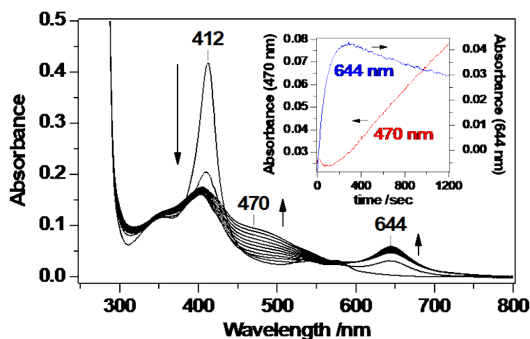
Fig. 5 Reaction of ferric heme-HutZ with \text{H}_2\text{O}_2 in the presence of 1 mM guaiacol. The inset shows the time courses of the absorbance at 470 and 644 nm. The spectra were measured at 2-min intervals for 30 min after addition of 0.1 mM \text{H}_2\text{O}_2 .
