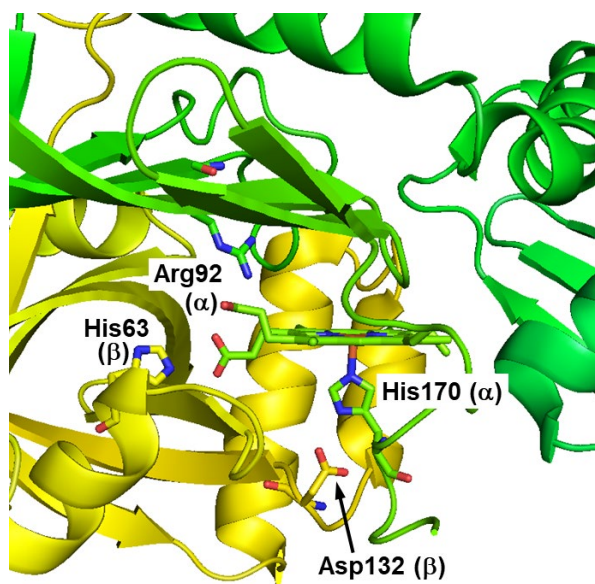
Fig. 1. Crystal structure of HugZ from H. pylori (PDB ID code 3GAS). Residues are numbered according to the amino acid sequence of HutZ from V. cholerae . \alpha and \beta indicate the subunits.
