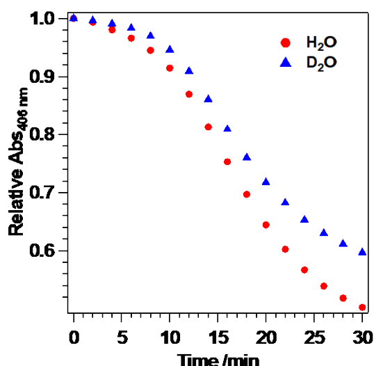
Fig. 11 Isotope effect of the heme-degradation reaction by HutZ. Time course of absorbance change at 406 nm in the reaction with ascorbic acid in H 2 O/D 2 O buffer at pH 6.0.
