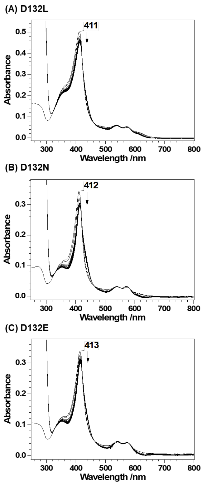
Fig. 5. Heme degradation reaction of the heme-HutZ complex with ascorbic acid (1.0 mM) at pH 8.0. Spectra were measured before addition of ascorbic acid, and at 2-min intervals for 30 min after addition of ascorbic acid. (A) Heme-D132L; (B) heme-D132N; and (C) heme-D132E
