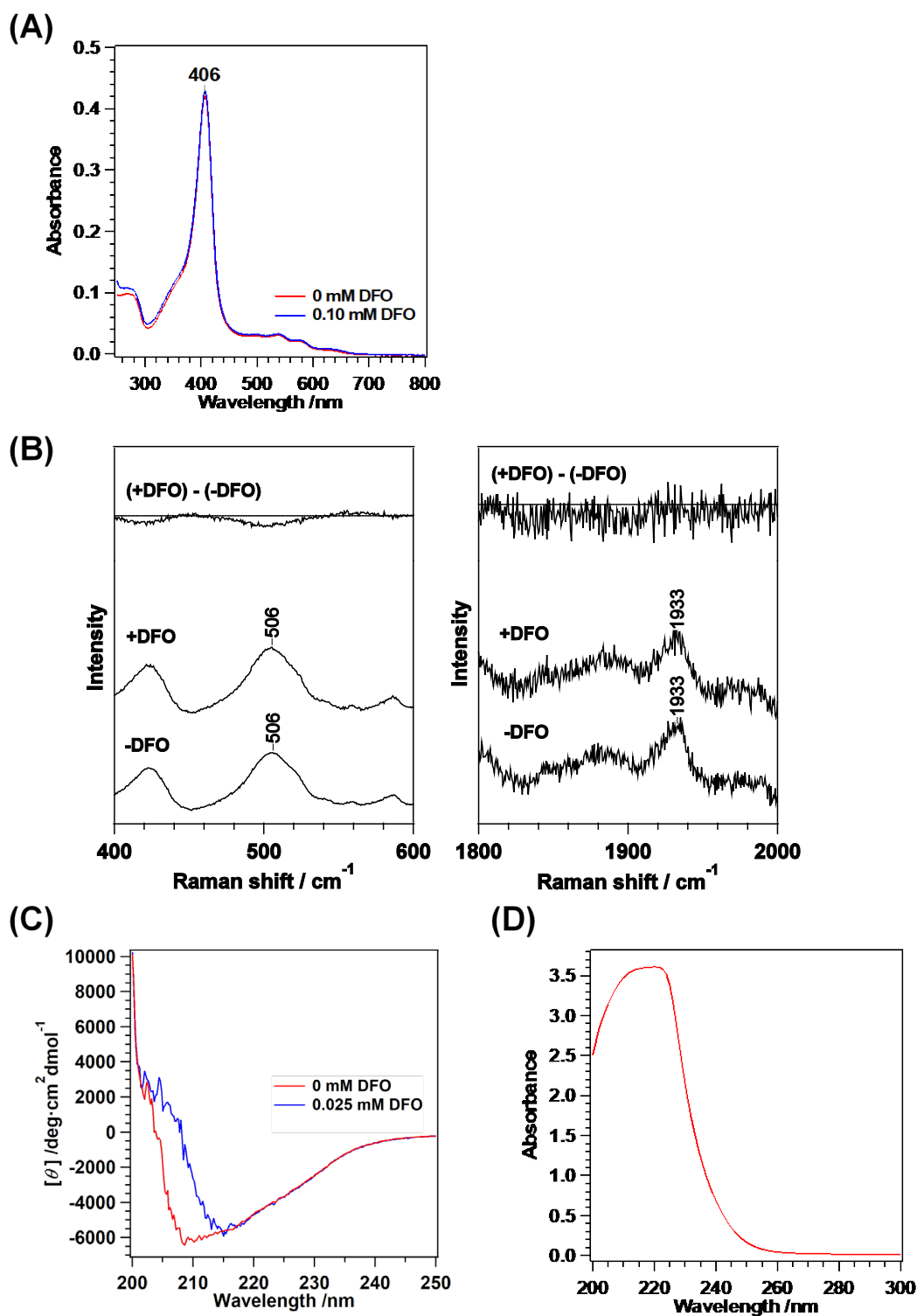
Fig. 4 (A) Absorption spectra of the heme-HutZ in the absence (red) and presence of 0.1 mM DFO (blue). (B) Resonance Raman spectra of the heme-HutZ in the CO-bound form. The protein concentration is 10 mM in 50 mM Tris-HCl/150 mM NaCl (pH 6.0). (C) CD spectra of heme-HutZ in the absence (red) and presence of DFO (blue). Protein concentration was 5.0 \mu\text{M} in 50 mM sodium phosphate/100 mM NaCl. (D) Absorption spectra of 1.0 mM DFO in 50 mM sodium phosphate/100 mM NaCl.
