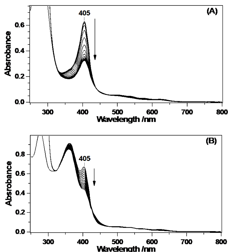
Fig. 15 Heme-degradation reaction of the heme-HutZ complex with ascorbic acid (1.0 mM) at pH 6.0 (A) in the presence of 50 \mu M chloramphenicol and (B) 50 \mu M tetracycline. Spectra were measured before addition of ascorbic acid and at 8-min intervals for 56 min after addition of ascorbic acid. Tetracycline caused a large absorption below 400 nm.
