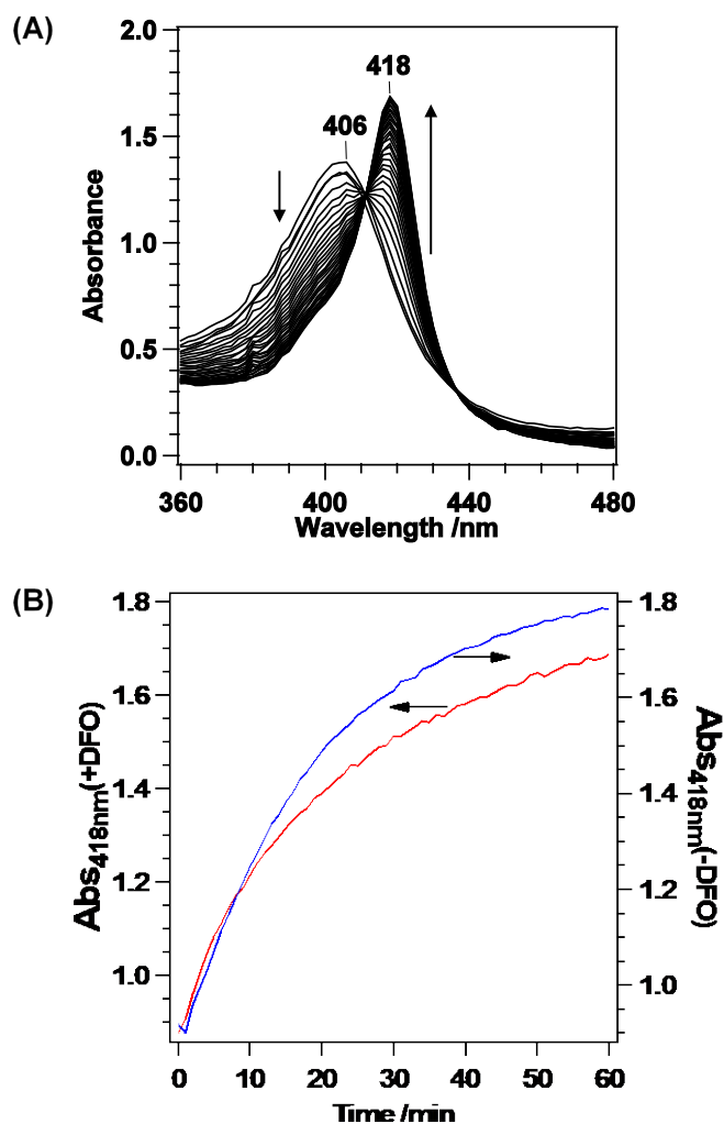
Fig. 7 Determination of reduction rate of heme. (A) UV-vis spectra of heme-HutZ after addition of ascorbic acid (1 mM) in the presence of DFO at pH 6.0 under CO atmosphere. (B) Time course of absorbance change at 418 nm in the presence (red, left axis) and absence (blue, right axis) of DFO.
