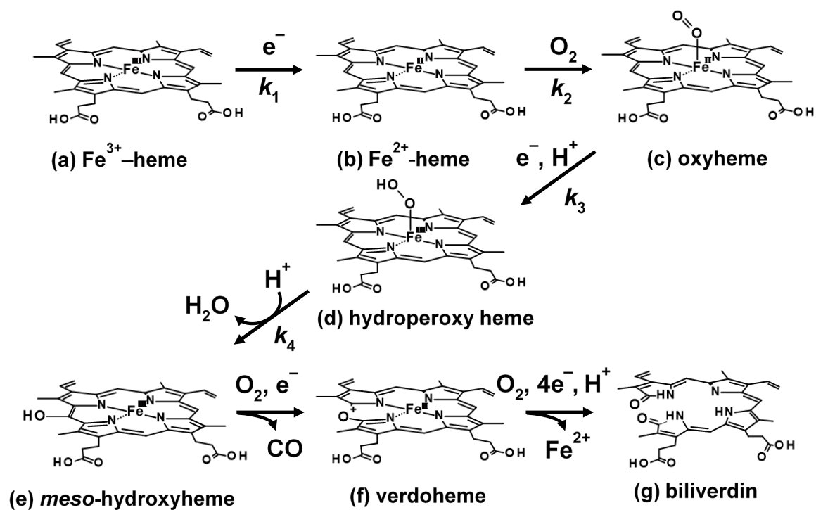
Fig. 6 Heme degradation mechanism in HutZ
