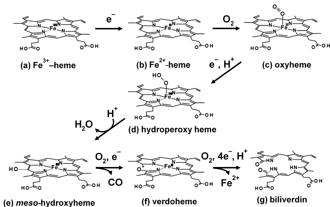
Fig. 1 Proposed heme degradation mechanism of HutZ.
