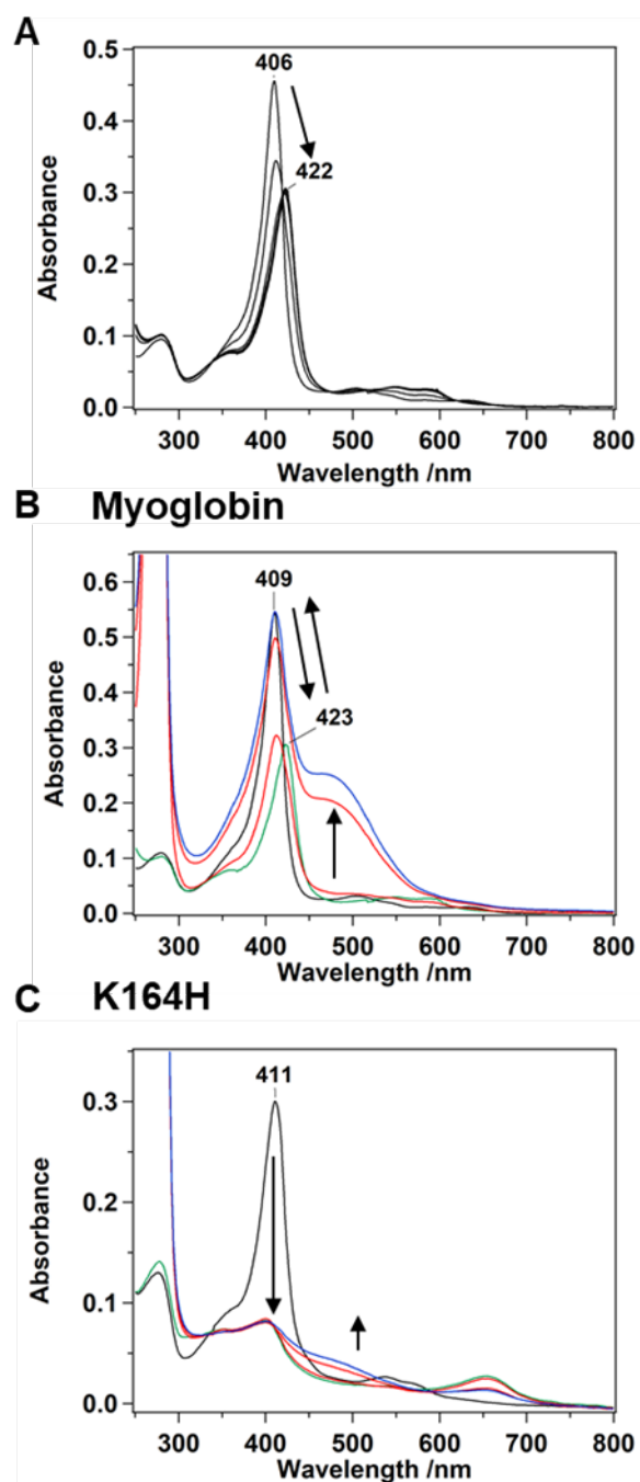
Fig. 5. (A) Absorption spectra of myoglobin in a reaction containing 0.1 mM \text{H}_2\text{O}_2 at pH 8.0. Spectra were measured before the addition of \text{H}_2\text{O}_2 , and at 1-min intervals for 10 min after the addition of \text{H}_2\text{O}_2 . (B, C) Reaction of myoglobin (B) and heme-K164H mutant (C) with \text{H}_2\text{O}_2 (90 \mu\text{M} ) in the presence of 0.45 mM guaiacol at pH 8.0. The absorption spectrum before the reaction is shown as a black line. The reaction with guaiacol was monitored before mixing (green line), and 1, 20 (red lines), and 30 min (blue line) after mixing.
