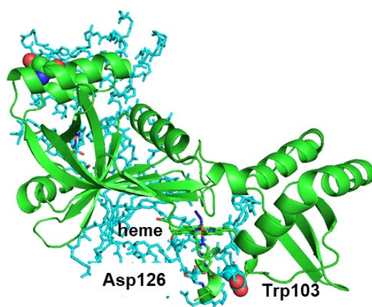
Fig. 12. Location of Trp103 and heme on the HugZ crystal structure (PDB 3GAS). Residues are numbered according to the amino acid sequence of Alr5027 from cyanobacteria Nostoc sp. PCC7120. Green and cyan show each protomer. Trp103 is present in a different protomer (green) from that (cyan) containing the nearby Asp126.
