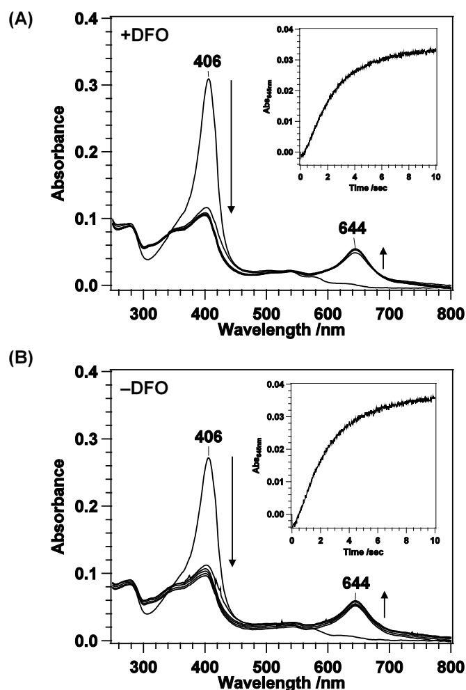
Fig. 9 Heme-degradation reaction of heme-HutZ with \text{H}_2\text{O}_2 (0.10 mM) at pH 6.0 in the presence (A), and absence of DFO (B). Spectra were measured before addition of \text{H}_2\text{O}_2 , and at 1-min intervals for 5 min after addition of \text{H}_2\text{O}_2 . Inset: Time course of absorbance at 644 nm.
