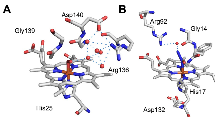
Fig. 2 Crystal structures of (A) rat HO-1 (PDB ID 4G7L) and (B) a HutZ homologous protein HugZ from Helicobacter pylori (3GAS). The residue numbering in (B) is based on V. cholerae HutZ. In HO-1, Asp140 forms a hydrogen bonding network with a water cluster, which is essential for the heme degradation activity of the enzyme. Arg92 in HugZ forms a hydrogen bond with iron-bound azide through a water molecule.
