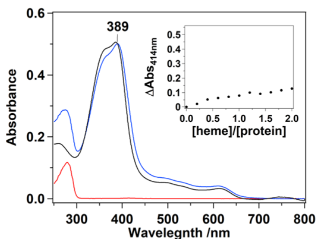
Fig. 3. Absorption spectra of the heme-WT Alr5027 complex. Spectra are for purified apo-Alr5027 (red line), free heme (black line), and heme-Alr5027 (blue line). The inset shows differences at 414 nm following incremental addition of heme (2–30 \mu\text{M} ) to Alr5027 (10 \mu\text{M} ) in 50 mM Tris-HCl and 150 mM NaCl (pH 8.0), measured against a blank cell containing buffer alone.
