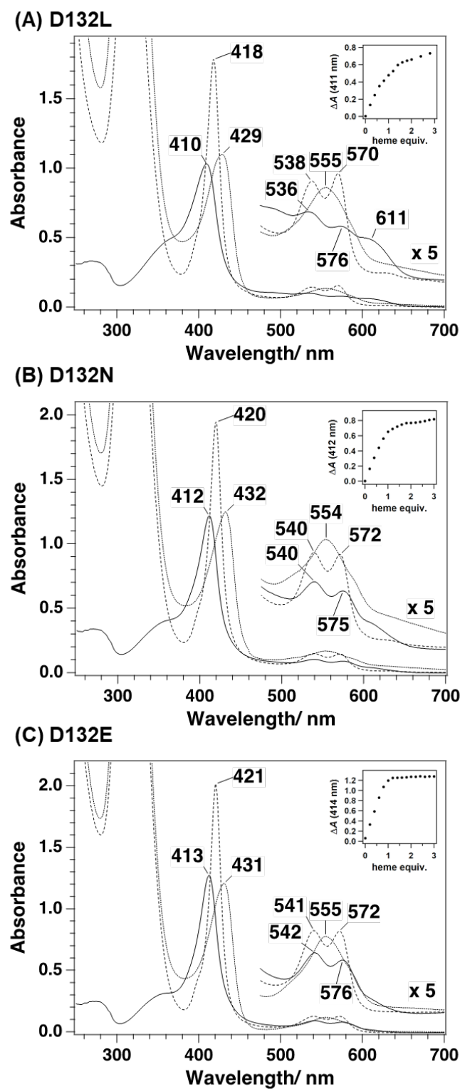
Fig. 2. Absorption spectra of the heme-HutZ complex. The protein concentration was 5 \mu M (on a per heme basis) in 50 mM Tris-HCl/150 mM NaCl, pH 8.0. Spectra shown are in the ferric (solid line), ferrous (dotted line), and CO-bound (dashed line) forms. Inset: Heme-binding curve generated from difference absorbance spectra by plotting \Delta A versus the molar ratios of heme to the protein. (A) Heme-D132L; (B) heme-D132N; and (C) heme-D132E.
