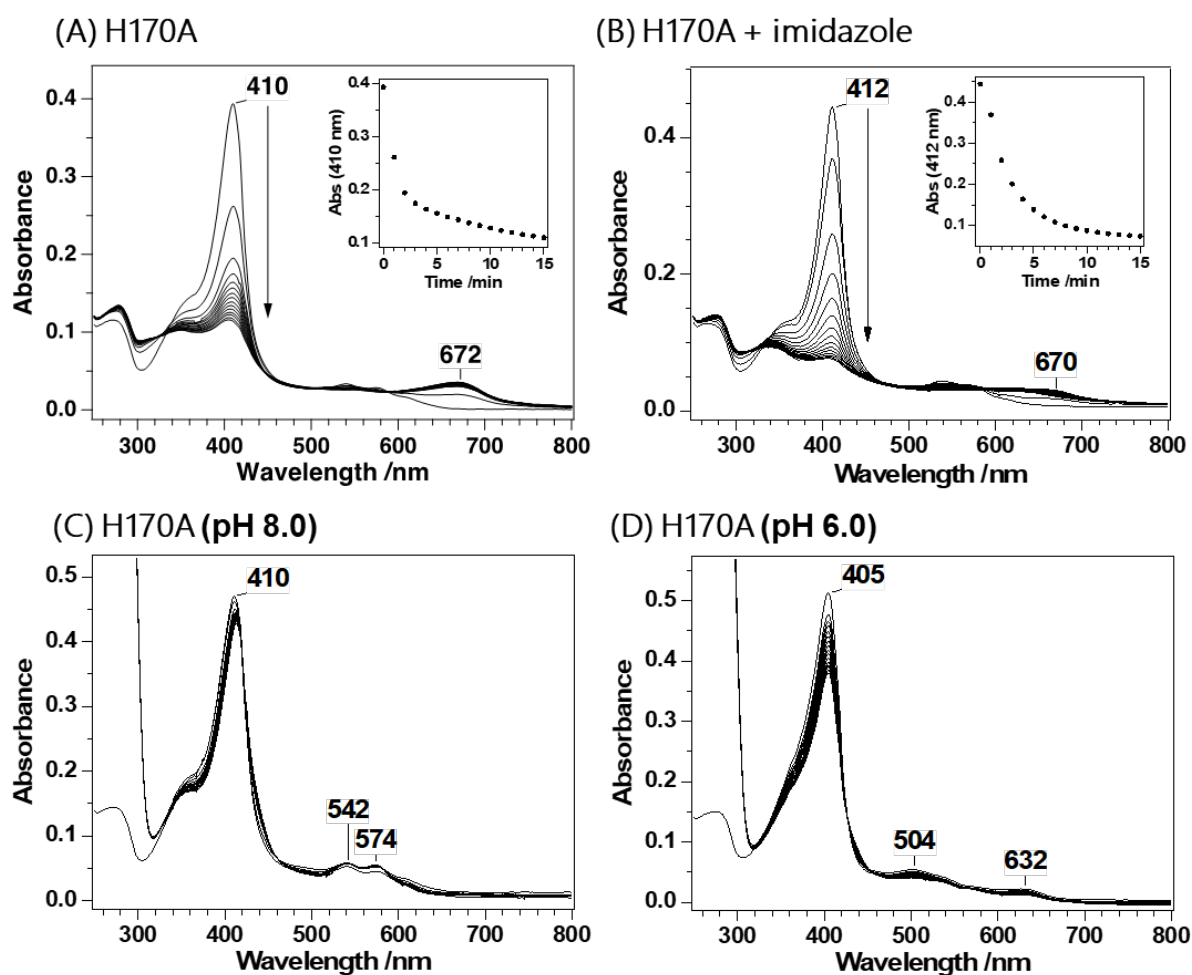
Fig. 11. Heme degradation reaction of the H170A mutant. Reaction with 0.2 mM H 2 O 2 at pH 8.0 in the (A) absence and (B) presence of 2000 equivalents of imidazole. Reaction with mM ascorbic acid at (C) pH 8.0 and (D) pH 6.0.
