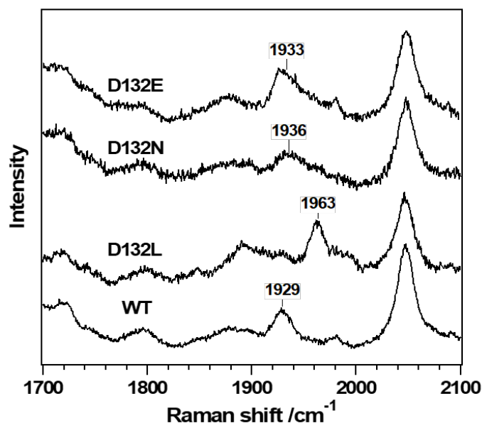
Fig. 8. Resonance Raman spectra of the heme-Asp132 mutants and heme-WT HutZ in the CO-bound form.
