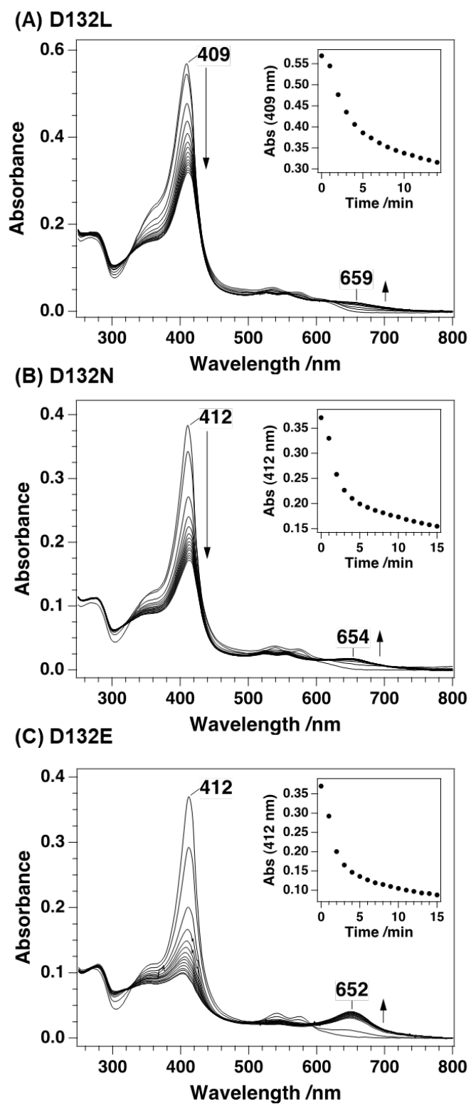
Fig. 3. Heme degradation reaction of the heme-HutZ complex with \text{H}_2\text{O}_2 (0.2 mM) at pH 8.0. Spectra were measured before addition of \text{H}_2\text{O}_2 , and at 1-min intervals for 15 min after addition of \text{H}_2\text{O}_2 . Inset: Time course of absorbance at the Soret maximum. (A) Heme-D132L; (B) heme-D132N; and (C) heme-D132E.
