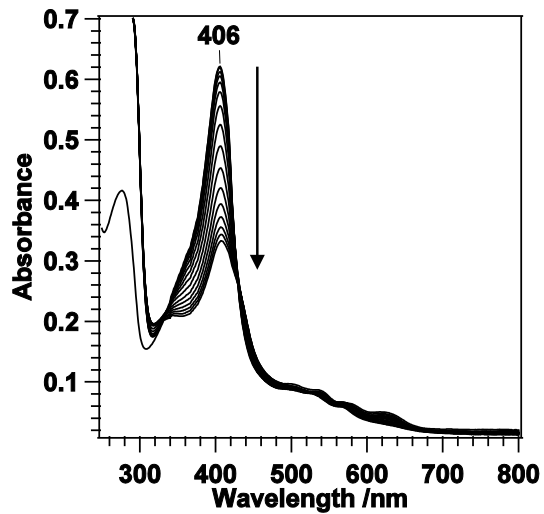
Fig. 2 Heme-degradation reaction of the heme-HutZ complex with ascorbic acid (1.0 mM) at pH 6.0. Spectra were measured before addition of ascorbic acid, and at 2-min intervals for 30 min after addition of ascorbic acid in the presence of (A) 0.10 mM DFO, (B) 1.0 mM citric acid, and (C) 0.10 mM EDTA.
