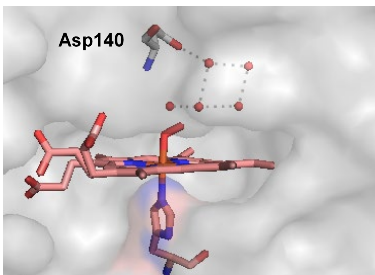
Fig. 10 Crystal structure of HO-1 from rat in the O 2 -bound form (PDB ID code 4G7L).
