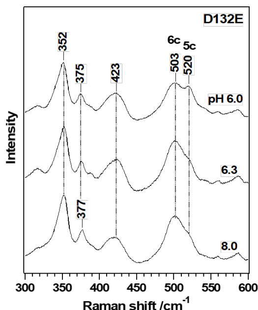
Fig. 13. Resonance Raman spectra of the heme-D132E mutant in the CO-bound form.
