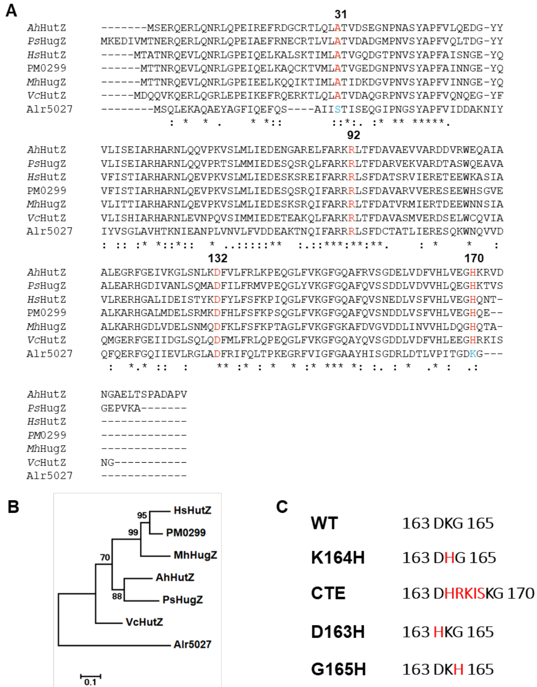
Fig. 1. Sequence alignment of Alr5027. (A) Sequence alignment of the HutZ family and Alr5027. The alignment was performed using ClustalW2 ( http://www.ebi.ac.uk/Tools/msa/clustalw2/ ). The active site arginine, aspartate, and histidine are shown in red bold type. Proteins used in the alignment are (from top to bottom) Aeromonas hydrophila subsp. hydrophila ATCC 7966 HutZ, Plesiomonas shigelloides HugZ, Histophilus somni HutZ, multocida str. Pm70 PM0299, Mannheimia haemolytica PHL213 HugZ, Vibrio cholerae HutZ, and Nostoc sp. PCC 7120 Alr5027. (B) Phylogenetic tree of Alr5027 with the HutZ family. The tree was obtained from the sequence alignment in Fig. 1A. The maximum likelihood method was used for tree construction and bootstrap analysis (parameter set at 1000 resampling), performed using MEGA 7 software. (C) Alignment of Alr5027 WT and mutants in the C-terminal region (163–165).
