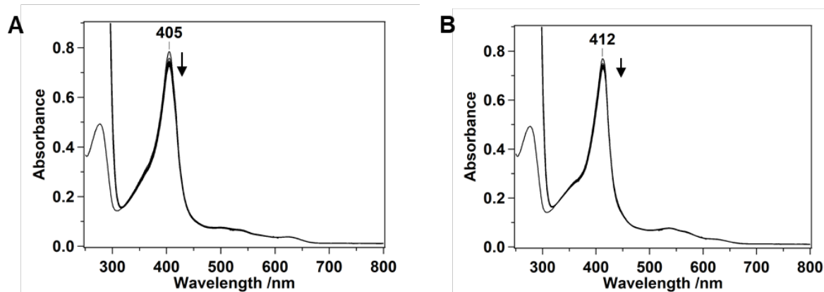
Fig. 11. Absorption spectrum of the heme-ERKT mutant. Heme-degradation reaction of the heme-Alr5027 ERKT mutant with ascorbic acid at pH 6.0 (A) and pH 8.0 (B). Spectra were monitored before the addition of ascorbic acid, and at 2-min intervals for 30 min after the addition of ascorbic acid.
