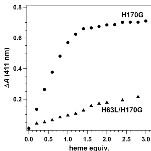
Fig. 10. Heme titration plot of the H63L/H170G double mutant.
