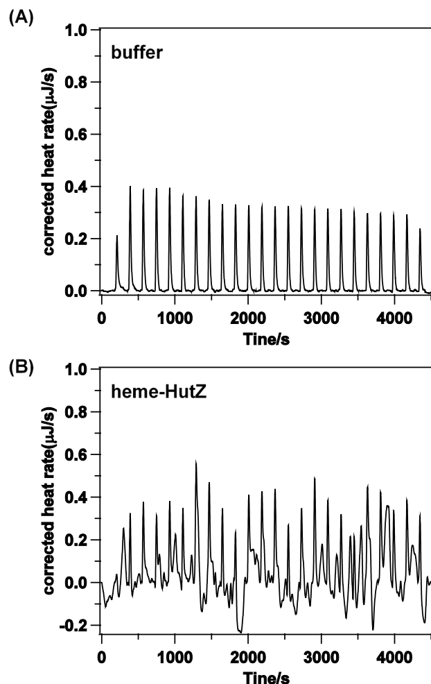
Fig. 5 ITC data for titration of 3 \mu\text{M} DFO into (A) buffer, and (B) 35 \mu\text{M} heme-HutZ. Injections ( 25 \times 2 \mu\text{L} ) were made at 180 sec intervals in 50 mM Tris-HCl/150 mM NaCl (pH 8.0) at 25 ^{\circ}\text{C} .
