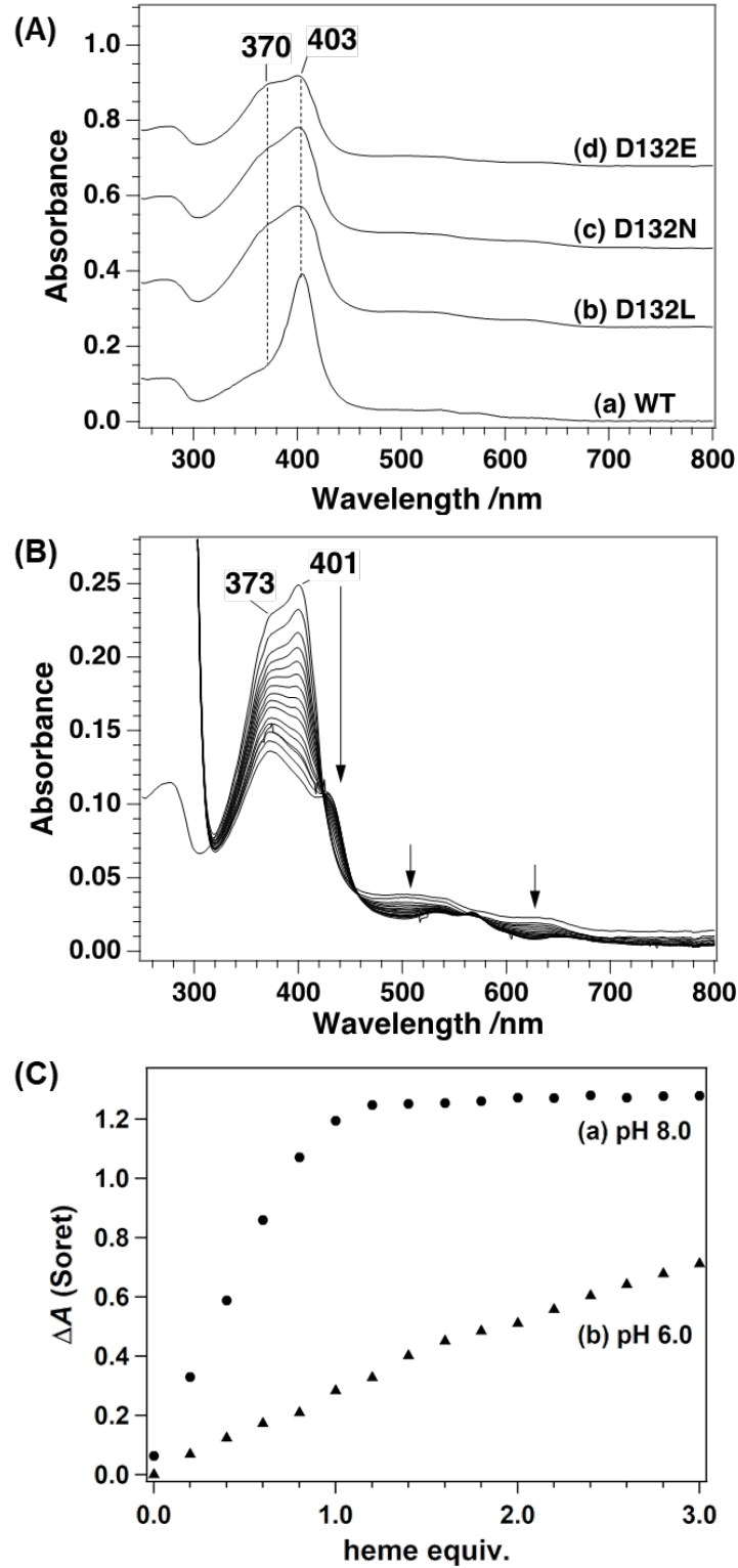
Fig. 6. (A) Absorption spectra of heme-Asp132 mutants and heme-WT HutZ at pH 6.0. (B) Heme degradation reaction of the heme-D132E mutant with ascorbic acid (1.0 mM) at pH 6.0. Spectra were measured before addition of ascorbic acid, and at 2-min intervals for 30 min after addition of ascorbic acid. (C) Heme-binding curve generated from difference absorbance spectra by plotting \Delta A versus the molar ratios of heme to D132E mutant at pH 8.0 (a) and pH 6.0 (b)
