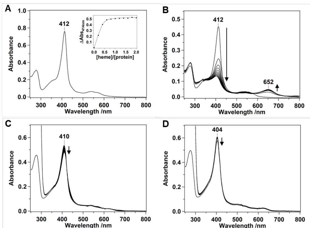
Fig. 9. Absorption spectrum of the heme-CTE mutant. (A) Absorption spectrum of the heme-CTE mutant. The inset shows differences at 414 nm. (B) Heme-degradation reaction of the CTE mutant with \text{H}_2\text{O}_2 (0.1 mM) at pH 8.0. The reaction conditions in (A) and (B) were same as those in Fig. 6A and C, respectively. (C, D) Heme-degradation reaction of the CTE mutant with 1.0 mM ascorbic acid at pH 8.0 (C) and pH 6.0 (D). Spectra were recorded before addition of ascorbic acid, and at 2-min intervals for 30 min after addition of ascorbic acid.
