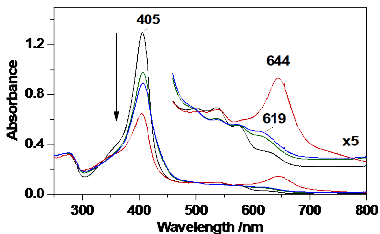
Fig. 3 Reaction of ferric heme-HutZ (10 μM) with 1 equivalent of H 2 O 2 at pH 6.0. Black, before the reaction; green and blue, 20 sec and 5 min after the reaction, respectively; red, 15 min after addition of air to the blue species. Reaction was conducted under an anaerobic condition.
