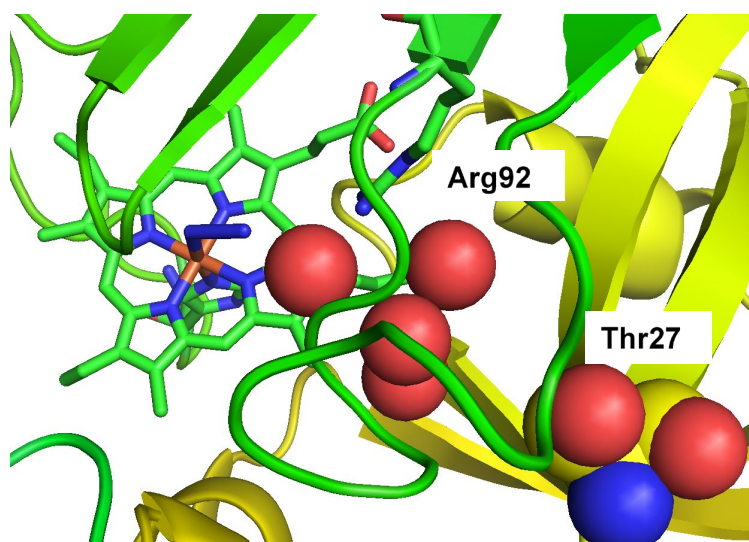
Fig. 12 Crystal structure of HugZ from Helicobacter pylori (PDB ID code 3GAS).
