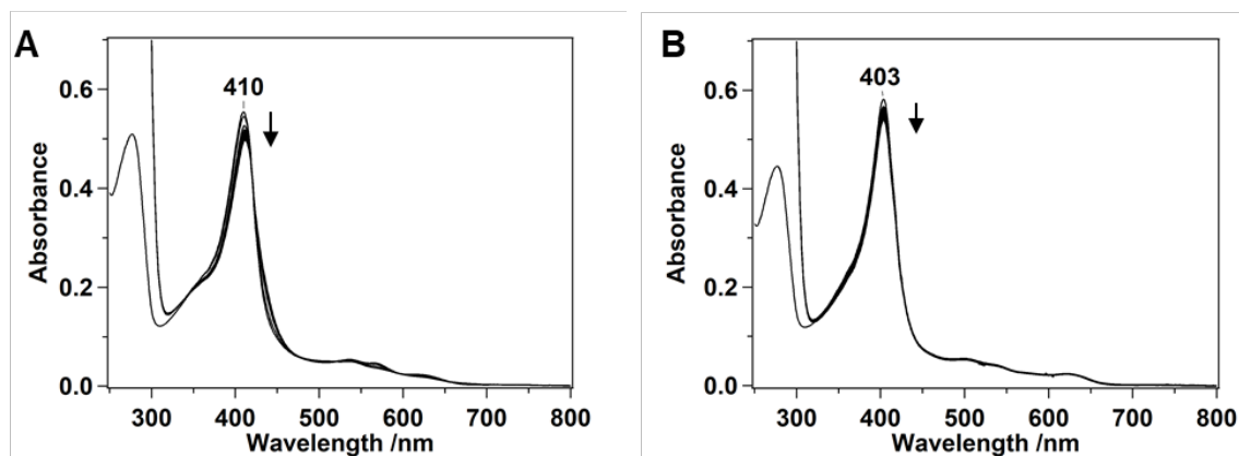
Fig. 7. Heme-degradation reaction of the K164H mutant with ascorbic acid. (A) pH 8.0 and (B) pH 6.0. Spectra were recorded before the addition of ascorbic acid, and at 2-min intervals for 30 min after the addition of ascorbic acid. The concentrations of the protein and ascorbic acid were 5 \mu M and 1.0 mM, respectively.
