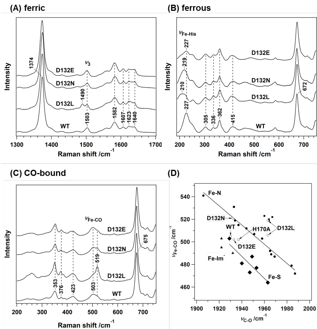
Fig. 7. Resonance Raman spectra of the heme-HutZ complex. The protein concentration was 10 \mu\text{M} in 50 mM Tris-HCl/150 mM NaCl, pH 8.0. The excitation wavelength for ferric and CO-bound forms was 413.1 nm, and that for the ferrous form was 441.6 nm. (A) Ferric form in the high-frequency region; (B) ferrous form in the low-frequency region; (C) CO-bound form in the low-frequency region; and (D) correlation plot of frequency of \nu_{\text{Fe-CO}} versus \nu_{\text{C-O}} . The two solid lines correspond to correlations for proximal imidazoles (solid black circles), proximal imidazolate (solid green triangles), and thiolate-ligated hemoproteins (solid diamonds). Data points for oxidase superfamily members are depicted as solid squares. The data point for heme-HutZ is presented as an open circle in red. The data shown in the \nu_{\text{Fe-CO}} versus \nu_{\text{C-O}} inverse correlation plot are taken from references 23-25 .
