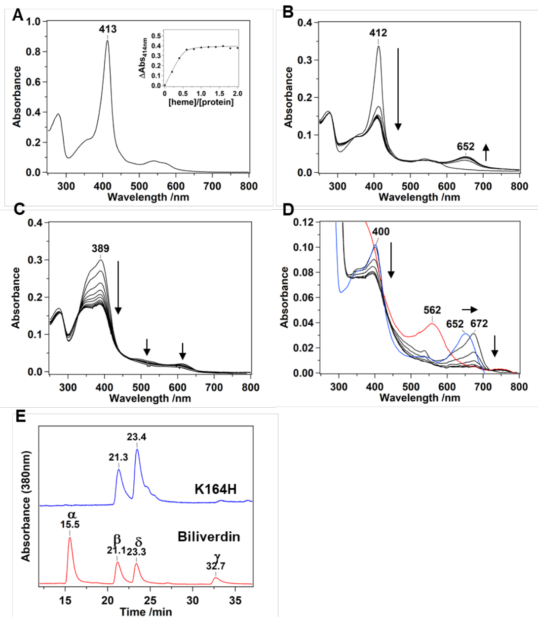
Fig. 4. Absorption spectra and chromatogram of the heme-K164H mutant. (A) Absorption spectra of the heme-K164H mutant at pH 8.0. The inset shows differences at 414 nm following incremental addition of heme (2–30 \mu\text{M} ) to the mutant (10 \mu\text{M} ) in 50 mM Tris-HCl and 150 mM NaCl (pH 8.0), measured against a blank cell containing buffer alone. (B, C) Heme-degradation reaction of the heme-K164H mutant (B) and heme-WT Alr5027 (C) reacted with 0.1 mM \text{H}_2\text{O}_2 at pH 8.0. Spectra were obtained before and after the addition of \text{H}_2\text{O} at 1-min intervals over 10 min. (D) Reaction of the verdoheme-K164H mutant with 1 mM ascorbic acid at pH 8.0. Absorption spectra in the reaction with ascorbic acid after the formation of verdoheme (blue line) by addition of 0.1 mM \text{H}_2\text{O}_2 . Spectra were recorded before and after the addition of ascorbic acid at 4, 8, 16, 24, and 32 min (black line). Ferrozine (0.10 mM) was added 32 min after the reaction (green line). (E) HPLC chromatograms of biliverdin standard (red line) and final products of the heme-K164H mutant (blue line) monitored at 380 nm.
