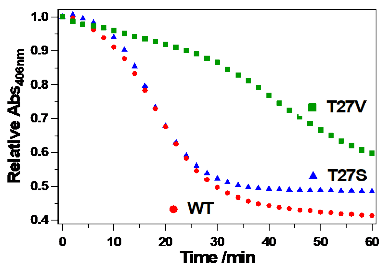
Fig. 13 Changes in absorbance intensity at 406 nm in reactions of heme-HutZ WT, and heme-HutZ T27V and T27S mutants with ascorbic acid (1 mM).
