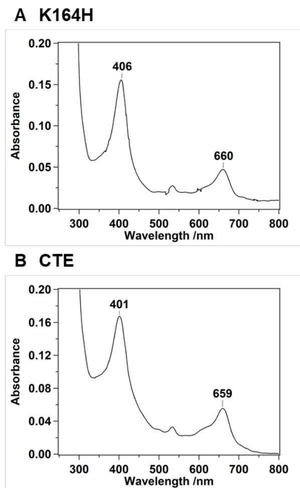
Fig. 6. Absorption spectra of verdoheme in aqueous pyridine. (A) K164H and (B) CTE heme-bound mutants were reacted with \text{H}_2\text{O}_2 under the same conditions at those in Fig. 5. Pyridine (final concentration, 33%) was added to the reaction mixture 10 min after the reaction to liberate the product from the protein.
