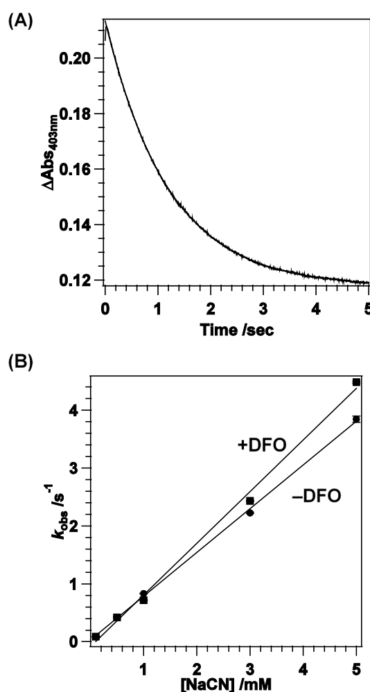
Fig. 8 Cyanide binding to heme-HutZ. (A) typical time trace of the absorbance change at 403 nm upon mixing 3.0\text{ }\mu\text{M} of heme-HutZ with 1.0\text{ mM} \text{CN}^- in 50\text{ mM} MES-NaOH/ 150\text{ mM} NaCl (pH 6.0). (B) Plots of k_{\text{obs}} versus \text{CN}^- concentrations.
