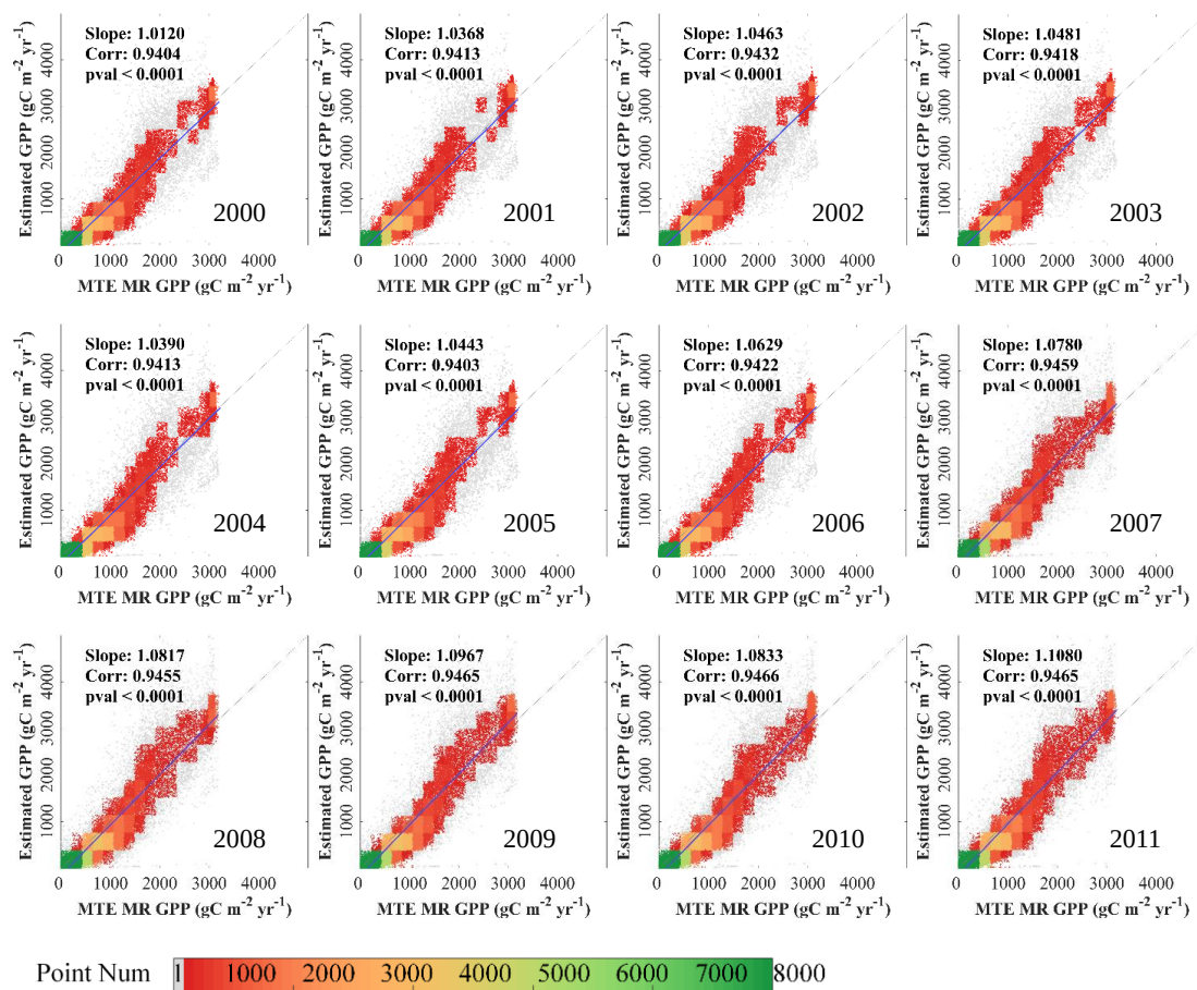
Figure S12 Comparisons of annual GPP estimated by the MTE-MR and the iBEPs model.
