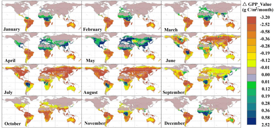
Figure 4.22 Comparison of monthly GPP estimates using different CO 2 data forms ( \text{GPP}_{2014}^{\text{monthly spatial CO}_2} minus \text{GPP}_{2014}^{\text{annual mean global CO}_2} ).
