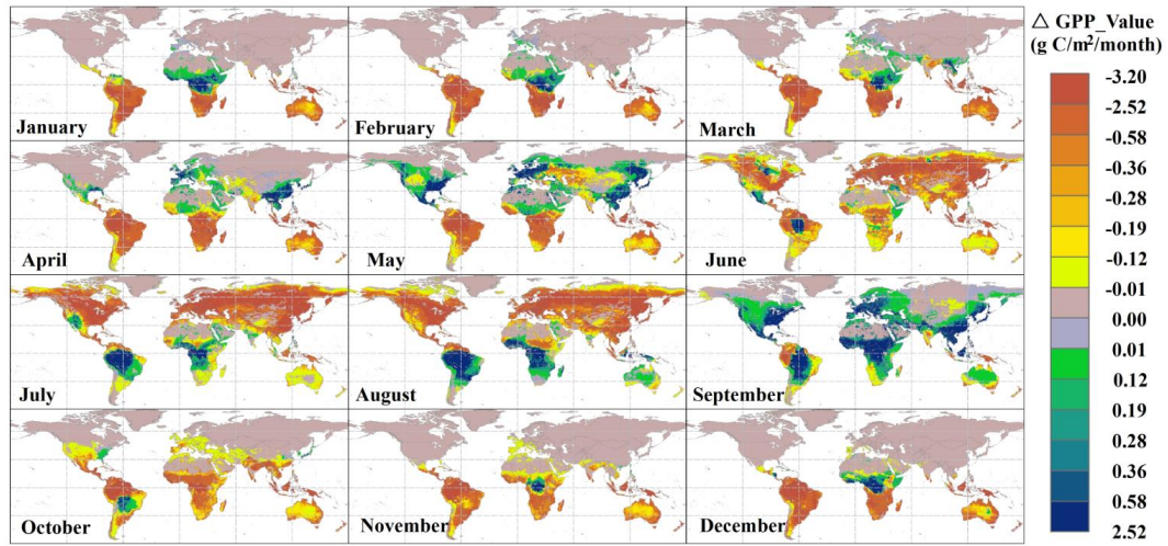
Figure 4.23 Comparison of monthly GPP estimates using different CO 2 data forms ( \text{GPP}_{2014}^{\text{monthly spatial CO}_2} minus \text{GPP}_{2014}^{\text{monthly mean global CO}_2} ).
