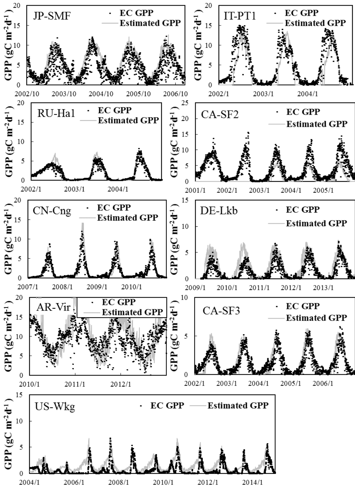
Figure S15-c Comparisons of flux GPP and the iBEPs estimated GPP of each site.
