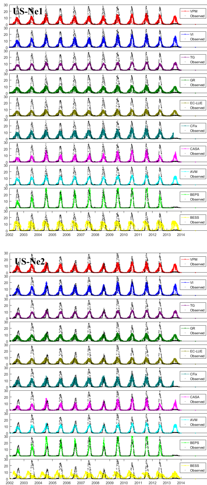
Figure S1-1 Comparisons of flux GPP and estimated GPP of each site.
