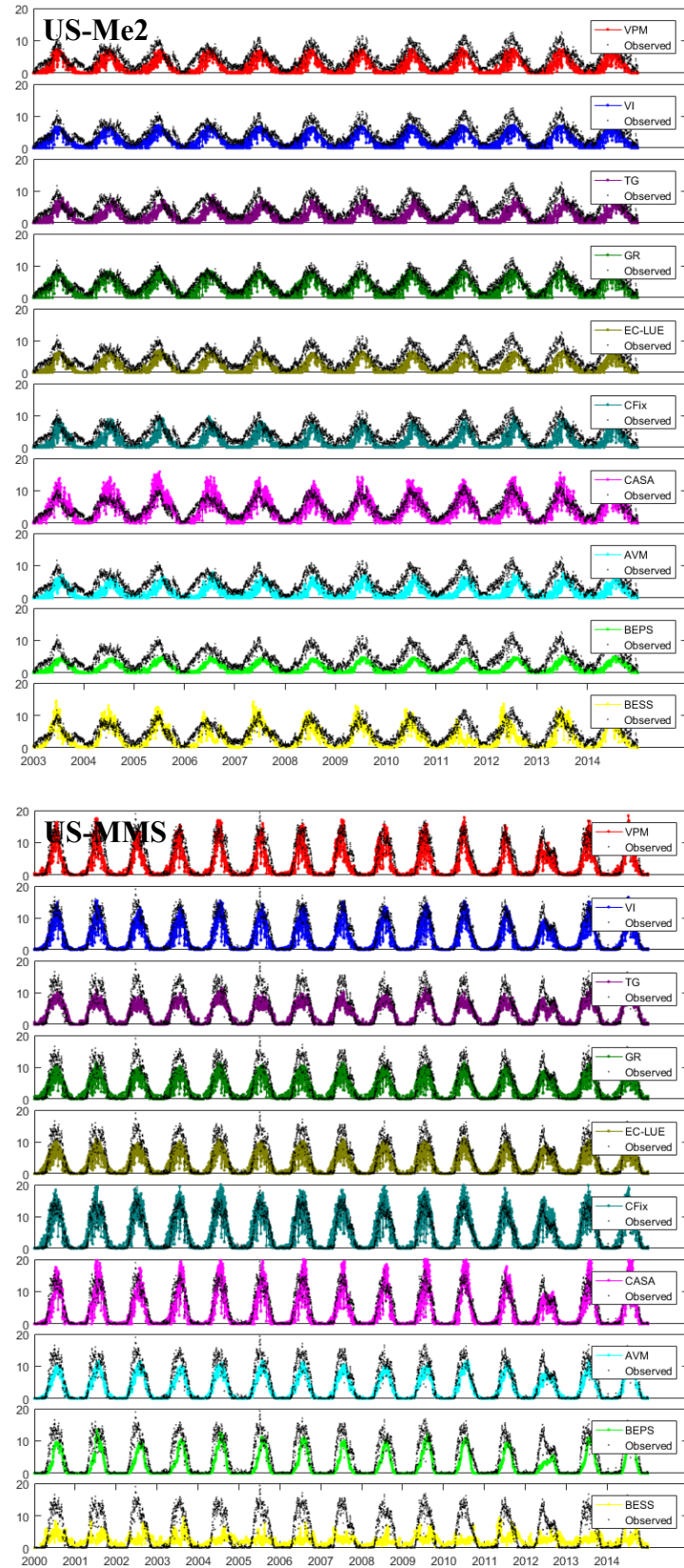
Figure S1-k Comparisons of flux GPP and estimated GPP of each site.
