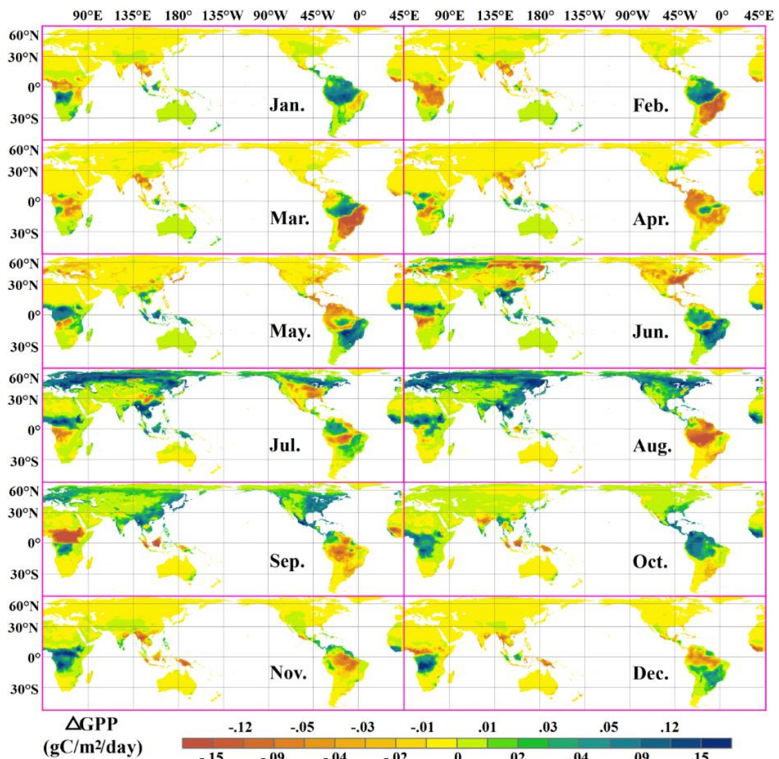
Figure 4.13 Comparison of the monthly GPP estimates using different CO 2 data forms (GPP ann CO 2 minus GPP spa CO 2 ).
