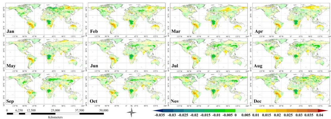
Figure S4 The monthly spatial distributions of linear trends in water conditions during the period 1982-2015.
