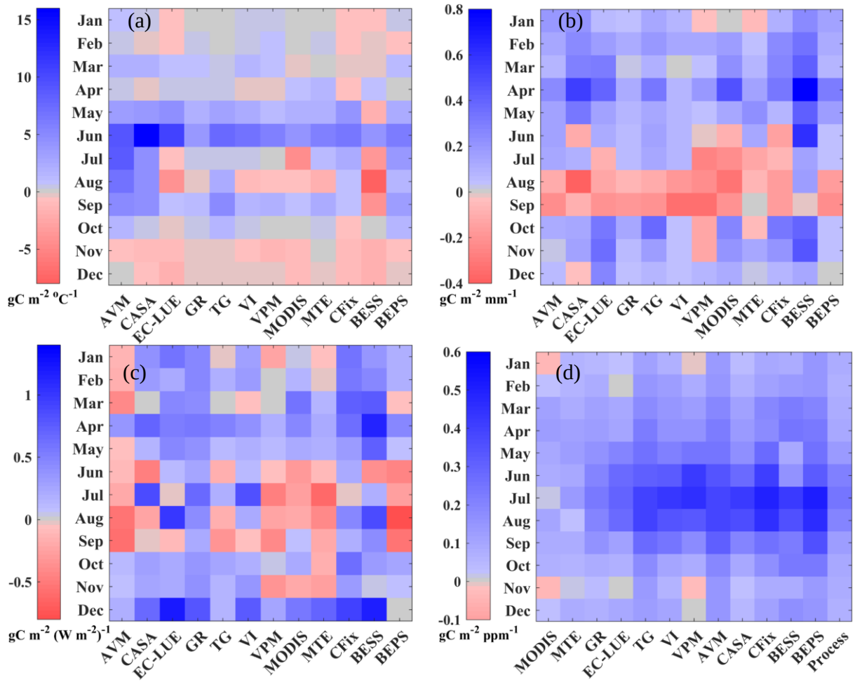
Figure 5.5 The monthly responses of GPP to variations in climate of each model, (a) to temperature change, (b) to precipitation change, (c) to radiation change and (d) to rising atmospheric CO 2 concentration.
