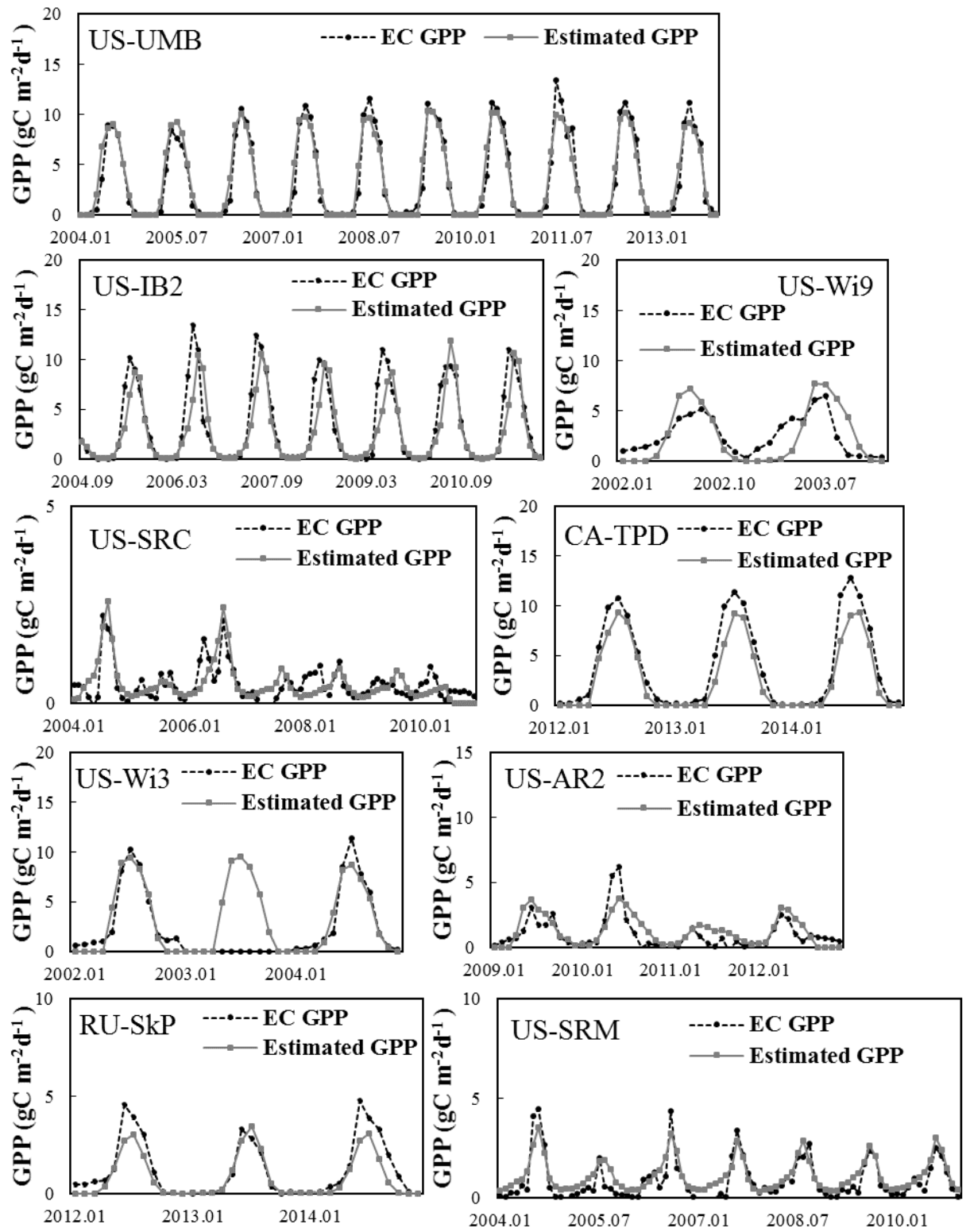
Figure S15-h Comparisons of flux GPP and the iBEPs estimated GPP of each site.
