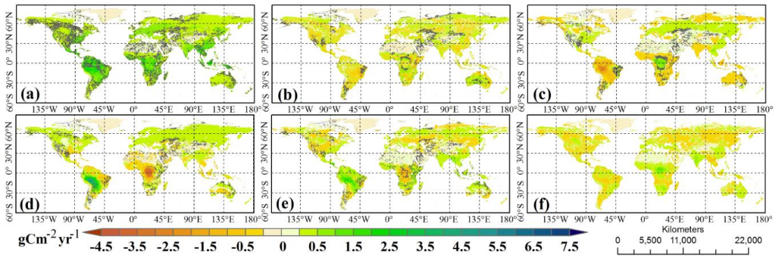
Figure 3.4 Spatial distribution of the trends in GPP due to (a) increases in atmospheric \text{CO}_2 concentration, (b) land-cover change, (c) solar radiation changes, (d) temperature changes, (e) changes in water conditions, and (f) their nonlinear interactions or non-attributed. The pixels ((a) to (e)) that are not satisfied at p\_value < 0.1 are drawn in gray.
