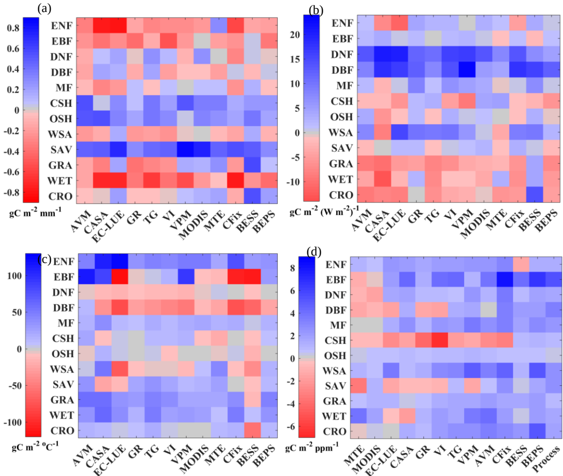
Figure 5.6 The responses of GPP to the variations in (a) precipitation, (b) radiation, (c) temperature and (d) rising \text{CO}_2 concentration across PFTs by each model.
