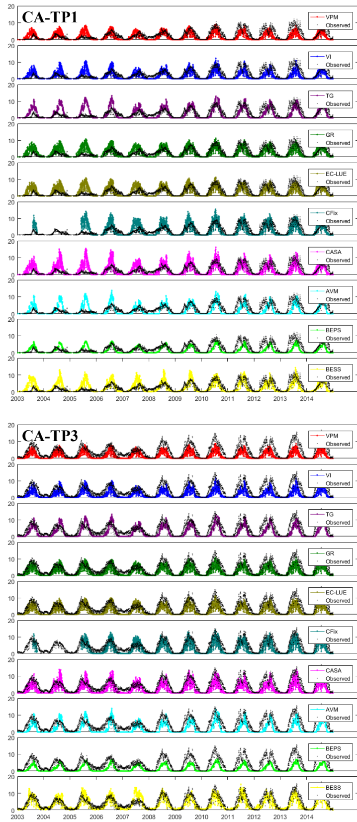
Figure S1-c Comparisons of flux GPP and estimated GPP of each site.
