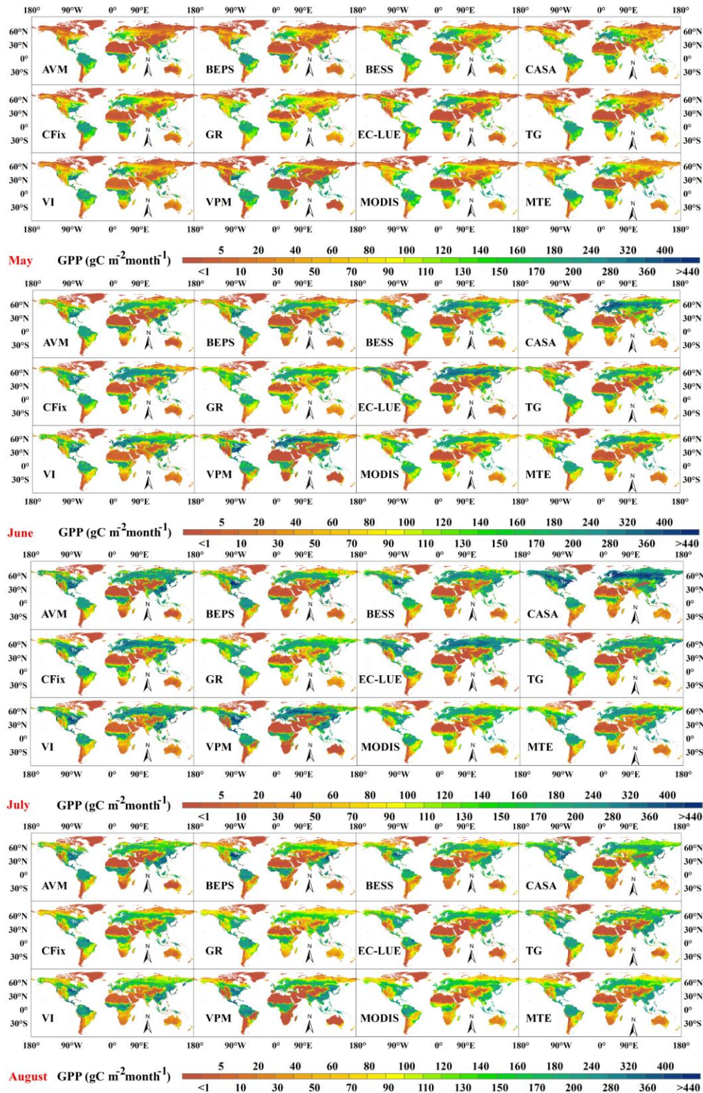
Figure 2.7-b Monthly global GPP estimation by each model.
