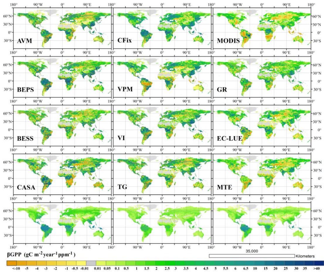
Figure 5.4 Global distribution of responses of GPP to rising atmospheric CO 2 concentration.
