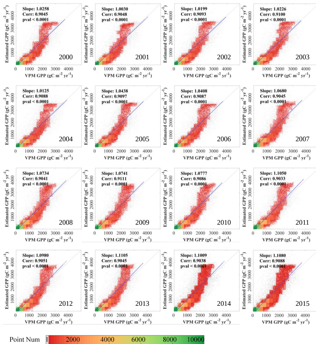
Figure S10 Comparisons of annual GPP estimated by the VPM algorithm and the iBEPs model.
