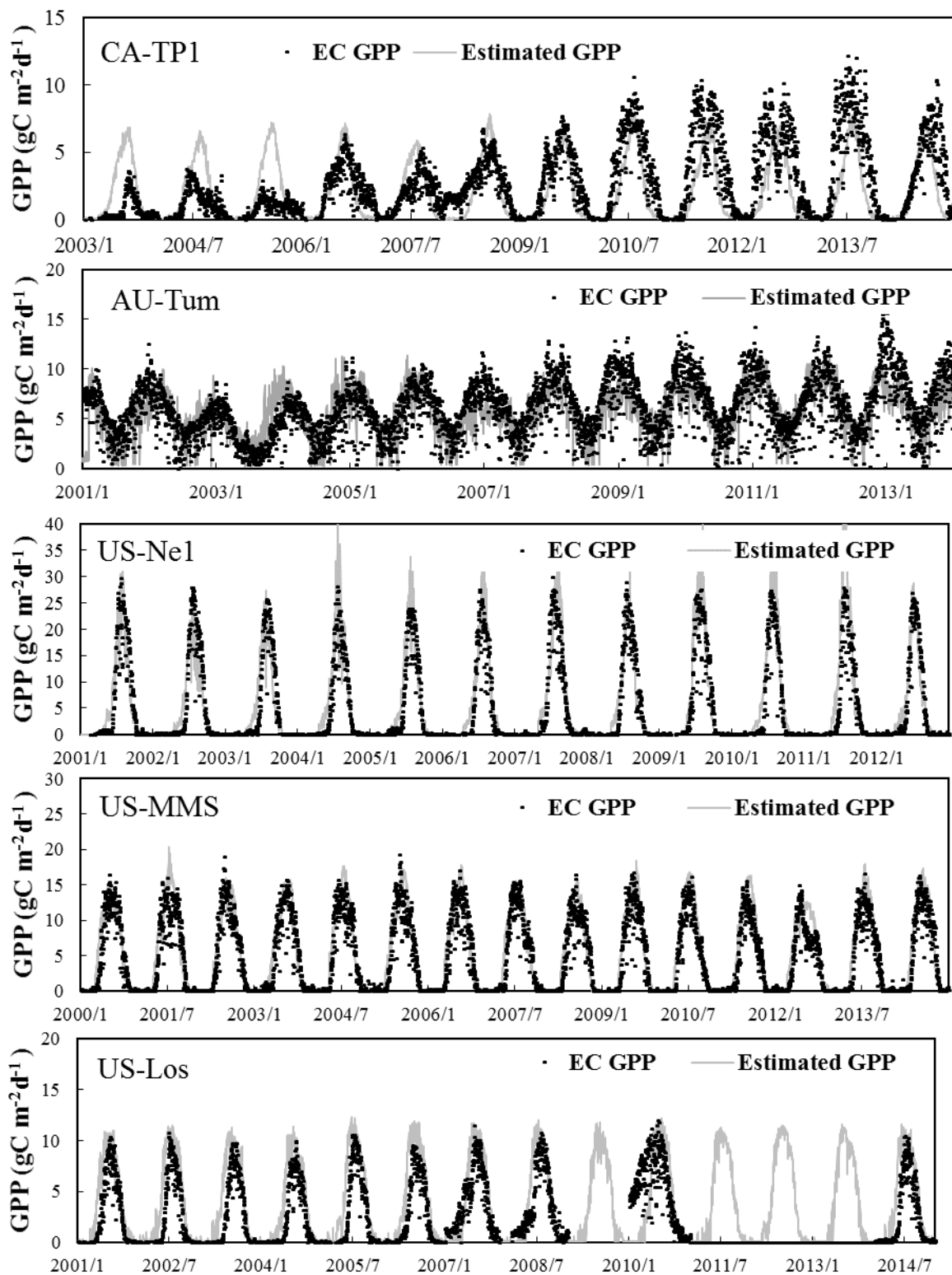
Figure S15-a Comparisons of flux GPP and the iBEPs estimated GPP of each site.
