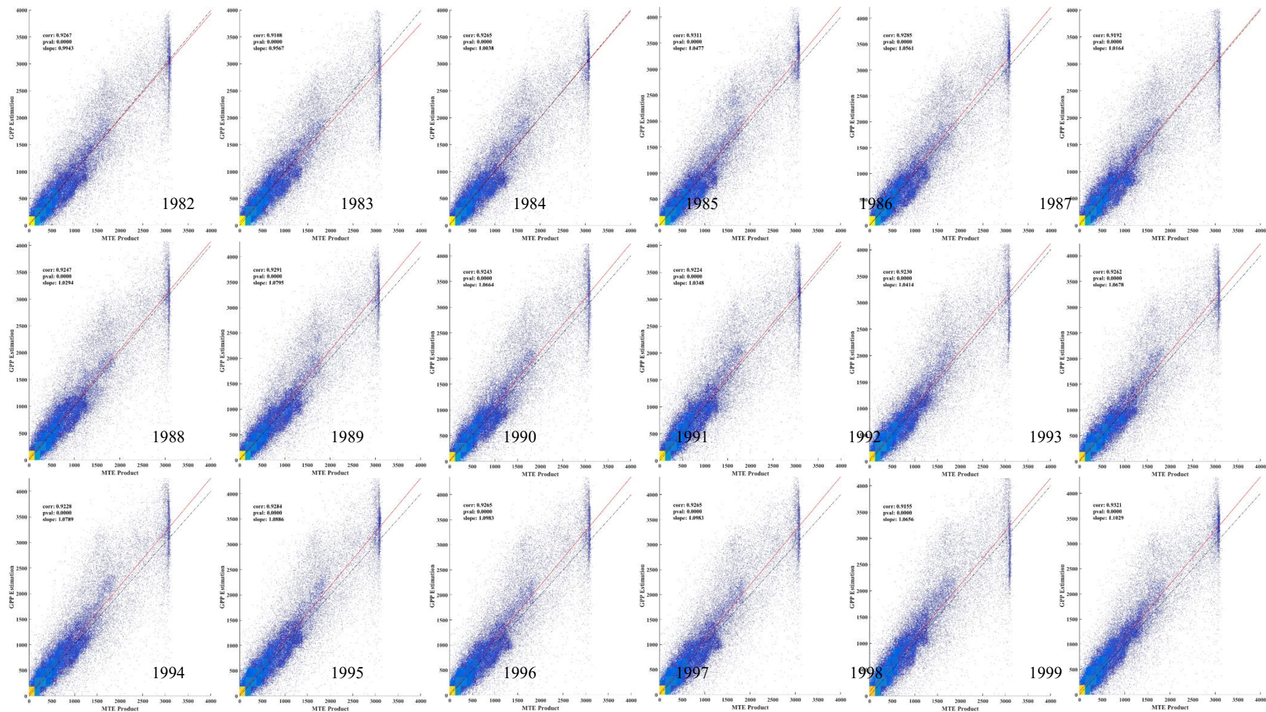
Figure S7-a Scatter plots of estimated GPP values (y axis) vs. MTE_MR GPP values (x axis) from 1982 to 2011. Only pixels over vegetated areas are shown. The parameters of the linear regression line in all panels are shown in Table 3.3.
