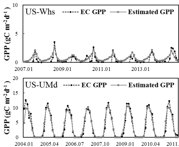
Figure S15-i Comparisons of flux GPP and the iBEPSd estimated GPP of each site.
