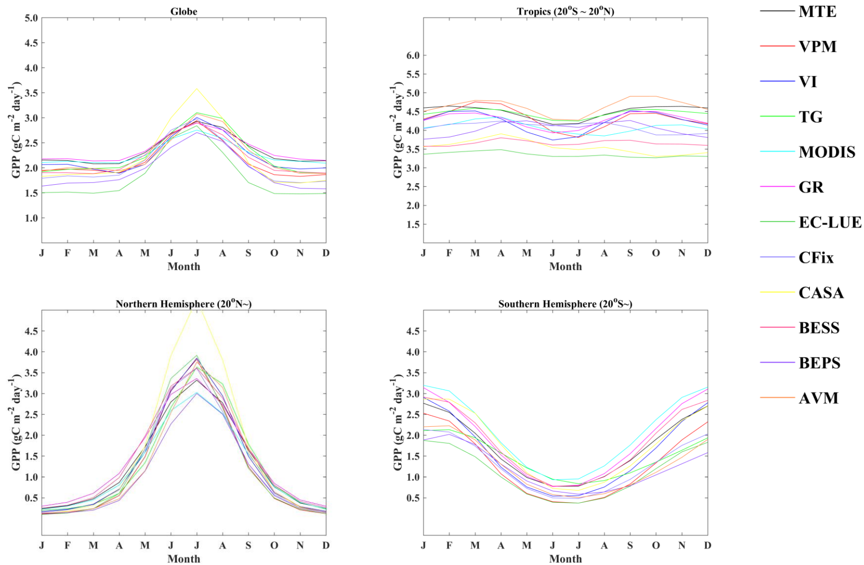
Figure 2.8 Comparison of seasonal variations in GPP among the different models.
