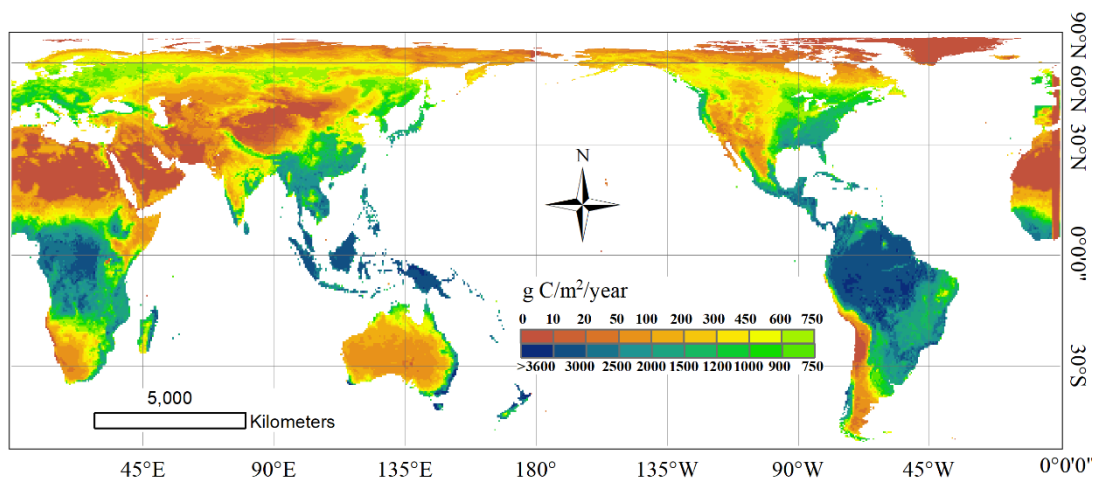
Figure 4.3. Global spatial distribution of the annual mean GPP for 2000-2015.
