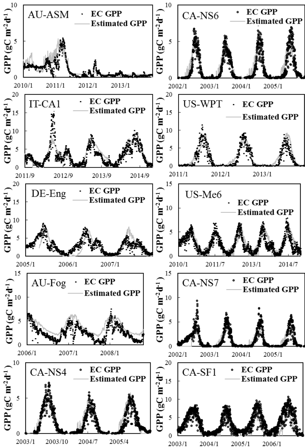
Figure S15-e Comparisons of flux GPP and the iBEPs estimated GPP of each site.
