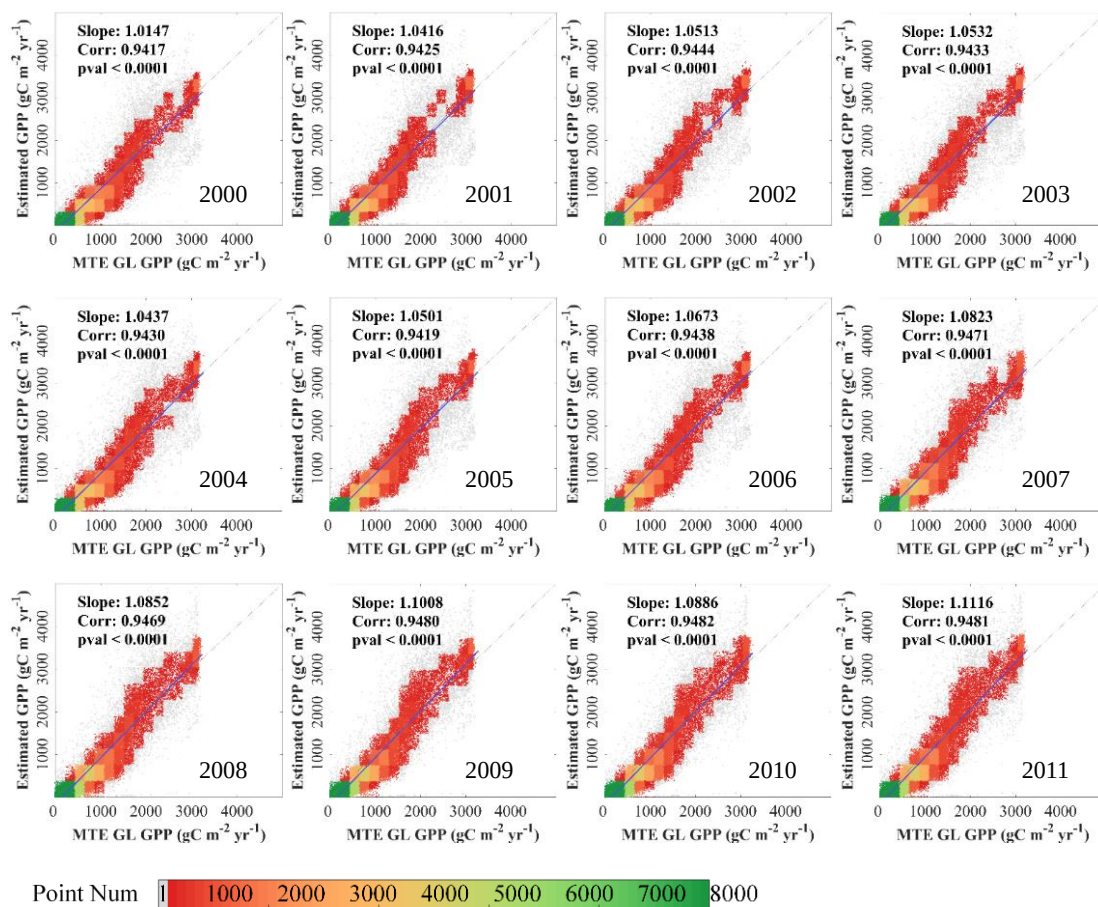
Figure S11 Comparisons of annual GPP estimated by the MTE-GL and the iBEPs model.
