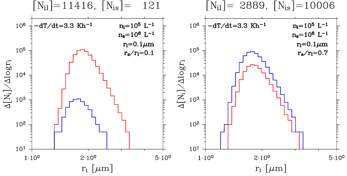
Figure 4.10: Same as Fig. 4.9, but for the cases of n_s = 10^6 \text{ L}^{-1} and r_s/r_l = 0.1 (left panel) and 0.7 (right panel).
