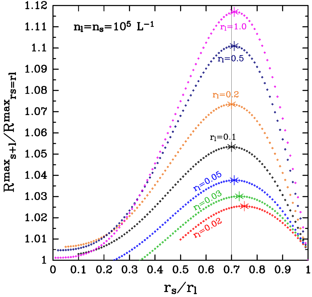
Figure 4.5: Same as Fig. 4.4, but redrawn by normalizing the vertical axis by the maximum ice nucleation ratio when r_s = r_l ( R_{rs=r_l}^{\max} ).
