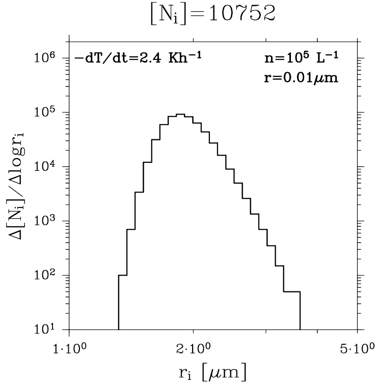
Figure 3.2: The size distribution of ice particles at the moment when the supersaturation is dissolved, obtained from the simulation shown in Fig. 3.1.
