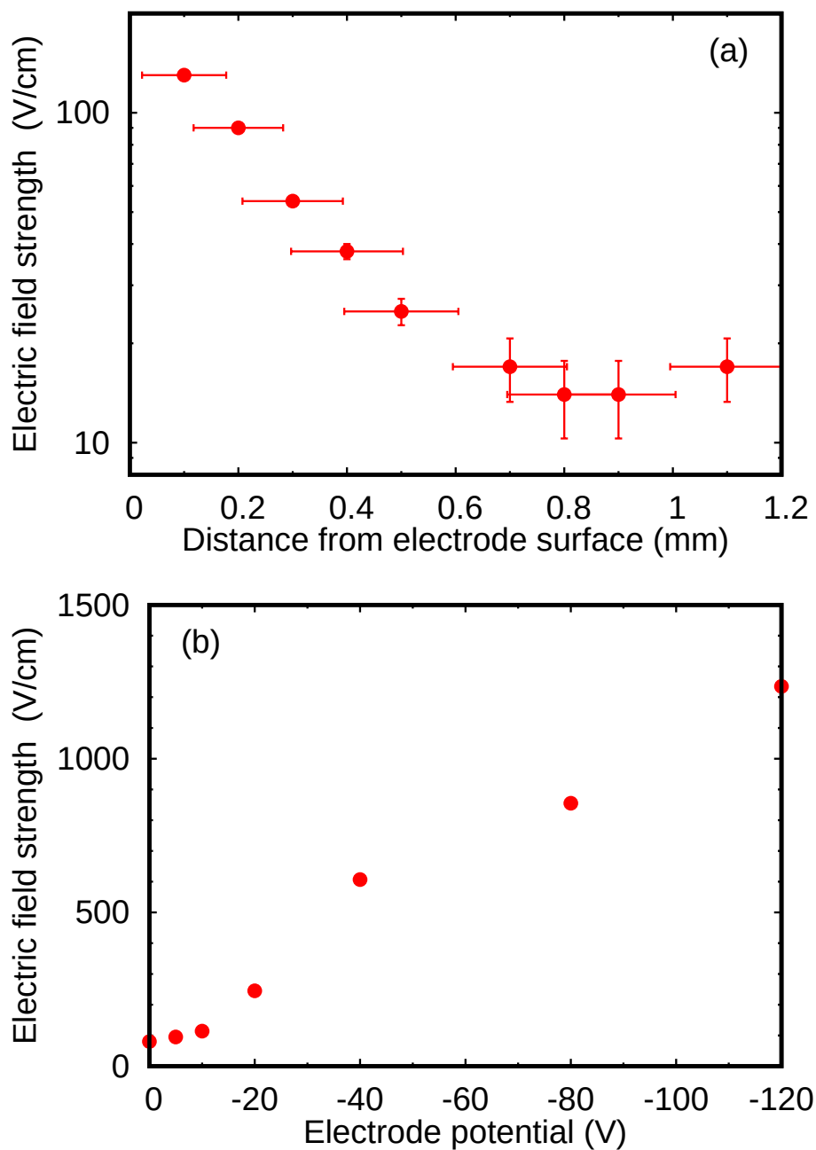
Figure 8. Electric field strength evaluated by the developed method. (a) shows the electric field as a function of the distance from the surface of the grounded electrode. (b) shows the electric field at a distance of 0.4 mm from the electrode as a function of the applied voltage.
