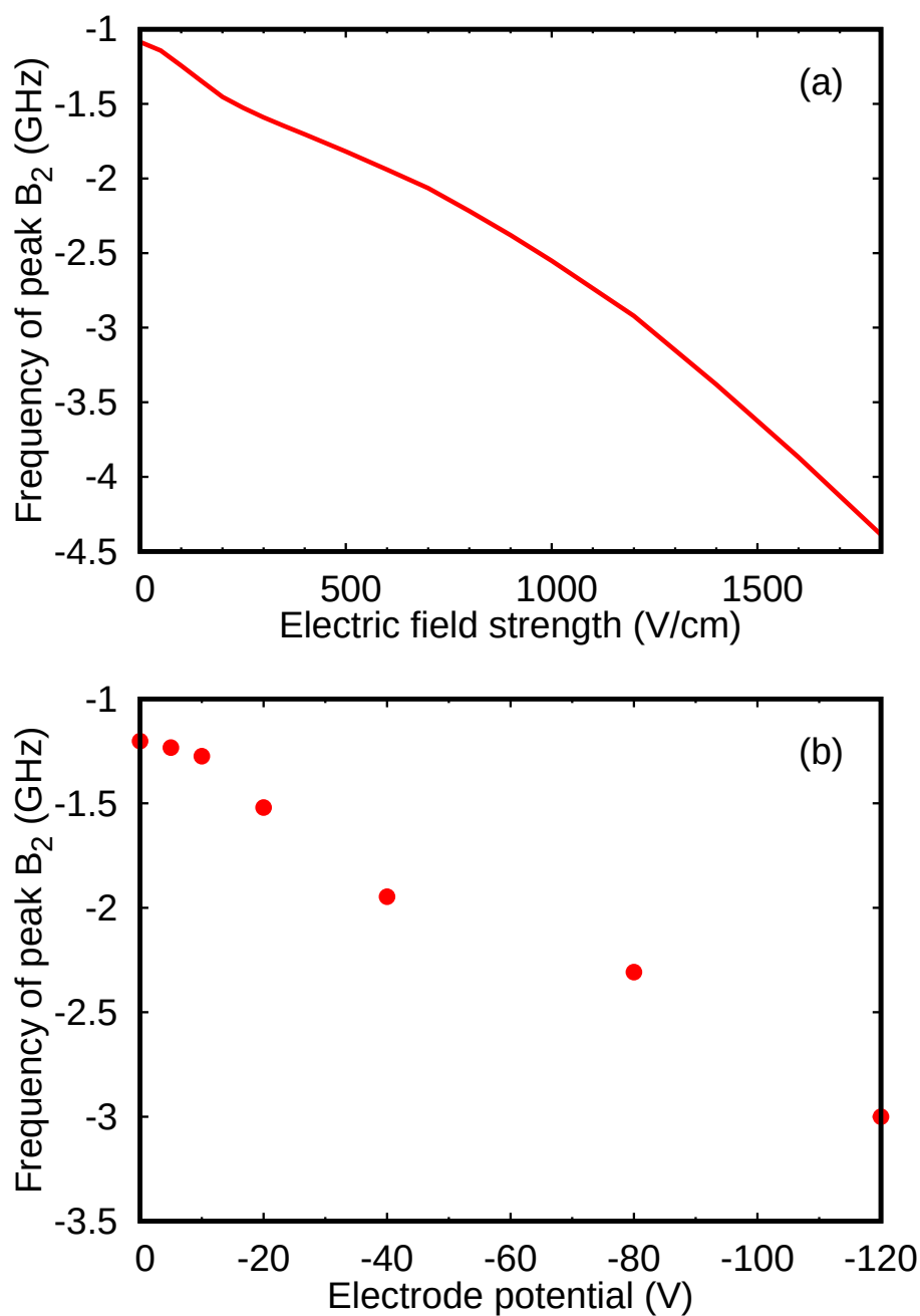
Figure 6. Frequency of the 2p^2P_{3/2}^{\circ} - 3d^2D_{3/2} transition (peak B (or B_2 )) in the \pi polarization configuration. (a) is the theoretical result as a function of the electric field. (b) is the experimental result observed at a distance of 0.4 mm from the electrode as a function of the applied voltage.
