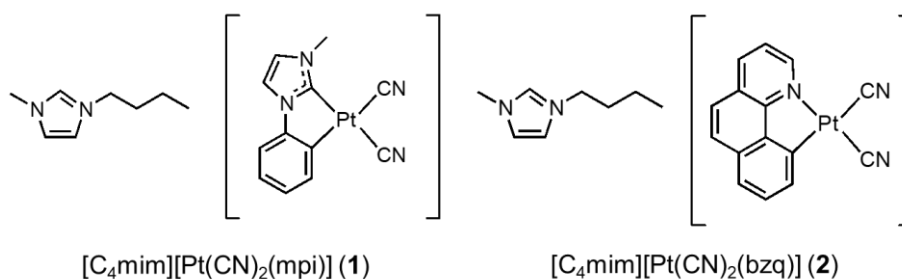
Scheme 1. Structural formula of Pt(II) complexes 1 and 2 .
