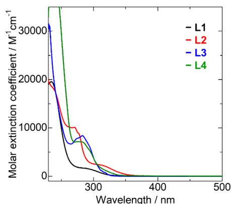
Figure 7. UV-vis absorption spectra of the ligands in \text{CH}_2\text{Cl}_2 (concentration = 1.0 \times 10^{-5} M) at room temperature: L1 = 1-methyl-3-phenyl-1 H -benzimidazolium (black line), L2 = 1-methyl-3-phenyl-1 H -benzimidazolium (red line), L3 = 1-methyl-3-(naphtharene-2-yl)-1 H -imidazolium (blue line), and L4
