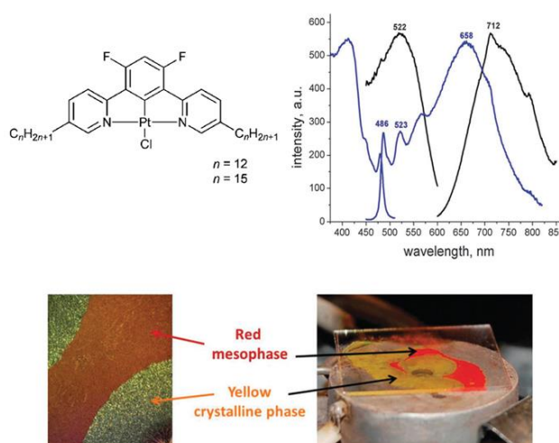
Figure 8. Structural formula of [Pt(Rdpb)Cl] and their photophysical properties. 30
