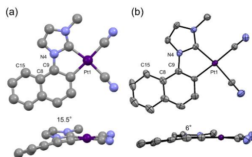
Figure 20. Atom numbers and torsion angles of (a) calculated optimized structure of excited triplet state and (b) crystal structure of 4 .
