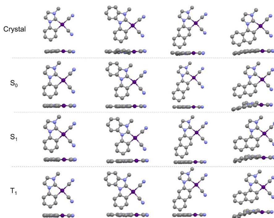
Figure 19. Crystal, ground state (S 0 ), excited singlet state (S 1 ), excited triplet state (T 1 ) optimized structure of complexes 1–4 viewed from top and side. The hydrogen atoms were omitted for clarity. The atom color represents Pt (purple), C (gray), and N (blue), respectively
