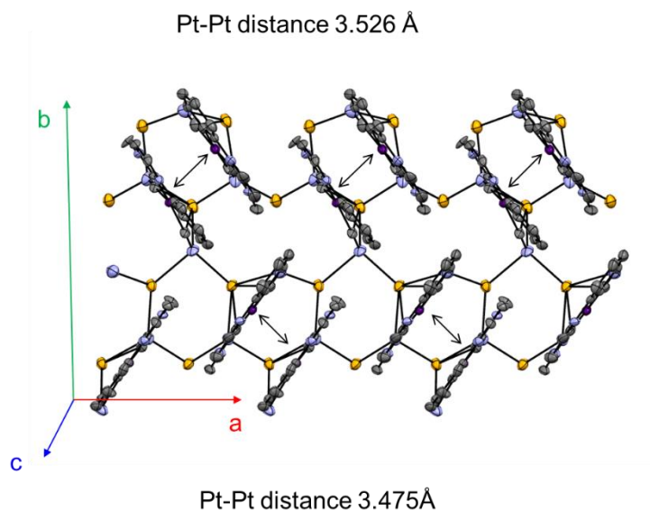
Figure 5. ORTEP drawings showing the dimer structure of potassium salt ( 3 ). Displacement parameters are drawn at the 50% probability level. Hydrogen atoms are omitted for clarity. Color code: Pt, purple; C, grey; N, blue; K, orange.
