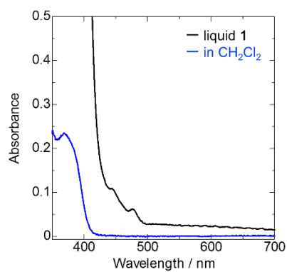
Figure 10. Absorption spectra of neat liquid 1 (black line) and 1 in \text{CH}_2\text{Cl}_2 (blue line, 1.0 \times 10^{-4} M)
