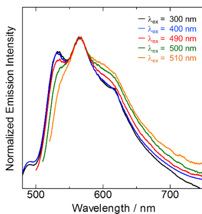
Figure 8. Excitation wavelength dependency for emission spectra of 1 . Thin liquid membrane condition of neat 1 sandwiched in two quartz plates were measured under \text{N}_2 atmosphere at 298 K.
