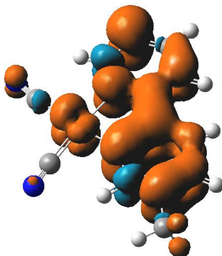
Figure 9. Spin density of monomer 4 ( [\text{Pt}(\text{CN})_2(\text{pty})]^- ) of the S=1 state mainly delocalized on the pty ligand, suggesting that the two-unpaired electron are on the pty ligand. Therefore, S=1 state can be assigned to ^3\text{LC} .
