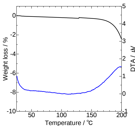
Figure 2. Thermogravimetry-differential thermal analyses of 1 at scan rate of 5 K min -1 (TG (black), DTA (blue)).
