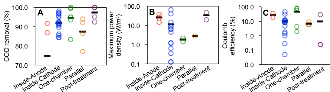
Fig. 2.2 A) COD removal, B) Maximum power density, and C) Coulomb efficiency in the integrated systems categorized into inside-Anode, inside-Cathode, One-chamber, Parallel, and Post-treatment. Maximum power generation expressed as watt over cubic meter was only referred in Fig. 2.2B .
