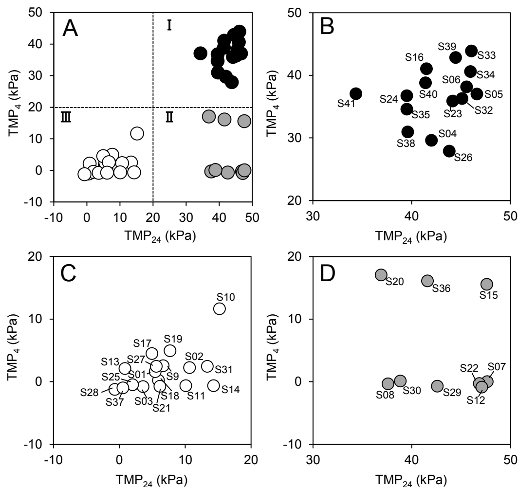
Figure 4.6 Classification of the isolated strains based on development of membrane fouling. (A) Relationship between TMP 4 and TMP 24 shown in Figure 1. The fouling patterns could be classified into three groups; I . membrane fouling is quickly developed and reached TMP > 20 kPa within 24 hr (black) (B), II . membrane fouling is gradually developed but reached TMP > 20 kPa within 24 hr (light gray) (D), and III . membrane fouling is gradually developed and reached TMP < 20 kPa after 24 hr (white) (C). The region of each group was enlarged as Fig. 4.6B , 4.6D and 4.6C , respectively.
