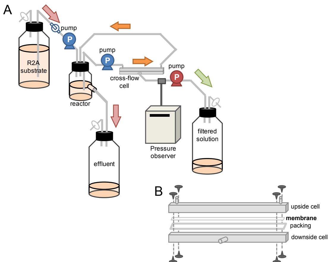
Figure 4.2 Illustrations of a bench-scale cross-flow membrane filtration system (CFMFS) (A) and a cross-flow membrane filtration cell (CFMFC) (B). Isolated bacteria were cultivated continuously in the “reactor” and circulated in the cross-flow cell as indicated with orange arrows. Fresh R2A broth medium (3.2 g/L) was fed to the reactor from a reservoir “R2A substrate” and the excess culture flowed to an “effluent” bottle as indicated with red arrows. The permeate was collected by a digital peristaltic pump as indicated with a green arrow.
