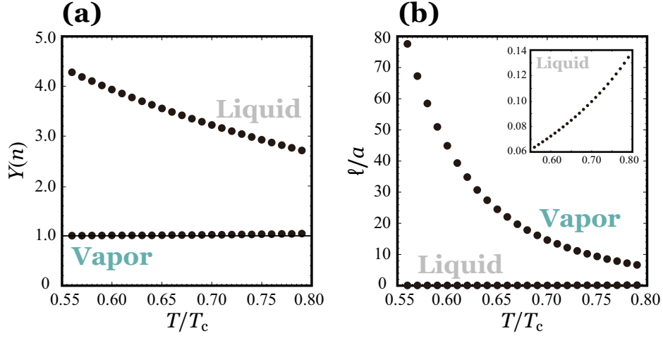
Figure 2.6: Temperature characteristics of (a) the pair correlation function Y(n) and (b) the mean free path \ell ; each abscissa is normalized by the critical temperature T_c , and the ordinate of (b) is normalized by the molecular diameter a .
