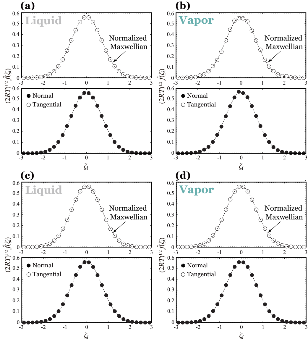
Figure 2.5: Velocity distribution function in the cases of (a) T/T_c = 0.56 and z/a = 0.1a , (b) T/T_c = 0.56 and z/a = 19.9 , (c) T/T_c = 0.79 and z/a = 0.1 , and (d) T/T_c = 0.79 and z/a = 19.9 .
