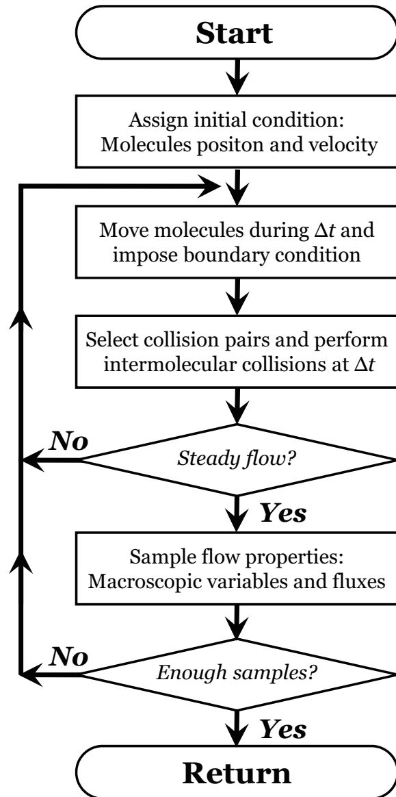
Figure 2.1: Flowchart of the EV-DSMC algorithm.
