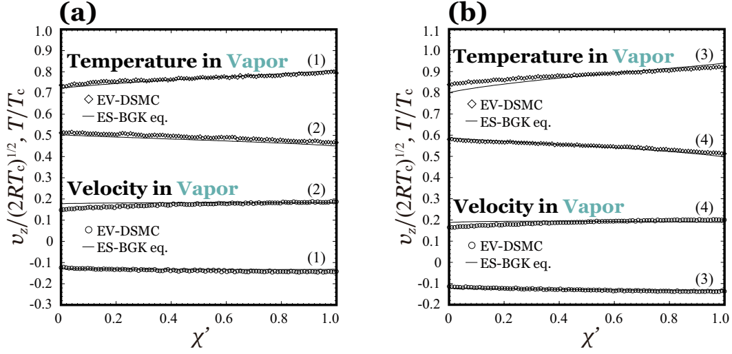
Figure 5.4: Comparison of the velocity v_z and the temperature T in vapor obtained from the EV-DSMC simulation and the numerical simulation of the ES-BGK equation for the quasi-steady pseudo half-space problem in the cases of (a) T_L/T_c = 0.60 ((1) \nu = 1.5 and (2) \nu = 0.5 ) and (b) T_L/T_c = 0.68 ((3) \nu = 1.5 and (4) \nu = 0.5 ); \chi' is the spatial coordinate ( \chi' = 0 indicates the vapor–liquid interface, and \chi' = 1 indicates the right-side end of the sampling window in Fig. 5.1), and the ordinates are normalized by the critical values.
