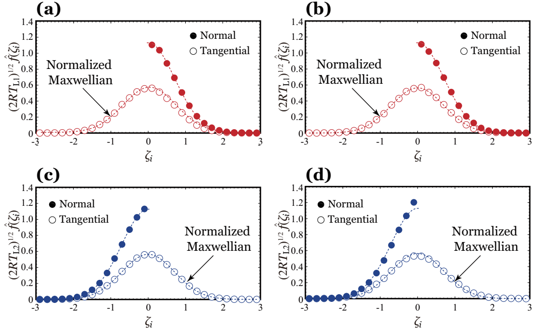
Figure 3.4: Normalized velocity distribution function of the KBC at the vapor–liquid interface of the reference liquid at T_L/T_c = 0.60 obtained from the EV-DSMC simulation in the cases of (a) T_{L1}/T_c = 0.60 and T_{L2}/T_c = 0.56 (net evaporation), (b) T_{L1}/T_c = 0.60 and T_{L2}/T_c = 0.59 (net evaporation), (c) T_{L1}/T_c = 0.68 and T_{L2}/T_c = 0.60 (net condensation), and (d) T_{L1}/T_c = 0.76 and T_{L2}/T_c = 0.76 (net condensation).
