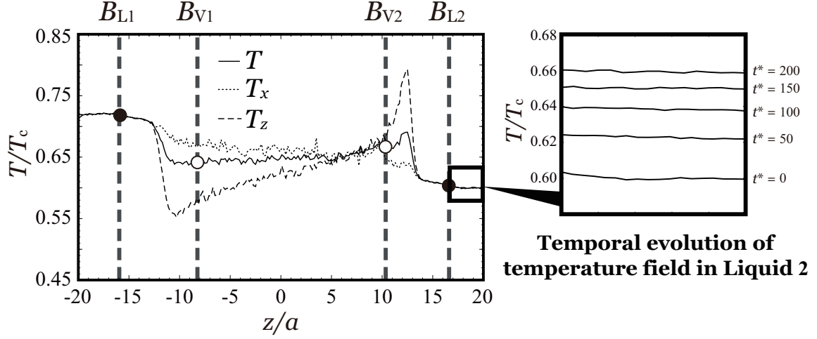
Figure 5.7: Spatial distributions of the various temperatures at t^* = 0 ; the abscissa is normalized by the molecular diameter a , and the ordinate is normalized by the critical temperature T_c . (enlarged view) Temporal evolution of the temperature field in liquid 2.
