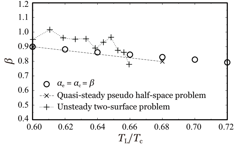
Figure 5.12: Liquid temperature dependence of \beta(T_L) in the quasi-steady pseudo half-space problem and the unsteady two-surface problem; the abscissa is normalized by the critical temperature T_c .
