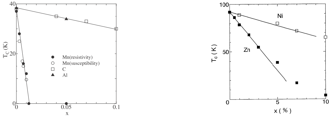
Figure 3.8: The relation of T_c and the impurity doping ratio x . Left: \text{Mg}_{1-x}\text{M}_x\text{B}_2 ( M = \text{Mn}, \text{Al} ) and \text{Mg}(\text{B}_{1-x}\text{C}_x)_2 [30]. Right: \text{YBa}_2(\text{Cu}_{1-x}\text{M}_x)_3\text{O}_7 ( M = \text{Zn}, \text{Ni} ). [31]
