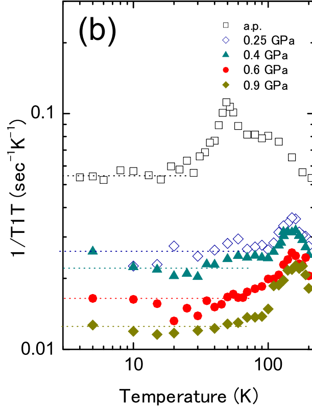
Figure 2.1: Temperature dependence of 1/T_1T of \kappa -NCS under several pressures [11].
