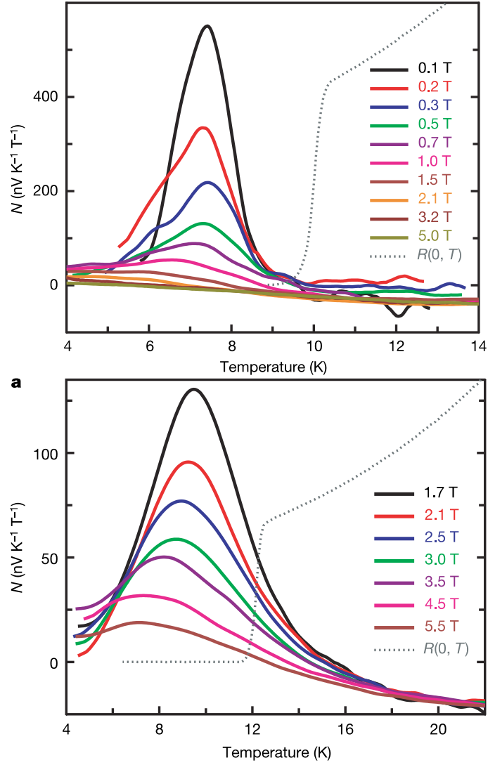
Figure 3.16: Temperature dependence of Nernst signal of \kappa -NCS (upper panel) and \kappa -Br (lower panel) salts under the various magnetic fields (solid lines) and resistivity at the zero field (dotted lines) [46]
