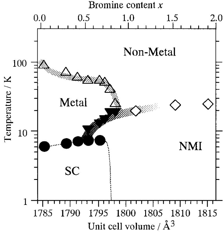
Figure 6.12: Phase diagram of \lambda -(BETS) 2 GaBr x Cl 4-x . Horizontal and vertical axis corresponds to the cell volume and temperature, respectively. SC and NMI represents the superconductor and nonmagnetic insulator [65].
