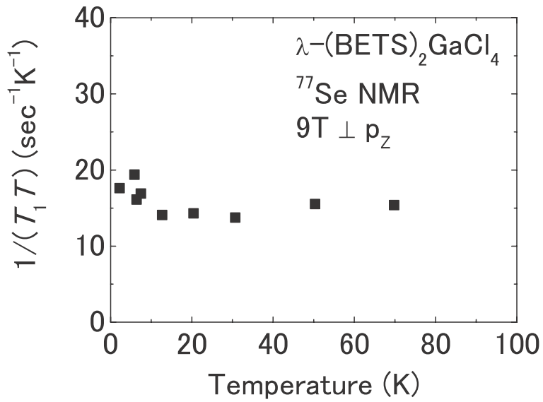
Figure 6.13: Temperature dependence of 1/T_1 T in 77 Se NMR [76].
