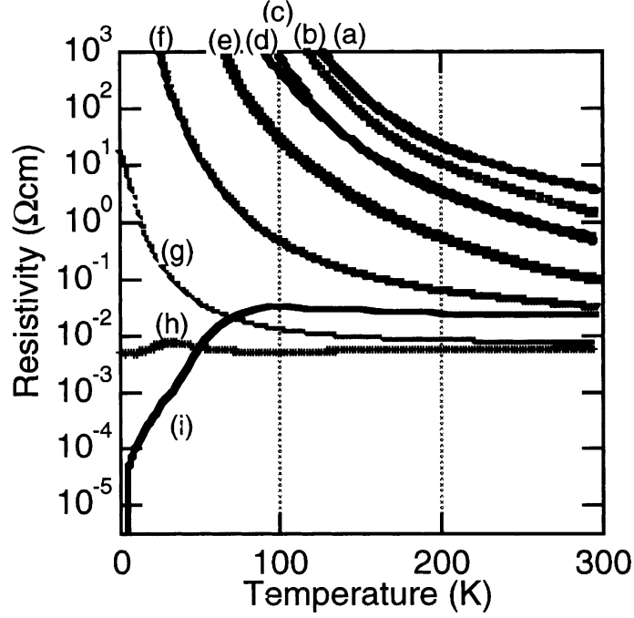
Figure 6.6: Temperature dependence of resistivity for \lambda - D_2GaCl_4 under applying pressures [72]. Applying pressures are (a) ambient pressure, (b) 0.45, (c) 1.65 GPa in \lambda -(BEDT-TTF) _2GaCl_4 salt, (d) ambient pressure, (e) 0.45, (f) 1.35, (g) 1.73, (h) 1.8 GPa in \lambda -(BEDT-STF) _2GaCl_4 salt, and (i) ambient pressure in \lambda -(BETS) _2GaCl_4 salt.
