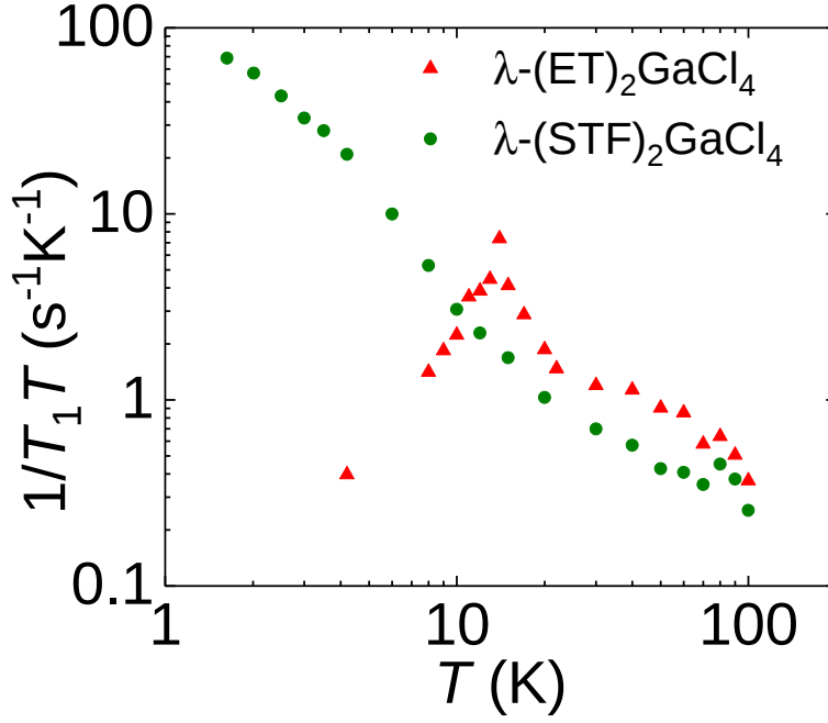
Figure 6.8: Temperature dependence of 1/T_1T in \lambda -(BEDT-TTF) 2 GaCl 4 and \lambda -(BEDT-STF) 2 GaCl 4 salts using 13 C NMR.
