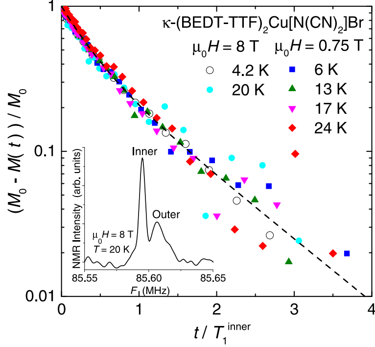
Figure 4.4: Recovery profile of nuclear magnetization of \kappa -Br at several magnetic fields and temperatures. The horizontal axis was scaled by T_1^{\text{inner}} determined at each temperature.
