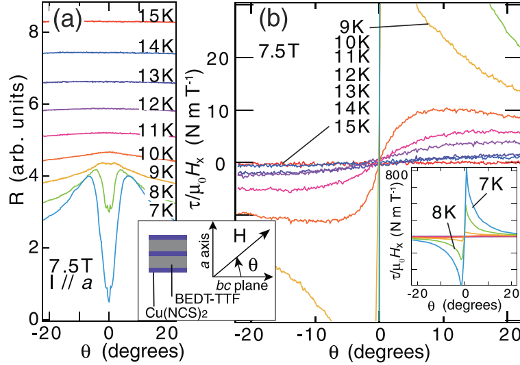
Figure 3.17: Angular dependence of the (a) interlayer resistance and (b) magnetic torque at 7.5 T for various temperatures in \kappa -NCS. The inset of (a) shows a schematic of the crystal structure and the definition of the field angle. The inset of (b) shows the overall views of the torque curves [49].
