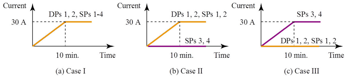
Figure 8. Three different charging cases.
