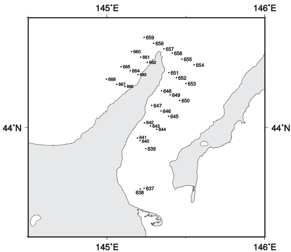
Figure 3. Oceanographic stations (Cruise 238; 2 maps)
