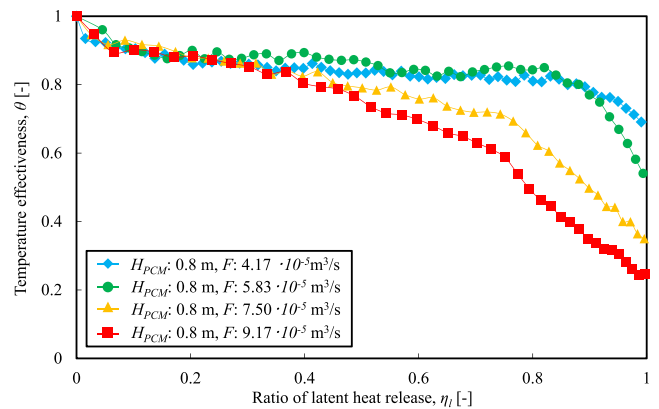
Fig. 5. Changes in temperature effectiveness \theta with latent heat release ratio \eta_l under condition of constant H_{PCM} : 0.8 m and different F . The range of F is 4.17 \cdot 10^{-5} \text{ m}^3/\text{s} \leq F \leq 9.17 \cdot 10^{-5} \text{ m}^3/\text{s} . It should be noted that an increase in \eta_l indicates the progress of the latent heat release and a decrease in liquid PCM. (Online version in color.)
