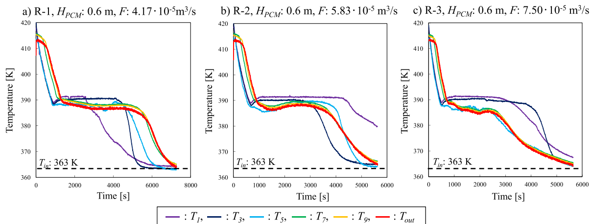
Fig. 2. Changes in local temperature in HSU and T_{out} in a) R-1: H_{PCM} : 0.6 m, F : 4.17 \cdot 10^{-5} \text{ m}^3/\text{s} , b) R-2 H_{PCM} : 0.6 m, F : 5.83 \cdot 10^{-5} \text{ m}^3/\text{s} , and c) R-3, H_{PCM} : 0.6 m, F : 7.50 \cdot 10^{-5} \text{ m}^3/\text{s} . (Online version in color.)
