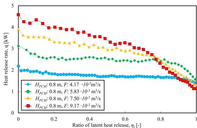
Fig. 6. Changes in heat exchange rate q with latent heat release ratio \eta_l under condition of constant H_{PCM} : 0.8 m and different F . The range of F is 4.17 \cdot 10^{-5} \text{ m}^3/\text{s} \leq F \leq 9.17 \cdot 10^{-5} \text{ m}^3/\text{s} . It should be noted that an increase in \eta_l indicates the progress of the latent heat release and a decrease in liquid PCM. (Online version in color.)
