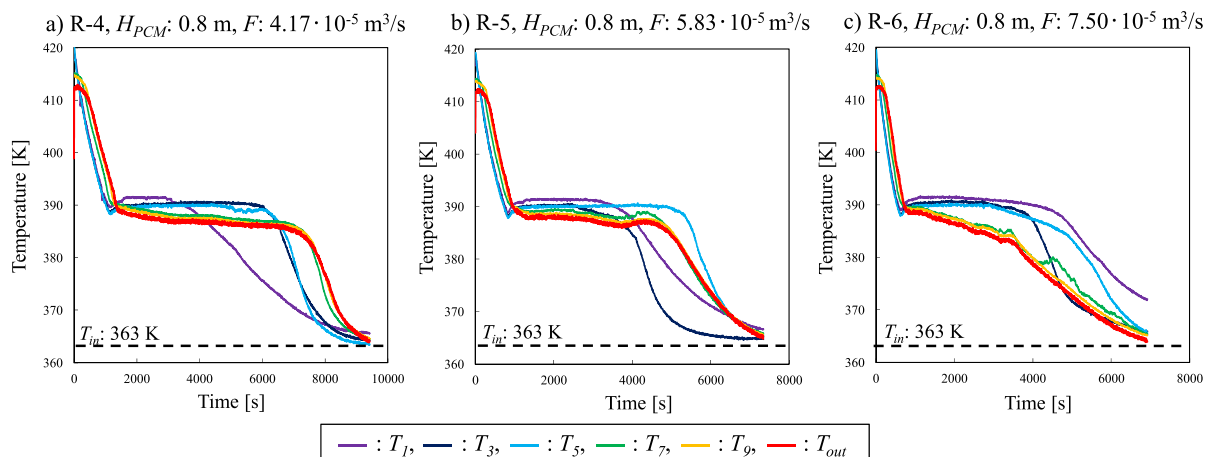
Fig. 3. Changes in local temperature in HSU and T_{out} in a) R-4: H_{PCM} : 0.8 m, F : 4.17 \cdot 10^{-5} \text{ m}^3/\text{s} , b) R-5 H_{PCM} : 0.8 m, F : 5.83 \cdot 10^{-5} \text{ m}^3/\text{s} , and c) R-6, H_{PCM} : 0.8 m, F : 7.50 \cdot 10^{-5} \text{ m}^3/\text{s} . (Online version in color.)
