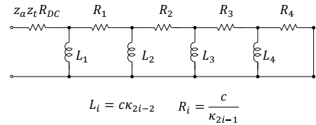
Fig. 6 Equivalent Caer circuit of winding considering proximity effect.
