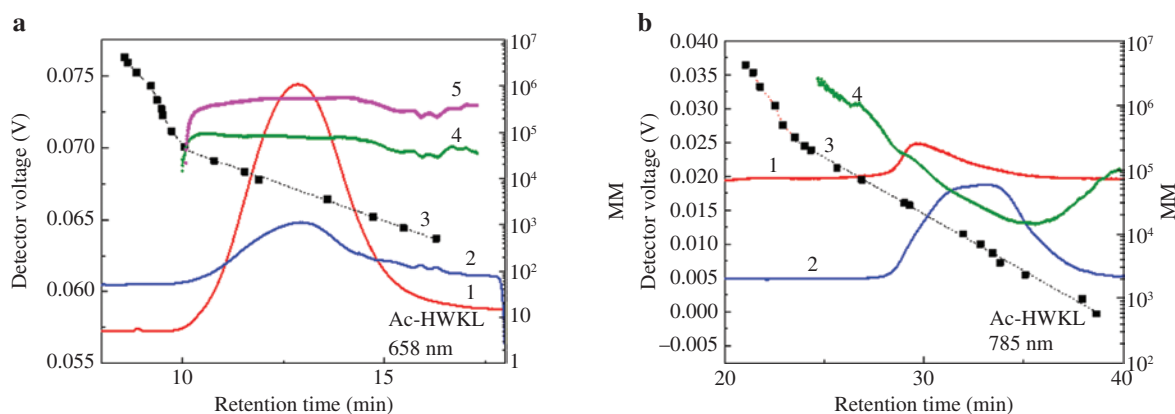
Figure 3: SEC-MALLS-RI chromatograms of Ac-HWKL obtained at 658 nm (a) and 785 nm (b).
