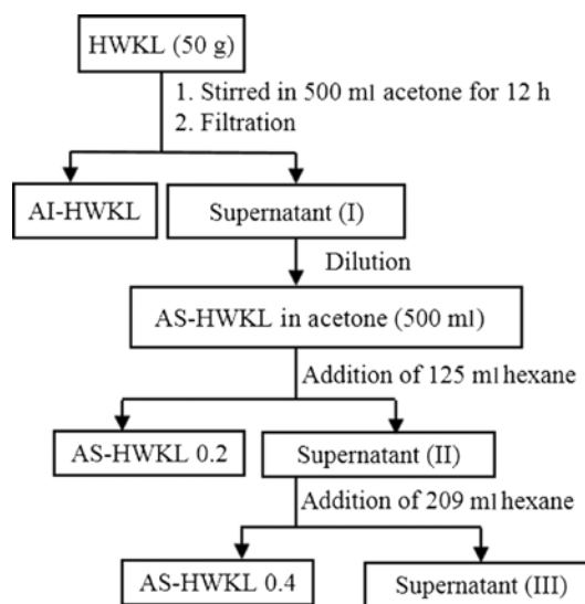
Scheme 1: HWKL fractional precipitation procedure.
