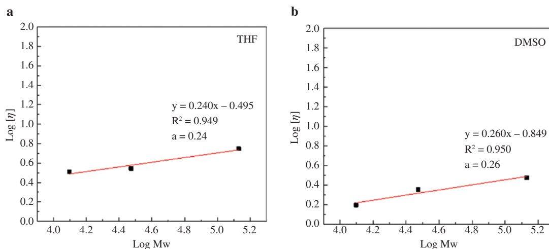
Figure 4: Logarithmic plot of [\eta] versus the absolute Mw for Ac-HWKL fractions in (a) THF and (b) DMSO.
