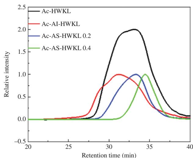
Figure 1: Size-exclusion chromatograms of acetylated HWKL and its fractions monitored by an RI detector in the Shimadzu LC system.
