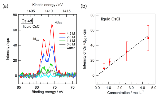
FIG. 4. (a) Cs 4d photoelectron spectra of pure water and 0.6, 1.1, 2.6, and 4.5 M aqueous CsCl solutions in environmental cells. Each spectrum was collected with an acquisition time of \sim 200 min. Linear approximation was adopted for background subtraction. (b) Concentration-dependence of the intensity of the Cs 4d_{5/2} peak. The black dashed line is a linear fit to the data.
