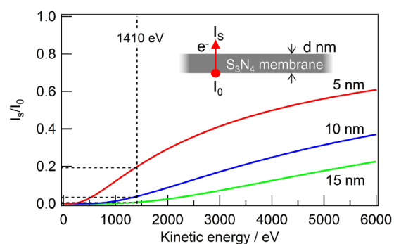
FIG. 2. Attenuation ratio of the photoelectron intensity ( I_s/I_0 ) passing through the 5 nm (red), 10 nm (blue), and 15 nm-thick (green) \text{Si}_3\text{N}_4 membranes as a function of the kinetic energy of photoelectrons.
