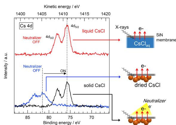
FIG. 3. Cs 4d photoelectron spectra acquired from the cells filled with a 4.5 M aqueous CsCl solution without charge neutralization (red curve) and a dry solid CsCl sample without (blue curve) and with charge neutralization (black curve).
