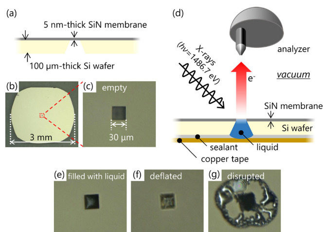
FIG. 1. (a) Cross-sectional and (b) top views of the Si chip and (c) a magnified image of the quasi-transparent SiN membrane. (d) Schematic illustration of the environmental cell and configuration of the XPS system. Photographs of the quasi-transparent windows used for screening: (e) filled with a liquid sample, (f) deflated, and (g) disrupted causing leakage of the liquid sample.
