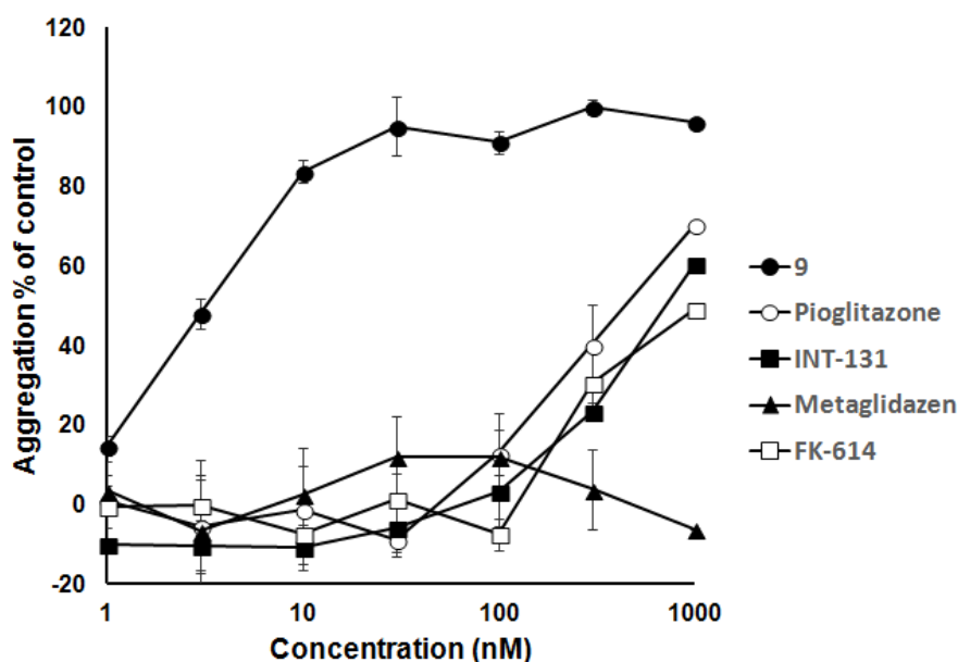
Figure 8. Aggregation activities of PPAR \gamma ligands in MKN-45 cells. The aggregation of MKN-45 cells was evaluated using an IN Cell Analyzer 1000 (GE Healthcare) after treatment of compounds for 5 days. The efficacy of 9 was calculated using its ratio of cell-aggregated clusters as the control value. The
