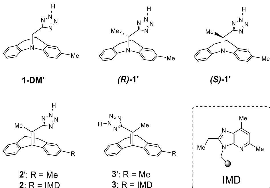
Figure 5. Chemical structures of model substrate for conformation studies and compound 2,3.
