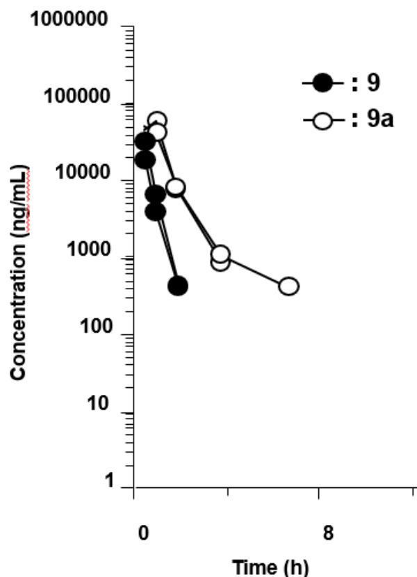
Figure 15. Plasma concentrations of 9 and 3-fluoro-dibenzooxepine derivative 9a in BALB/c mice orally administered (30 mg/kg, n = 2 ).
