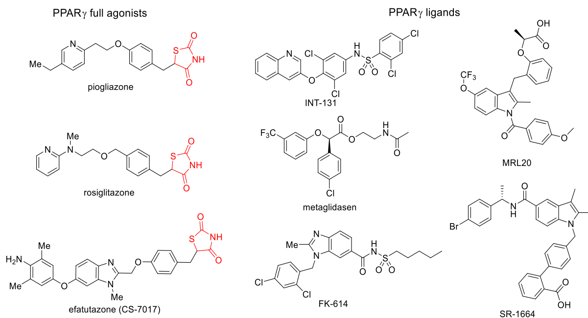
Figure 1. Chemical structures of PPAR \gamma full agonists and ligands. The structures of TZD are showed in red.
