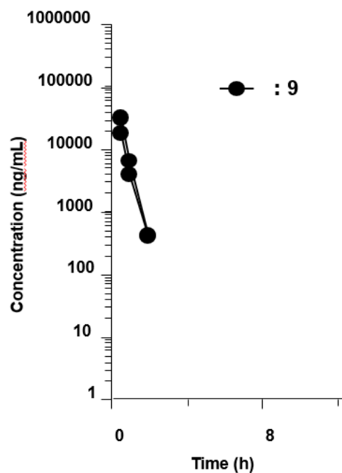
Figure 13. Plasma concentrations of 9 after its oral administration in BALB/c mice (30 mg/kg, n = 2 ).
