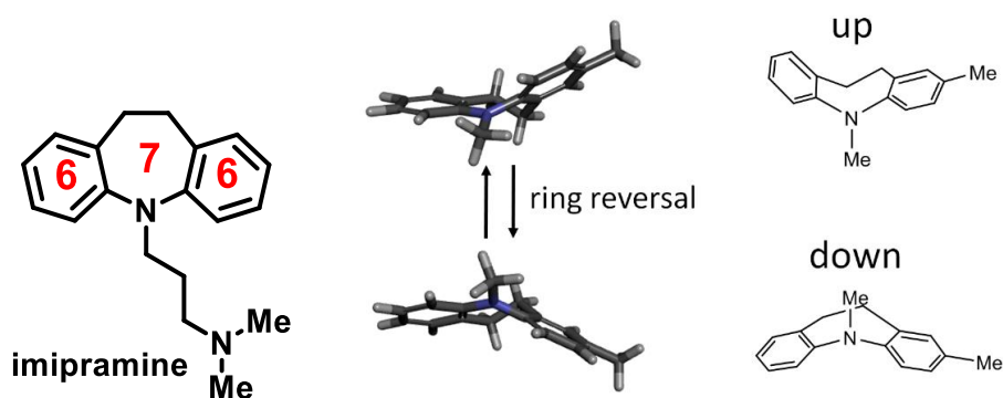
Figure 4. Ring reversal motion of the 6-7-6-tricyclic ring systems.
