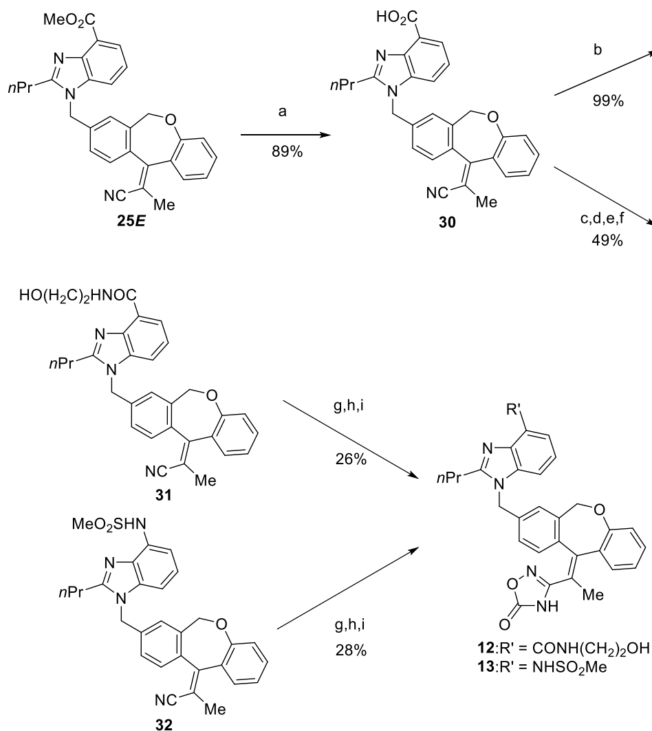
Scheme 4. Modification of the substituents in 4-position on benzimidazole ring a
