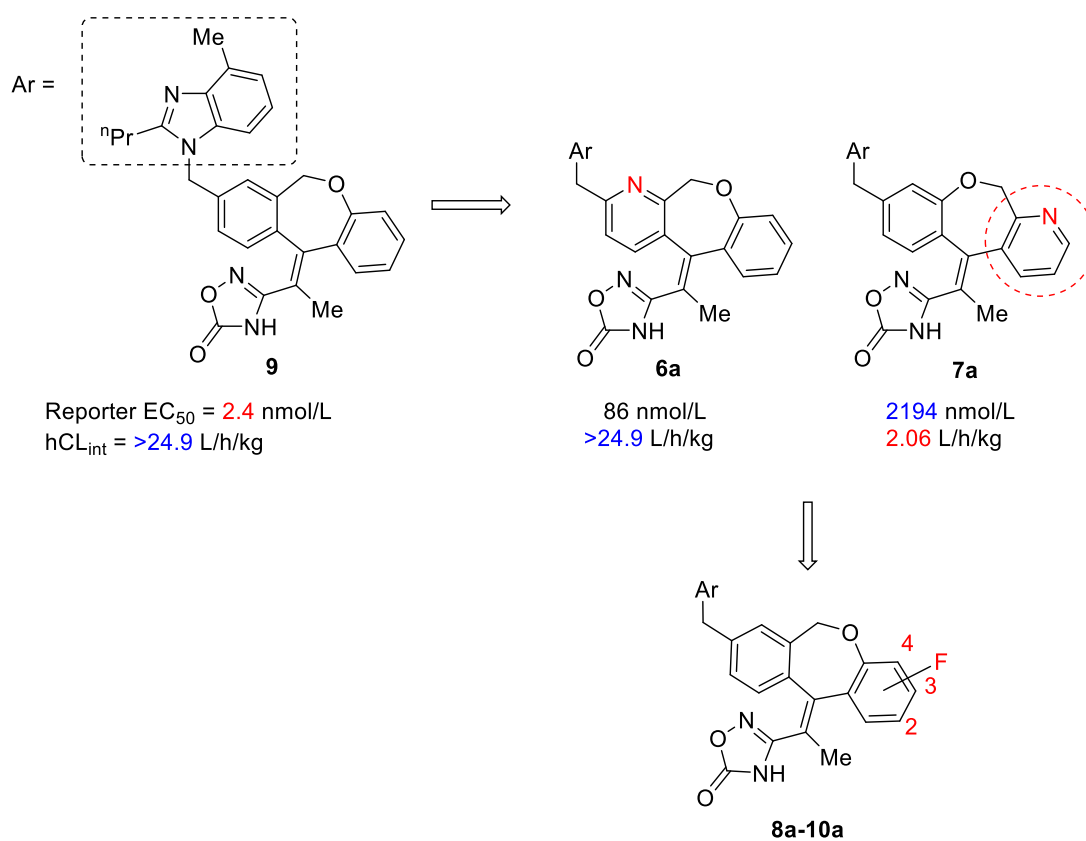
Figure 14. Improvement of the human metabolic stability of lead compound 9 by modification of the tricyclic core-structure.
