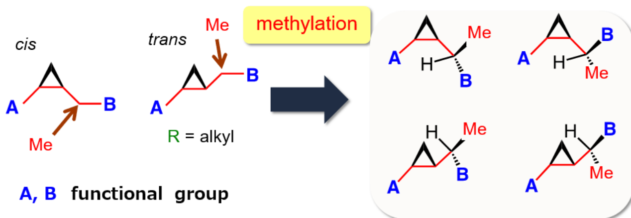
Figure 3. Conformational restriction by methyl group in cyclopropane scaffolds.
