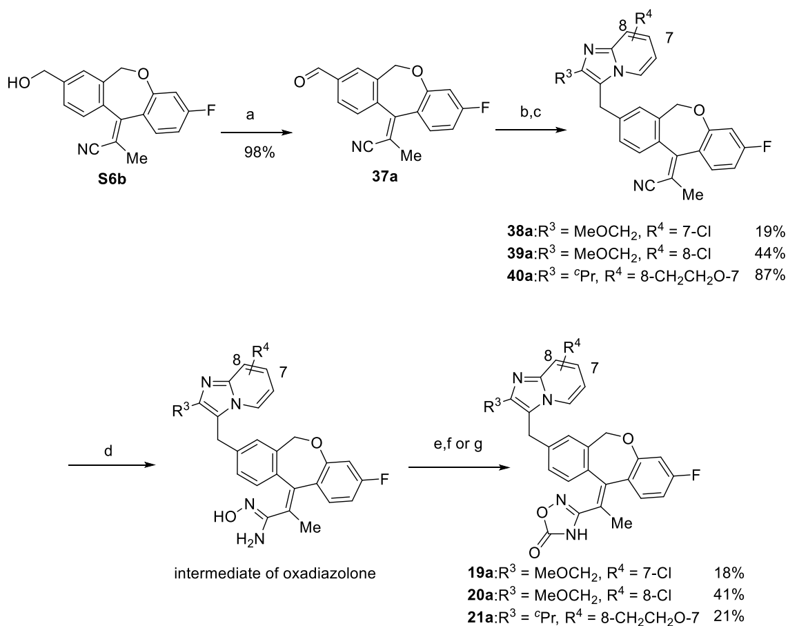
Scheme 7. Synthesis of the side chain structure from 8-formyldibenzooxepine a
