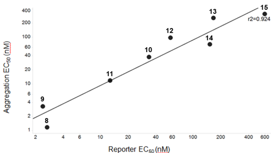
Figure 10. The correlation of the EC 50 values of tricyclic compounds 8 – 15 on the aggregation of MKN-45
