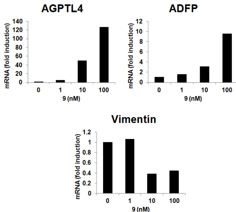
Figure 9. The gene expression in MKN-45 cells after the treatment of 9 at 1–100 nM. The gene expression was determined by quantitative PCR using an ABI PCR system. The fold-inductions are shown as the values relative to baseline.
