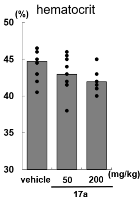
Figure 18. Hematocrit values in CD-1 mice treated orally with 17a twice a daily at 50 and 200 mg/kg. p = 0.671 between the vehicle-treated group and the 17a 50 mg/kg-treated group. p = 0.176 between the vehicle-treated group and the 17a 200 mg/kg-treated group.
