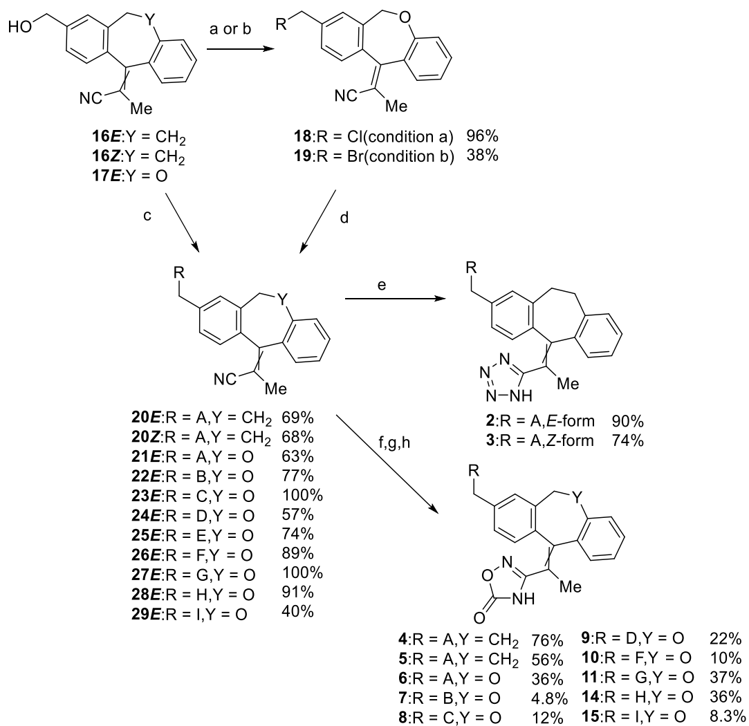
Scheme 3. Synthesis of dibenzocycloheptane and dibenzoxepine compounds a
