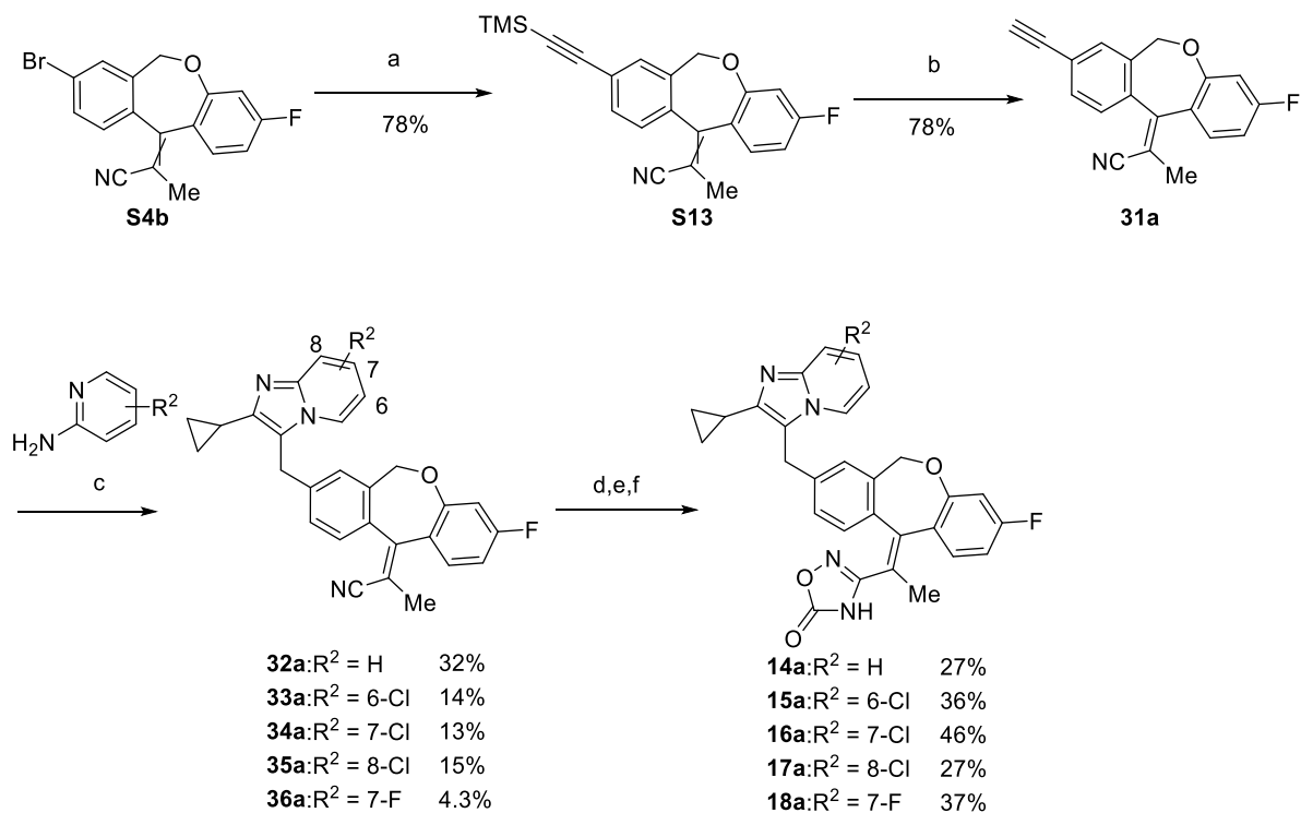
Scheme 6. Introduction of the substituents to benzo[1,2- a ]imidazole ring a
