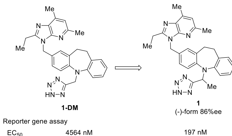
Figure 2. Chemical structure and reporter activity of compound 1 .
