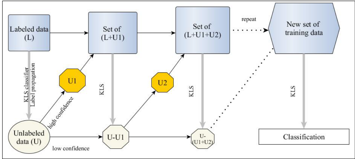
Figure 2.3. Flowchart of classification using the combination of self-learning with kernel least squares classifier in this study
