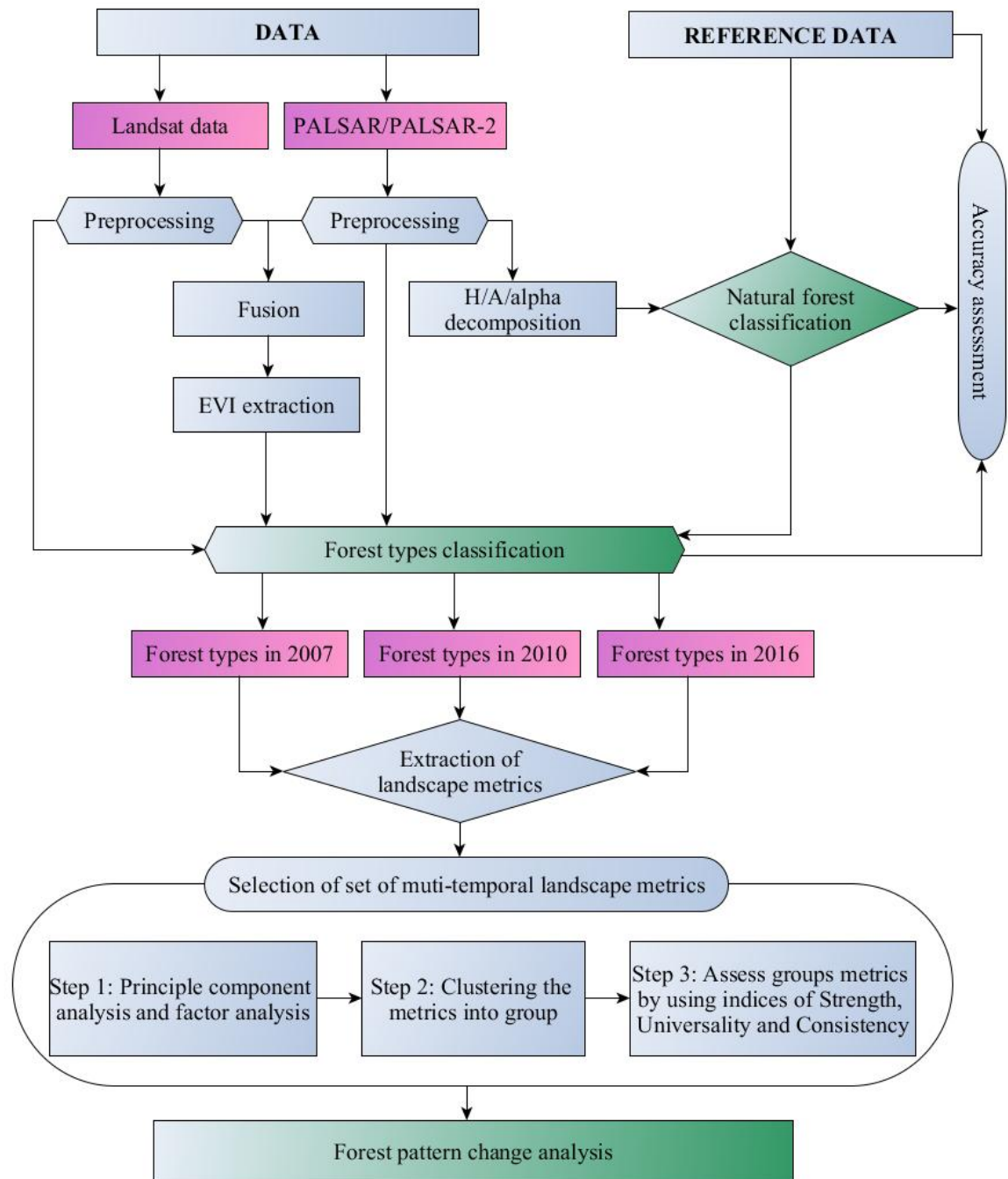
Figure 2.2. Flowchart of the methodology employed in this study
