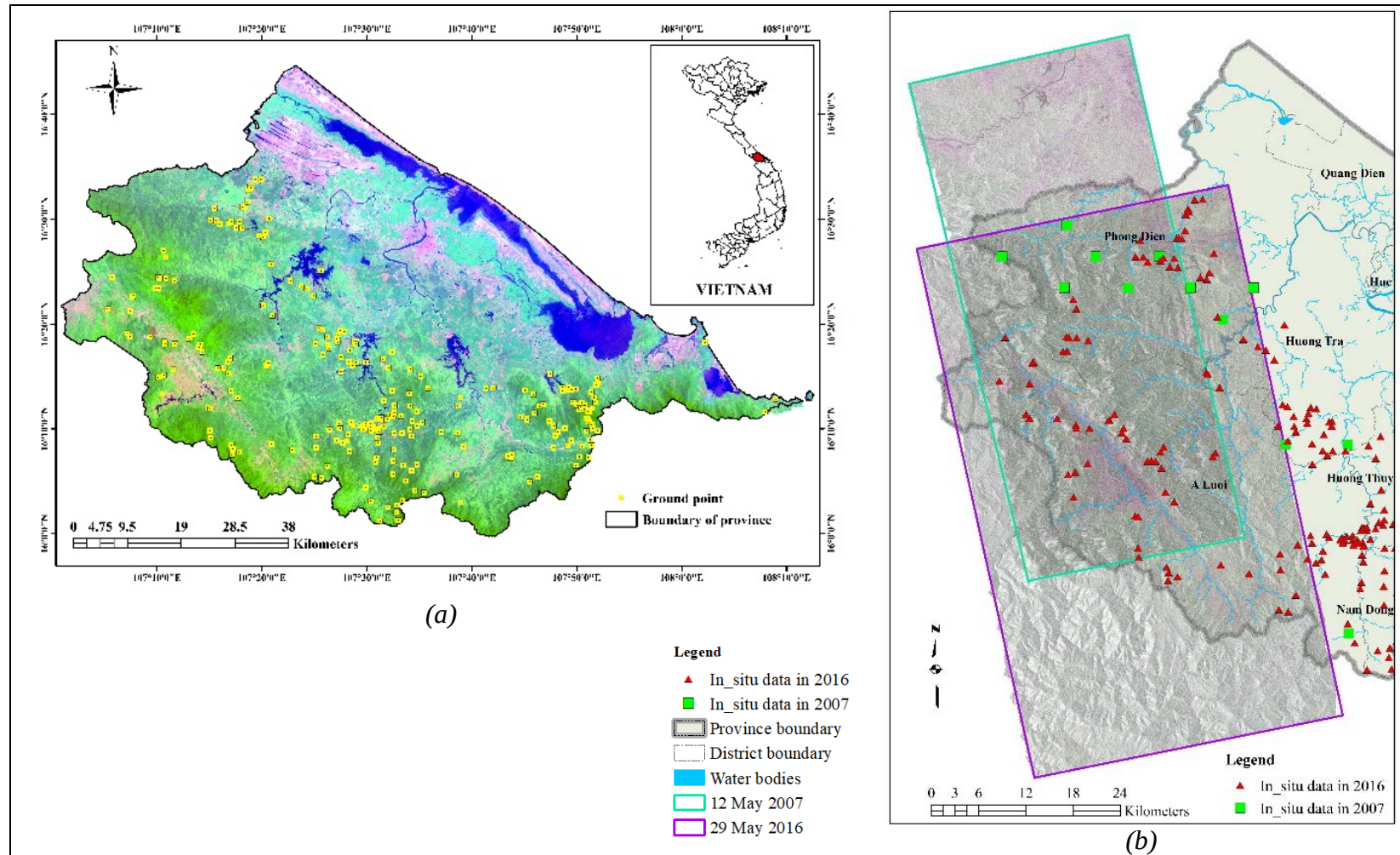
Figure 3.1. Location map of the study area in Landsat TM in pseudo-colors band 7,5,2 (a), and the cover of SAR images and in-situ data in 2007 and 2016 (b)
