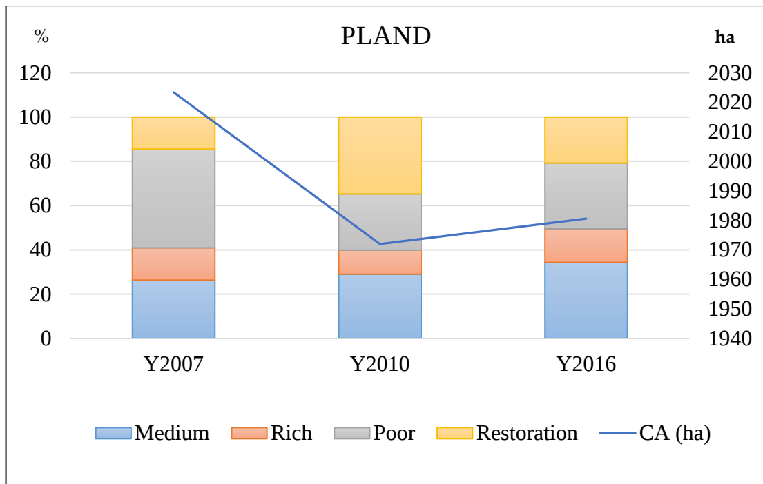
Figure 2.5. Variation of four forest grades in the total class area of natural forest (CA_ha) and percentage of landscape (PLAND_%) for each forest type
