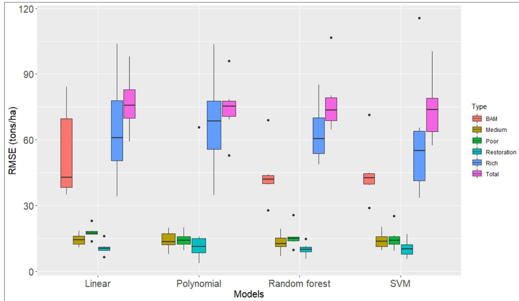
Figure 3.4. Root mean squared error (RMSE) of regression models in tons/ha using 10-fold cross-validation for different forest grades
