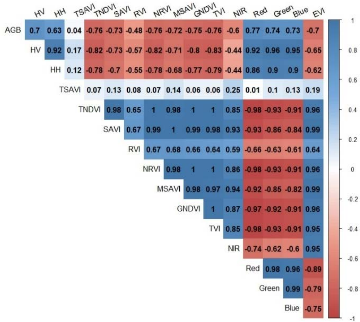
Figure 4.2. Pearson's correlation coefficient (R) between aboveground biomass and different remotely sensed parameters
