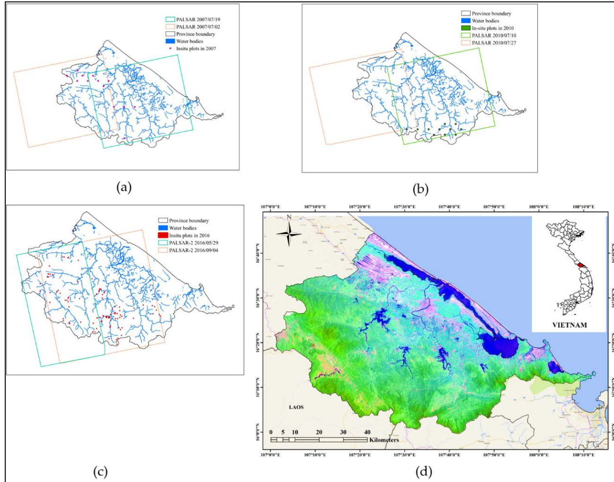
Figure 2.1. Cover of synthetic aperture radar (SAR) images and in-situ data in (a) 2007, (b) 2010, (c) 2016, and (d) location map of the study area in Landsat data with pseudo colors (R: SWIR 2, G: near-infrared, B: green)
