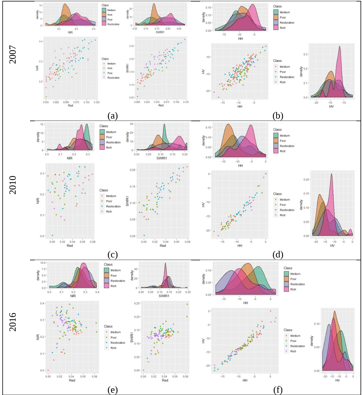
Figure C1. Distribution and density of some parameters (HH and HV signals in decibels for SAR data, and red, near-infrared, and shortwave infrared 1 in reflectance for Landsat data) in four forest grades in three years 2007 (a,b), 2010 (c,d), and 2016 (e,f)
