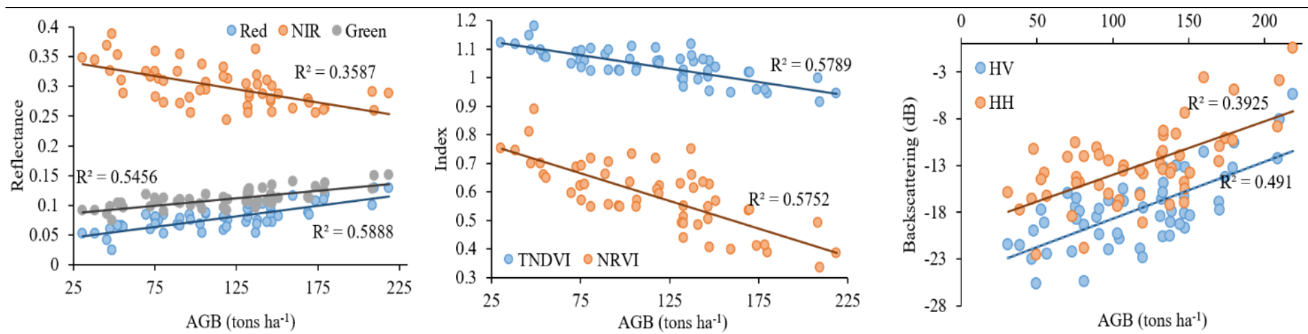
Figure 4.3. Linear regression between aboveground biomass and Landsat reflectance in Green, Red, and NIR (left panel); Vegetation indices in TNDVI and NRVI (middle panel); and PALSAR-2 backscattering in HH and HV (right panel)
