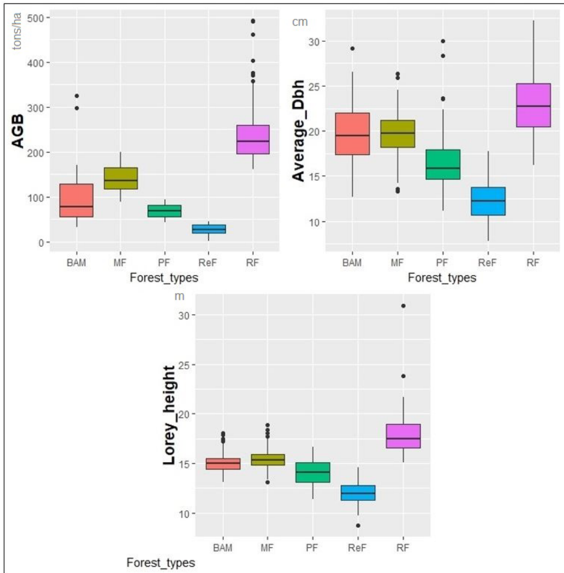
Figure 3.2. Boxplots of average above-ground biomass (AGB), Diameter at breast height (DBH), and Lorey's height ( H_{\text{Lorey}} ) of plots in the five forest grades
