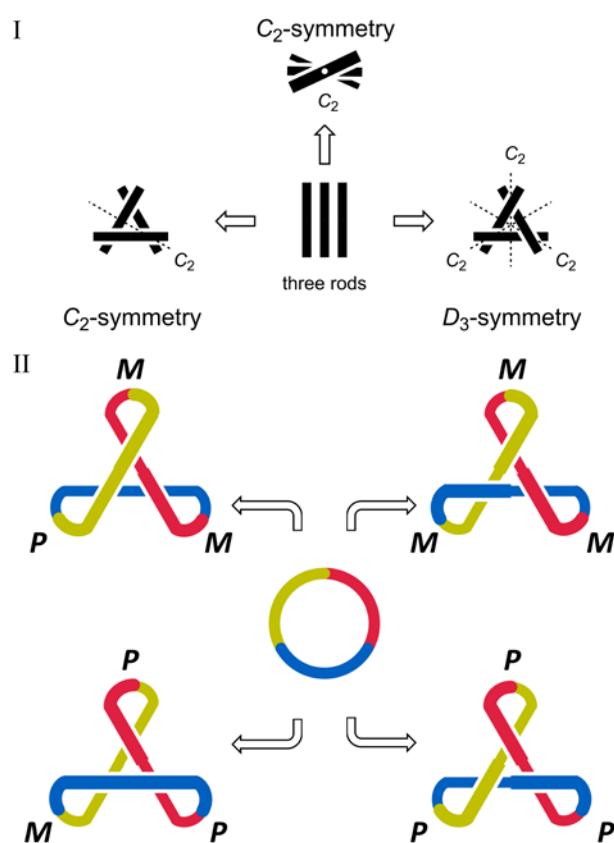
Scheme 1 Chirality generated (I) in assemblies of three achiral rods, and (II) in a macrocycle through three-fold twisting.
