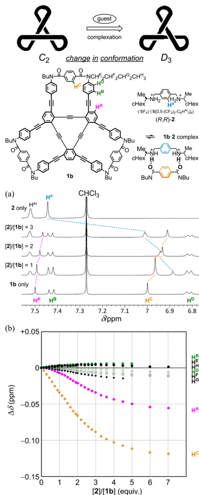
Fig. 3 (a) Partial ^1\text{H} NMR spectra (aromatic region) of 1b (0.7 mM) in the presence of (R,R) - 2 [0 ( 1b only), 1, 2 and 3 equiv.], and (R,R) - 2 . All spectra were measured in 1.7 vol% acetonitrile- d_3 /chloroform- d at 303 K; (b) titration curves based on changes in the chemical shifts ( \Delta\delta = \delta_{\text{1b}+2} - \delta_{\text{1b}} ) for protons \text{H}^{\text{A}} – \text{H}^{\text{D}} of 1b .
