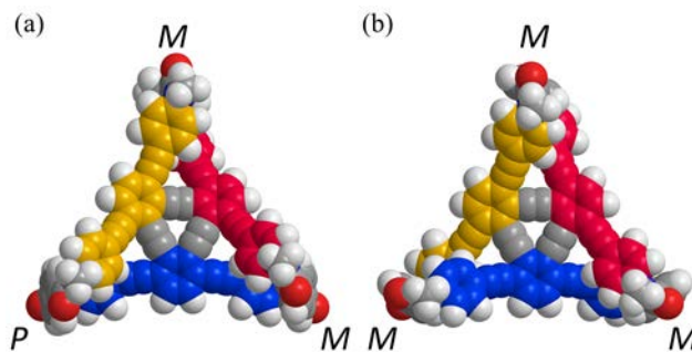
Fig. 2 Energy-minimized structures of model macrocycle 1' [X = Me] with (a) C 2 -symmetry (rel. 0 kJ mol -1 ) and (b) D 3 -symmetry (+0.80 kJ mol -1 ), obtained by a conformational search using MacroModel software (v11.8 OPLS3e, Monte Carlo Multiple Minimum method, non-solvated, 20,000 steps). Only one of two enantiomeric conformations is depicted.
