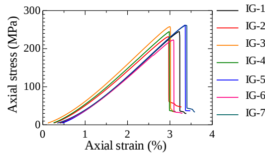
Fig. 4.3 Stress–strain curves.
