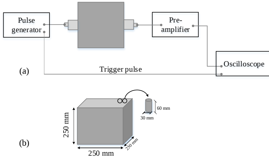
Fig. 3.2 Specimen from the Shikotsu welded tuff block. (a) Measuring P-wave velocity of the block (b) coring direction and core specimen.
