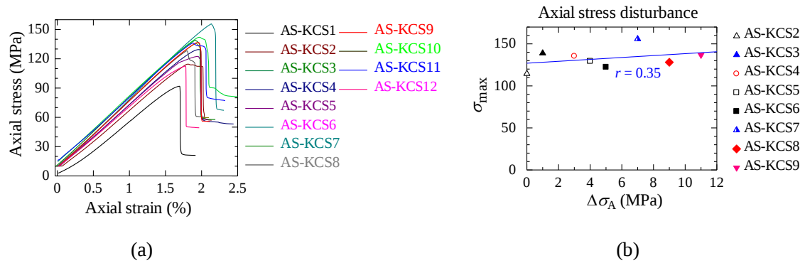
Fig. 2.6 (a) Stress–strain curves and (b) maximum stress ( \sigma_{\max} ) vs. the amplitudes of the axial stress disturbances ( \Delta\sigma_A ) under P_C = 10 MPa of the Kushiro Cretaceous sandstone.
