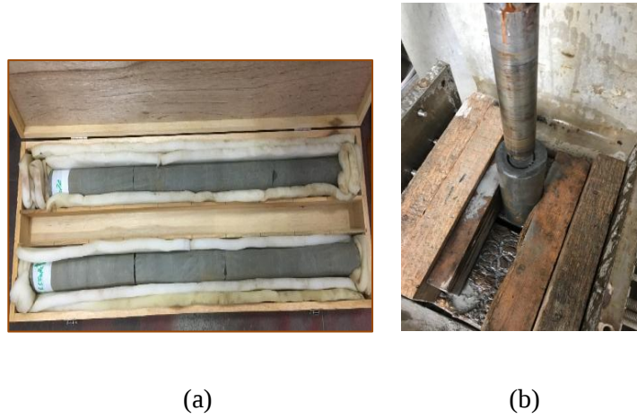
Fig. 2.3 (a) Cores of Kushiro Cretaceous sandstone and (b) Specimen coring.
