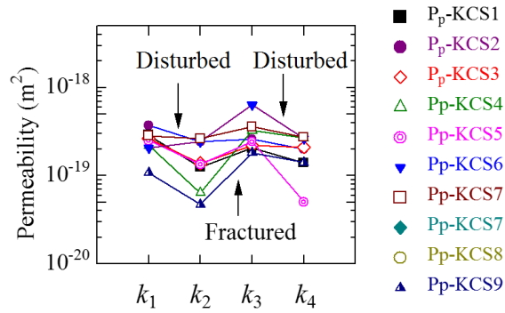
Fig. 2.14 Permeability variation due to pore pressure disturbances and triaxial compression under P_C = 10 MPa.
