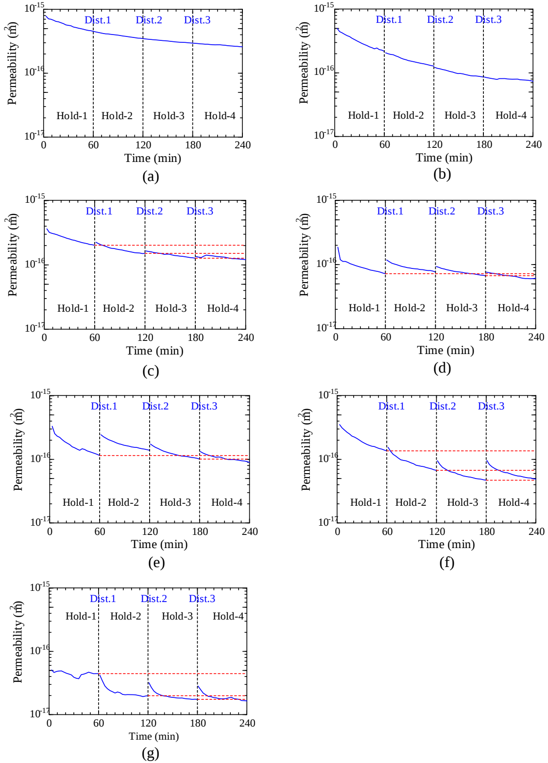
Fig. 4.6 Variations in permeability due to multiple transient axial stress disturbances: (a) IG-1, (b) IG-2, (c) IG-3, (d) IG-4, (e) IG-5, (g) IG-6, and (f) IG-7.
