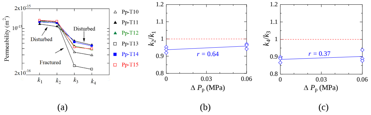
Fig. 3.9 (a) Variation in permeability and permeability ratios of the intact rocks (b) and the fractured rocks (c) due to transient pore pressure disturbances and triaxial compression of the Shikotsu welded tuff ( P_p = 0.1 MPa).
