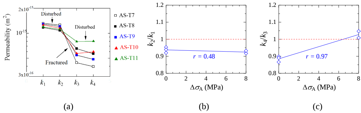
Fig. 3.7 (a) Variation in permeability, and permeability ratios of the intact rocks (b) and fractured rocks (c) ( P_p = 0.1 MPa) due to transient axial stress disturbances and the triaxial compression of the Shikotsu welded tuff.
