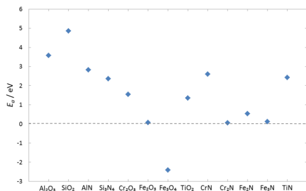
Figure 1. Calculated hydrogen absorption energy, including ZPE, in pristine ceramic materials.
