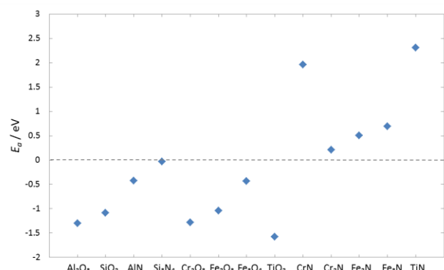
Figure 8. Calculated hydrogen absorption energy, including ZPE, in single anion-substituted ceramic materials.
