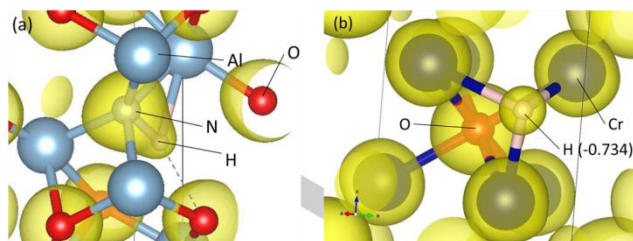
Figure 9. Electron density distribution of the most stable absorption configuration of (a) \text{Al}_2\text{O}_3 and (b) \text{Cr}_2\text{N} with single substitutional impurity. The isosurface is described at 0.7 \text{ e}/\text{\AA}^3 .
