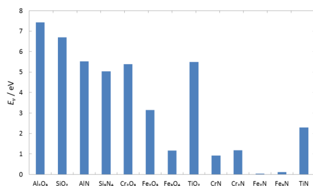
Figure 5. Calculated single anion vacancy formation energy.
