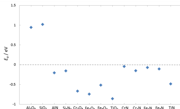
Figure 6. Calculated hydrogen absorption energy, including ZPE, in single anion-deficient ceramic materials.
