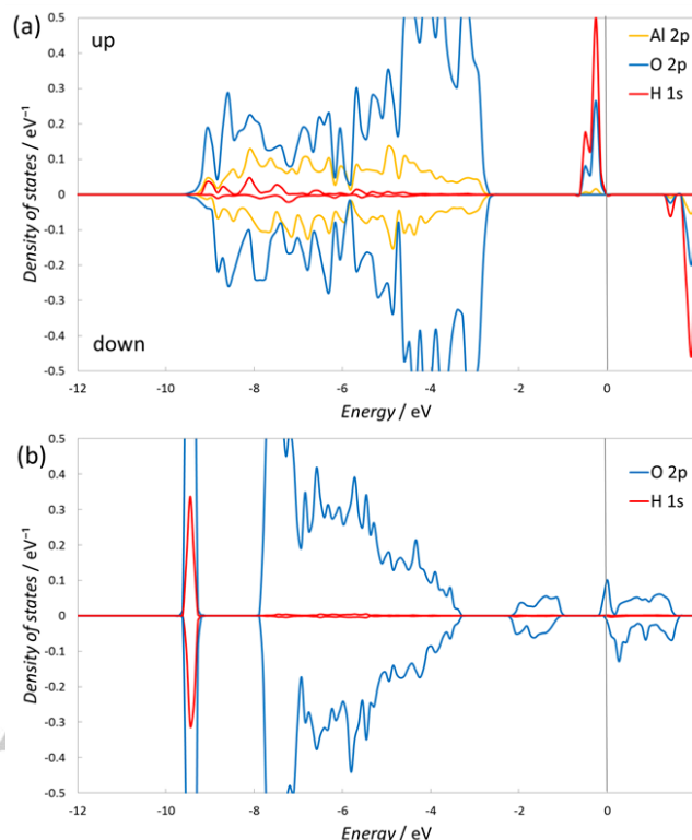
Figure 3. pDOS of a hydrogen atom adsorbed in (a) \text{Al}_2\text{O}_3 and (b) \text{Cr}_2\text{O}_3 .
