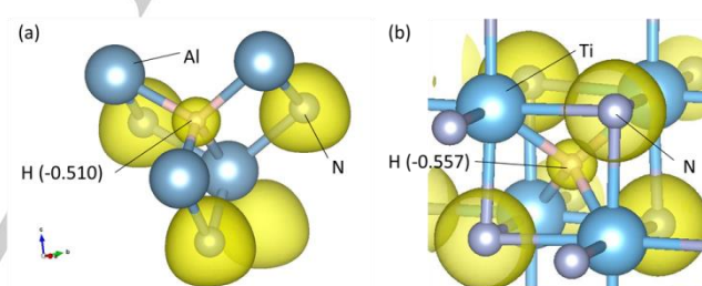
Figure 4. Electron density distribution of the most stable absorption configuration of (a) \text{AlN} and (b) \text{TiN} . The isosurface is described at 0.7 \text{ e}/\text{\AA}^3 .
