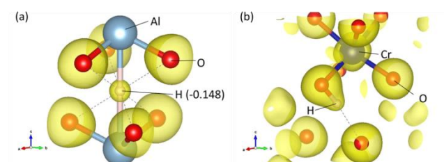
Figure 2. Electron density distribution of the most stable hydrogen absorption configuration of (a) \text{Al}_2\text{O}_3 and (b) \text{Cr}_2\text{O}_3 . The isosurface is described at 0.7 \text{ e}/\text{\AA}^3 .
