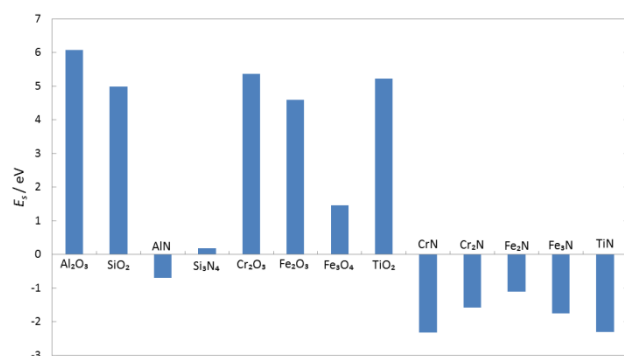
Figure 7. Calculated single anion substitution energy.
