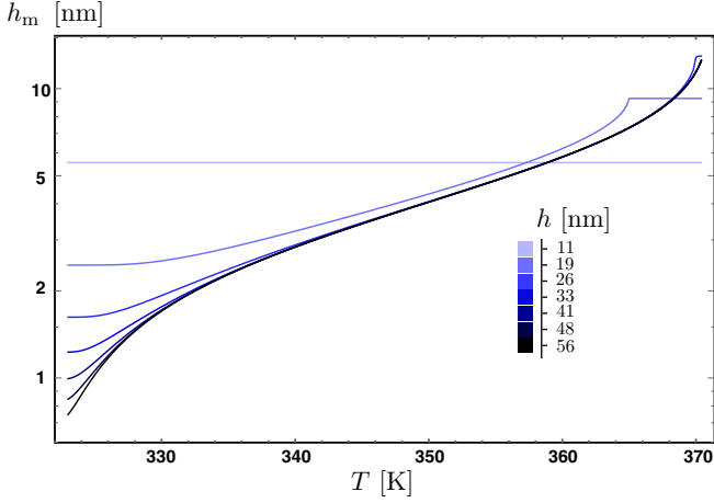
FIG. 3. Mobile layer thickness of low- M_w polystyrene freestanding films as a function of temperature for several film thicknesses, as computed from Eq. (19) and the procedure detailed in Sec. II D. The corresponding plot for low- M_w polystyrene supported films is simply obtained by replacing the label “ h ” in the legend by “ 2h ”, according to Eq. (22).
