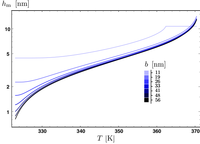
FIG. 5. Mobile layer thickness of low- M_w polystyrene cylindrical particles as a function of temperature for several particle radii, as computed from Eq. (28) and the procedure detailed in Sec. II D.
