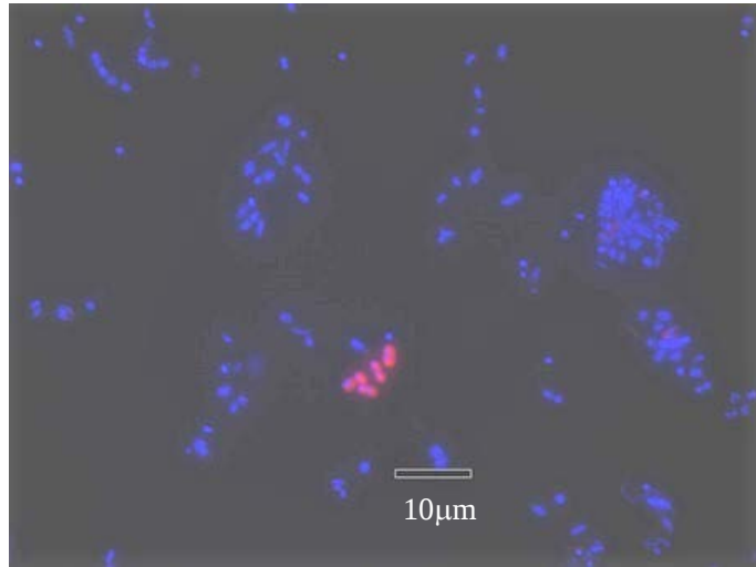
Figure 4 Detection of unknown group A bacteria in deer rumen digesta by fluorescent in situ hybridization Whole cell hybridization was carried out using winter rumen digesta of deer and Cy3 labelled probe specific to unknown group A bacteria. Unknown group A bacteria are seen in clustered cocci (Red). Other bacteria are stained with 4',6-diamidino-2-phenylindole (Blue).
