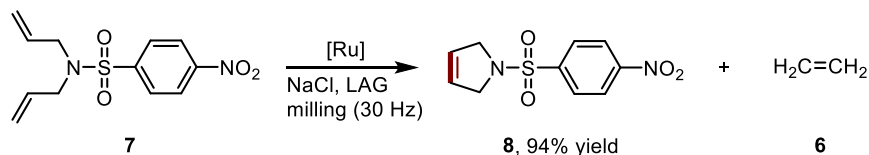
Scheme 3. Ruthenium-catalyzed olefin metathesis under mechanochemical conditions. a) Ruthenium-catalyzed cross-metathesis of solid olefins under mechanochemical conditions. b) Ruthenium-catalyzed ring-closing metathesis of solid olefins under mechanochemical conditions.
