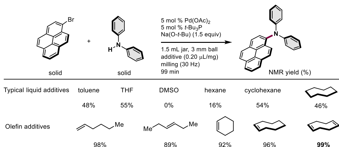
Scheme 6. Olefin-accelerated solid-state C–N cross-coupling reactions using mechanochemistry.
