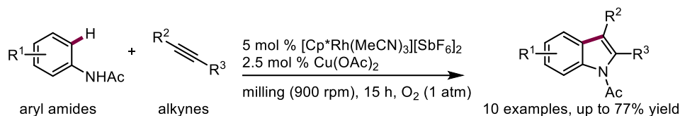
Scheme 1-1. Transition-metal-catalyzed C–H bond functionalizations using mechanochemistry. a) Oxidative Heck-type reaction, b) halogenation reaction, c) amination reaction, d) oxidative olefination reaction, e) arylation reaction, f) oxidative cyclization.
