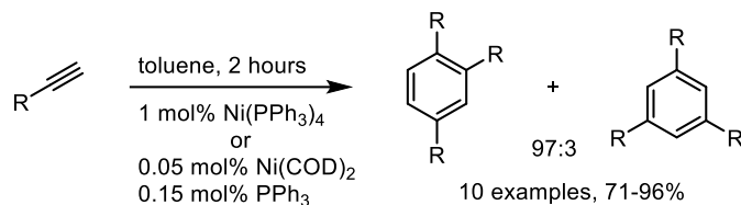
Scheme 5. Nickel(0)-catalyzed cyclization of alkynes. a) Nickel(0)-catalyzed cyclization of alkynes under mechanochemical conditions. b) Nickel(0)-catalyzed cyclization of alkynes under solution-based conditions.
