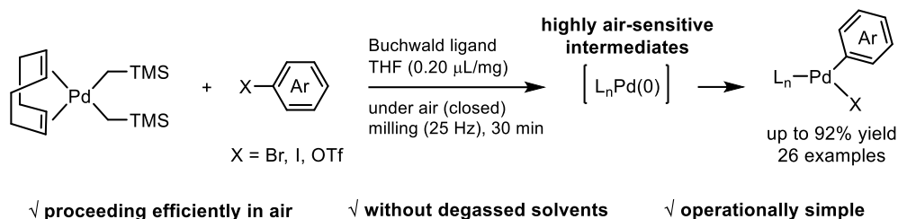
Scheme 8. Synthesis of oxidation addition complexes from aryl halide and palladium(0) using mechanochemistry.
