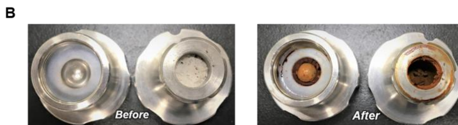
Fig. 2-2. Mechanoredox arylation and borylation using mechanical force. (A) Optimization of the mechanoredox arylation reactions. (B) Reaction mixture of the mechanoredox arylation of 2a after grinding in a ball mill. A stainless-steel milling jar (1.5 mL) and a stainless-steel ball (diameter: 5 mm) were used. See experimental section for details.
