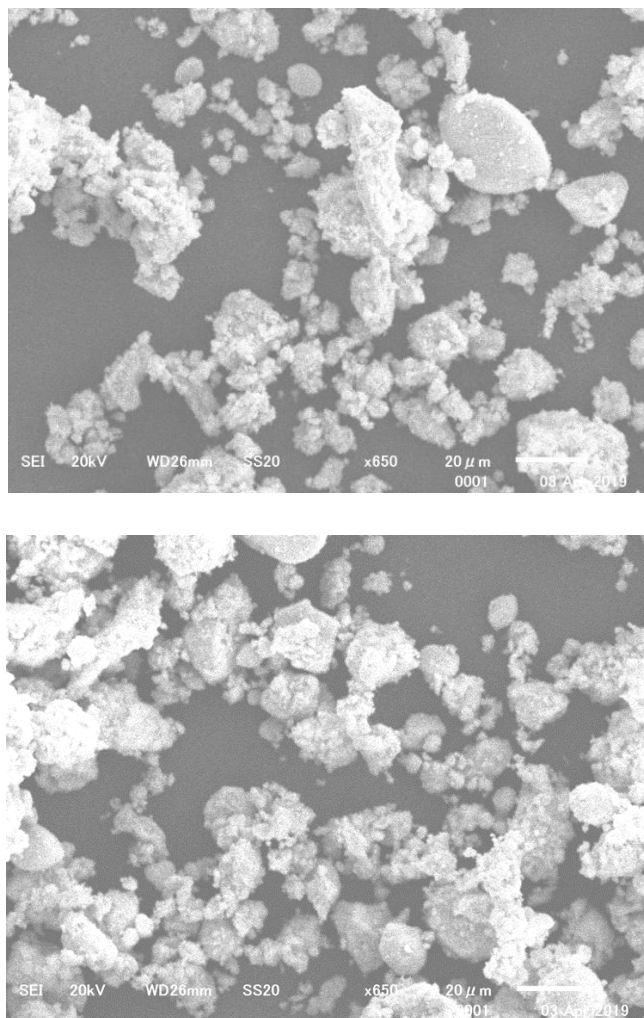
Fig. S6. SEM images of BaTiO 3 particles after ball milling (30 Hz, 1 h).
