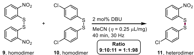
Scheme 4. Aromatic disulfide metathesis reaction. a) aromatic disulfide metathesis reaction under solution-based conditions. b) aromatic disulfide metathesis reaction under mechanochemical conditions.
