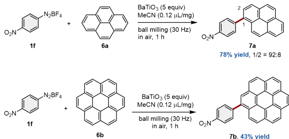
Fig. 2-4. Exploration of a gram-scale synthesis, catalyst recycling, and the arylation of polyaromatic hydrocarbon compounds. (A) Mechanochemical arylation of 2a with 1o on the gram scale using a 25-mL ball-milling jar (picture on the right). (B) \text{BaTiO}_3 recycling experiments using 1k and 2a . (C) Mechanochemical arylation of the polyaromatic hydrocarbons 6 with 1f . See experimental section for details.
