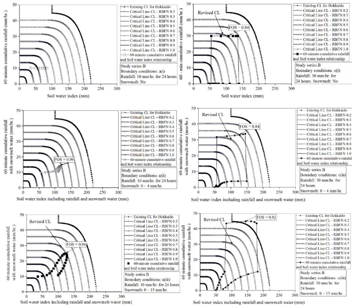
Figure 22 Revision of CL for SWI based on occurrence and non-occurrence of slope failures using data from study series B with 45° slope angle, 5 m slope height, 10 mm/hr. and 30 mm/hr. rainfall with two different snowmelt rates
