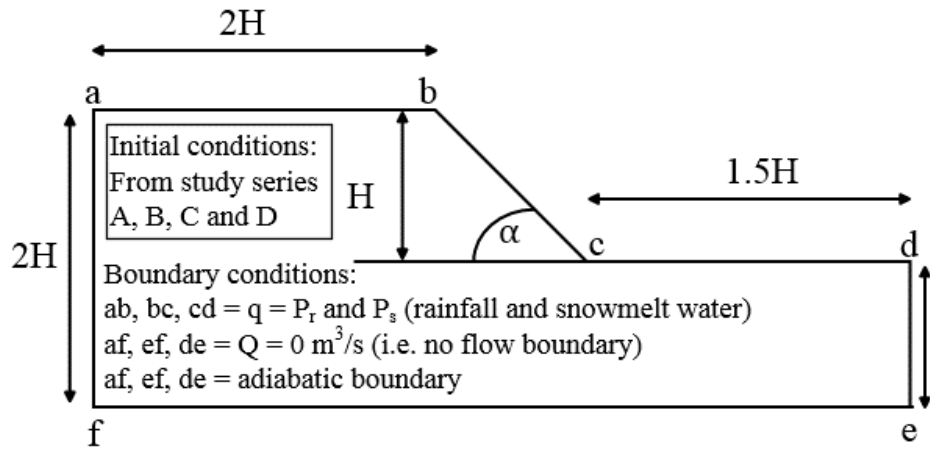
Figure 12 Slope geometry and boundary conditions for homogeneous soil slope used in parametric studies
