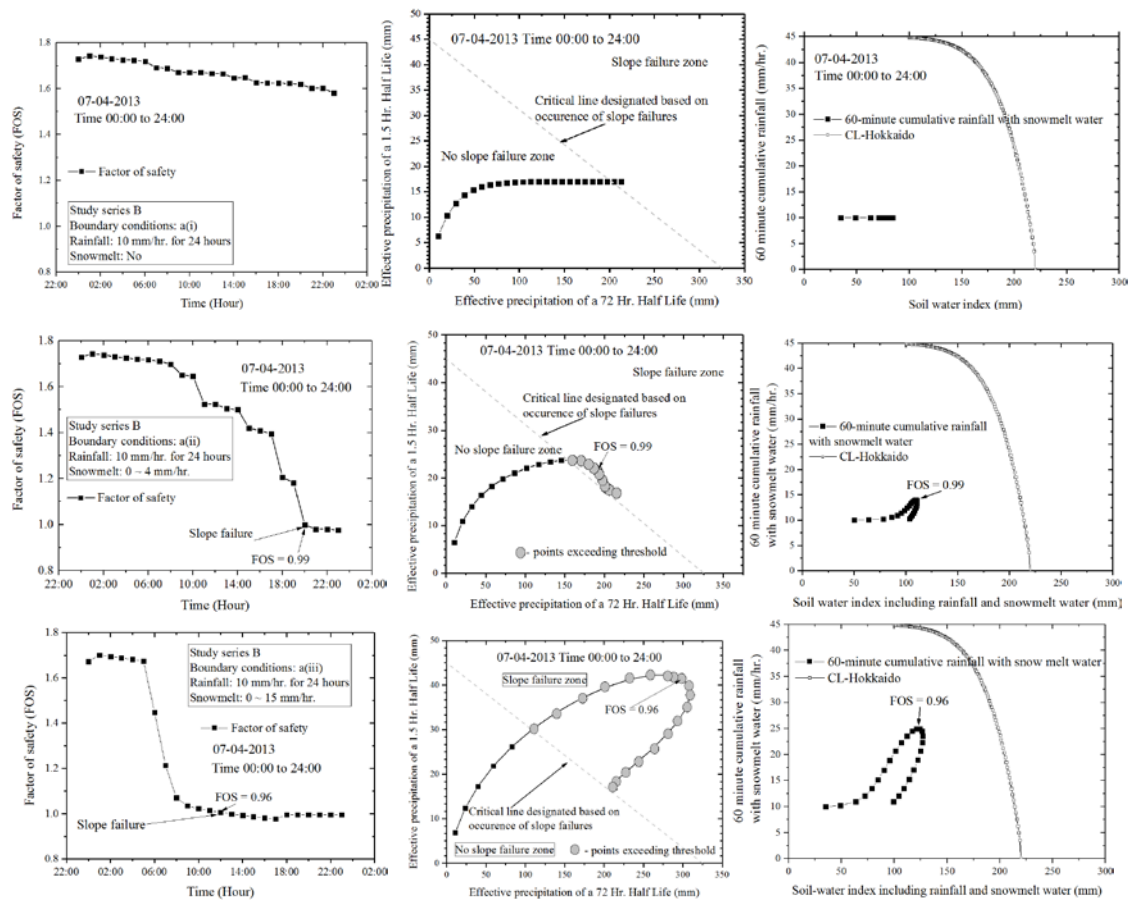
Figure 17 Factor of safety, Effective Precipitation index and Soil Water Index for study series B
