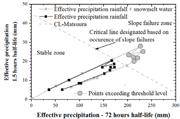
Figure 15 Possible revisions of the Effective rainfall index with snowmelt water/ Effective precipitation index
