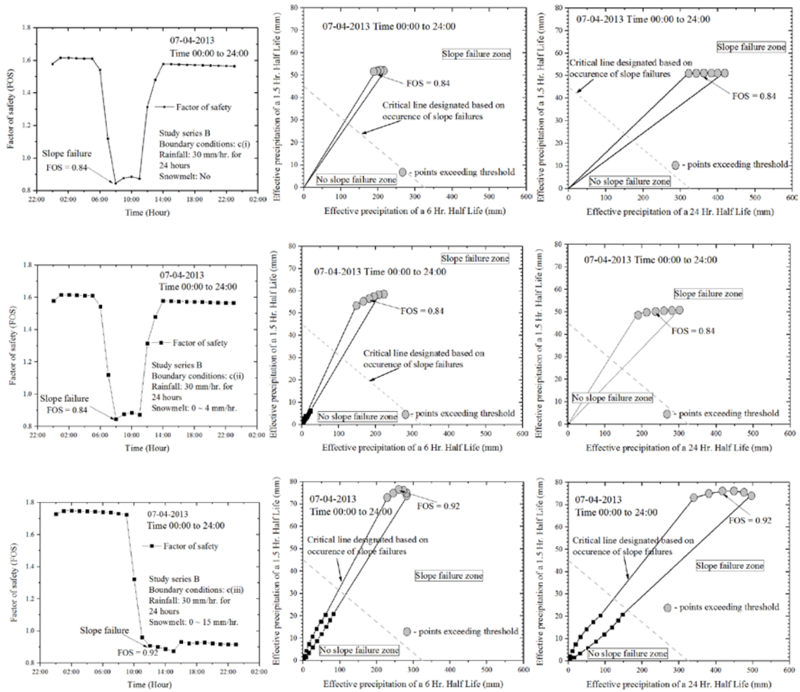
Figure 20 Comparison of Factor of safety, Effective Precipitation index 6 hours half-life and 24 hours half-life for study series B with 45° slope angle, 5 m slope height, 30 mm/hr. rainfall with two different snowmelt rates
