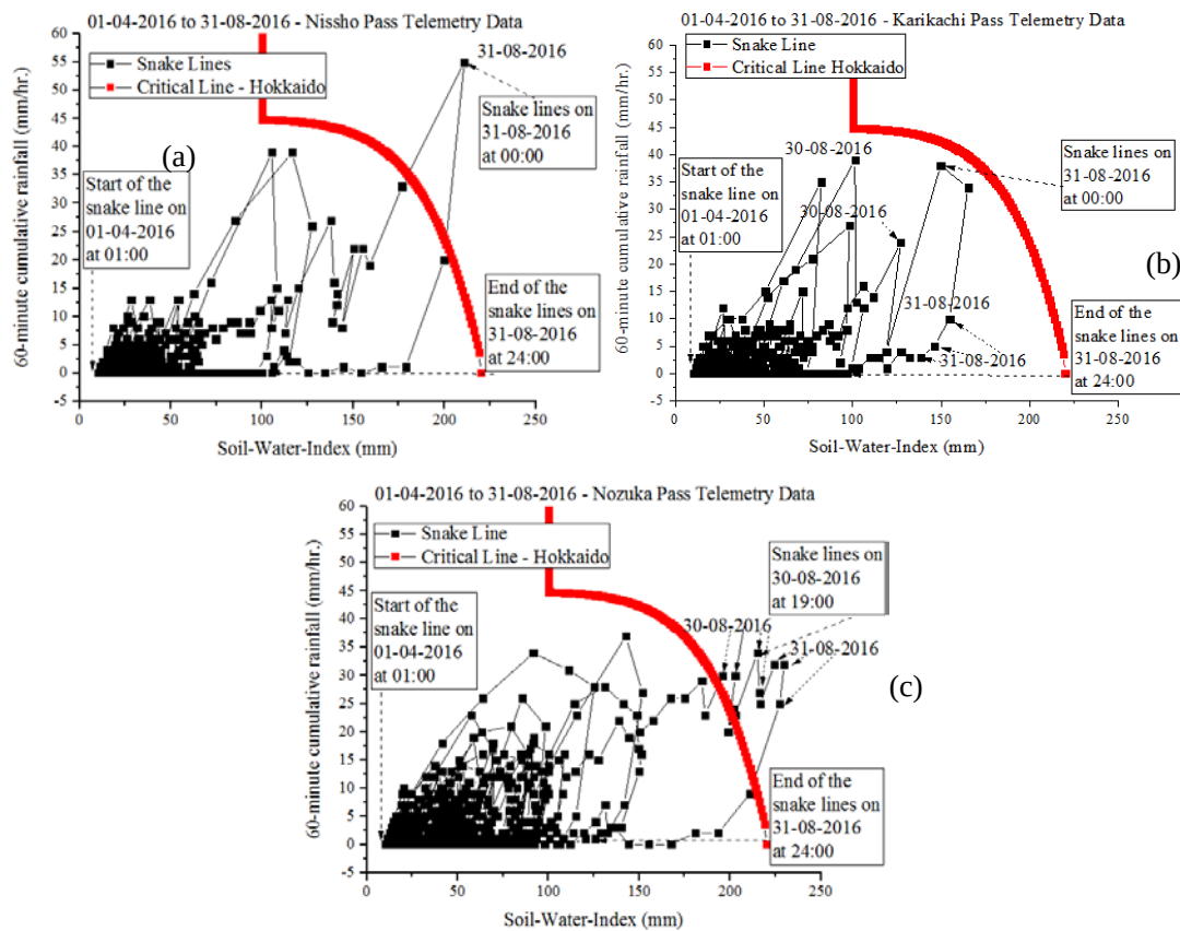
Figure 7 60-minute cumulative rainfall and Soil Water Index relationships (SWI) for data collected from (a) Nissho pass, (b) Karikachi pass and (c) Nozuka pass telemetries
