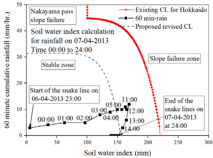
Figure 6 60-minute cumulative rainfall and Soil Water Index relationships (SWI) for Slope failure on April 2013 along National Highway Route 230
