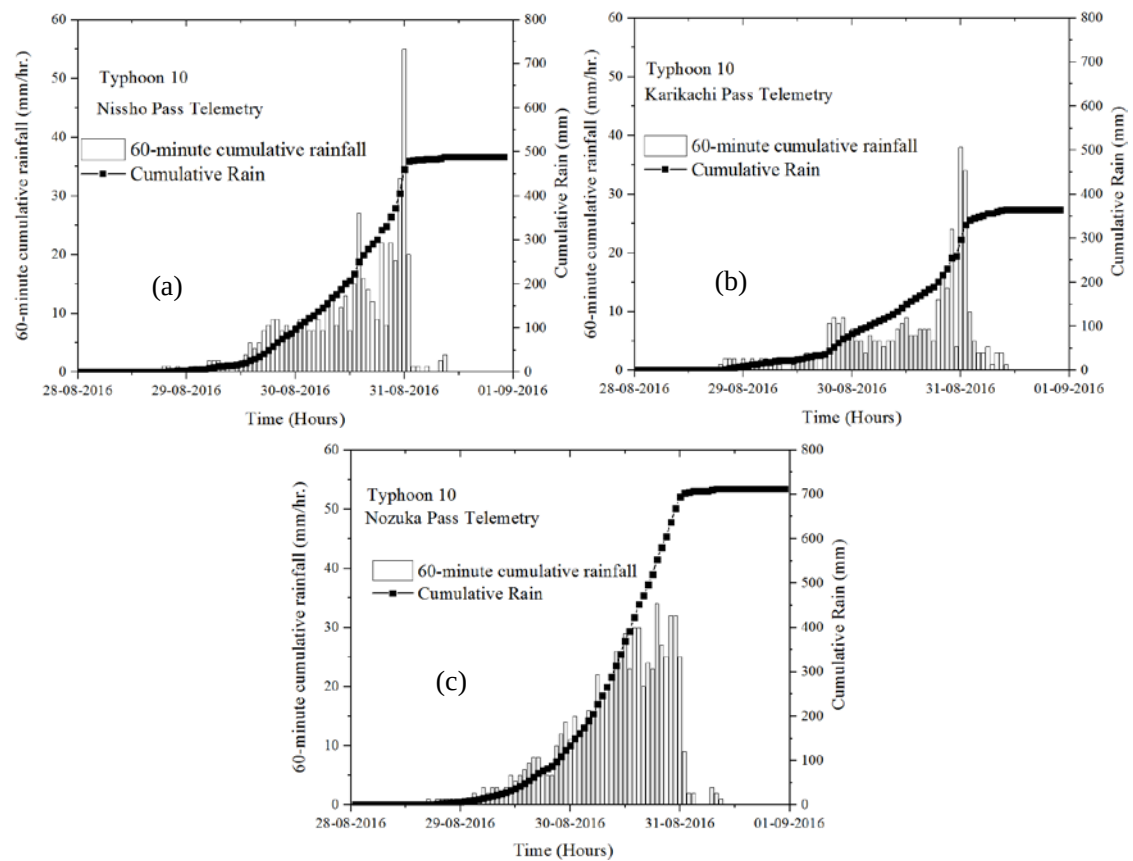
Figure 3 Rainfall recorded during typhoon at (a) Nissho pass meteorological telemetry (b) Karikachi pass meteorological telemetry and (c) Nozuka pass meteorological telemetry
