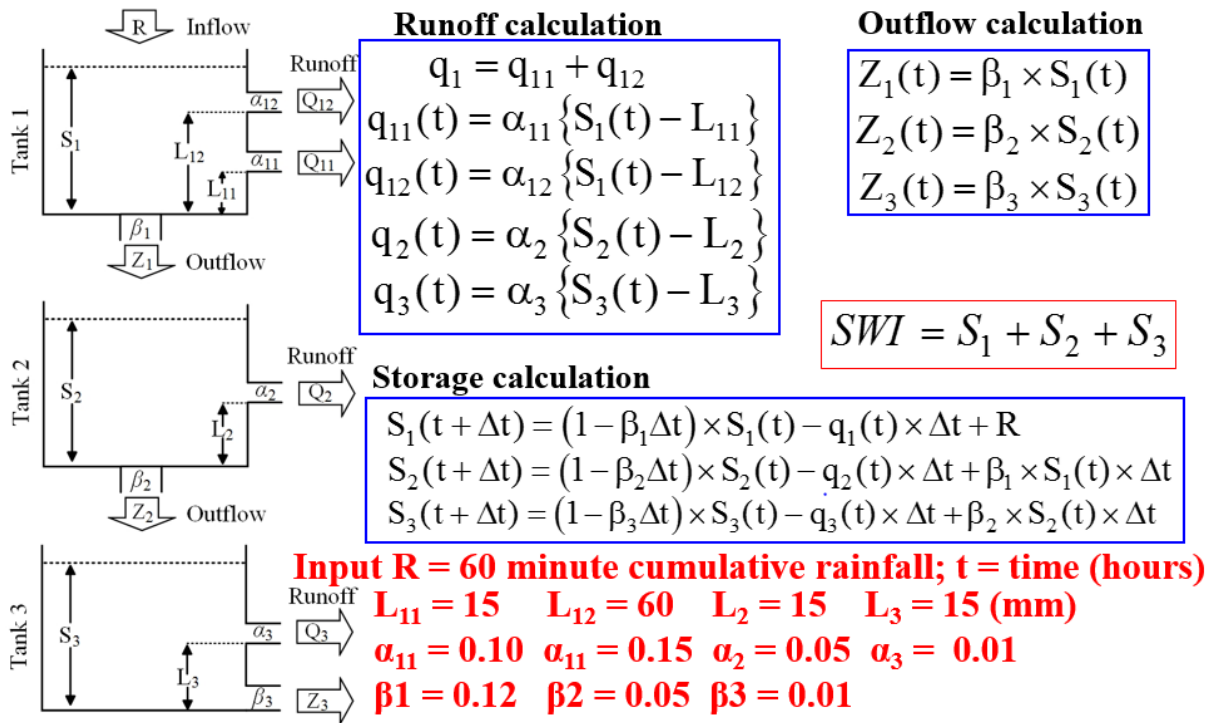
Figure 4 Three-layer tank model for Soil Water Index (adapted from Okada, 2001)
