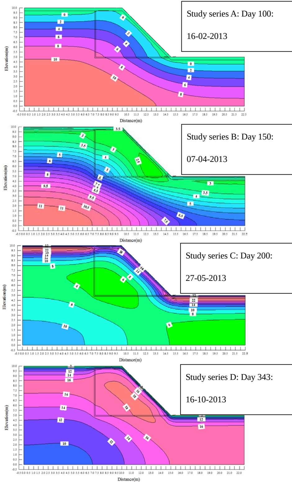
Figure 14 Initial temperature (°C) distributions during four different seasons
