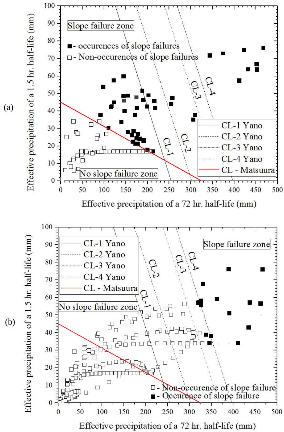
Figure 21 Plots of all slope failures and stable cases using Effective Precipitation index with half-lives 1.5 hours and 72 hours (a) series B and C, (b) series A and D.
