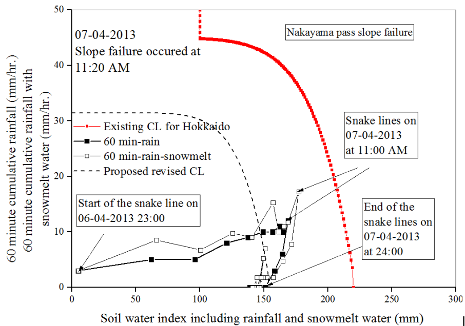
Figure 16 Prediction of Nakayama pass slope failure with consideration of snowmelt water using SWI
