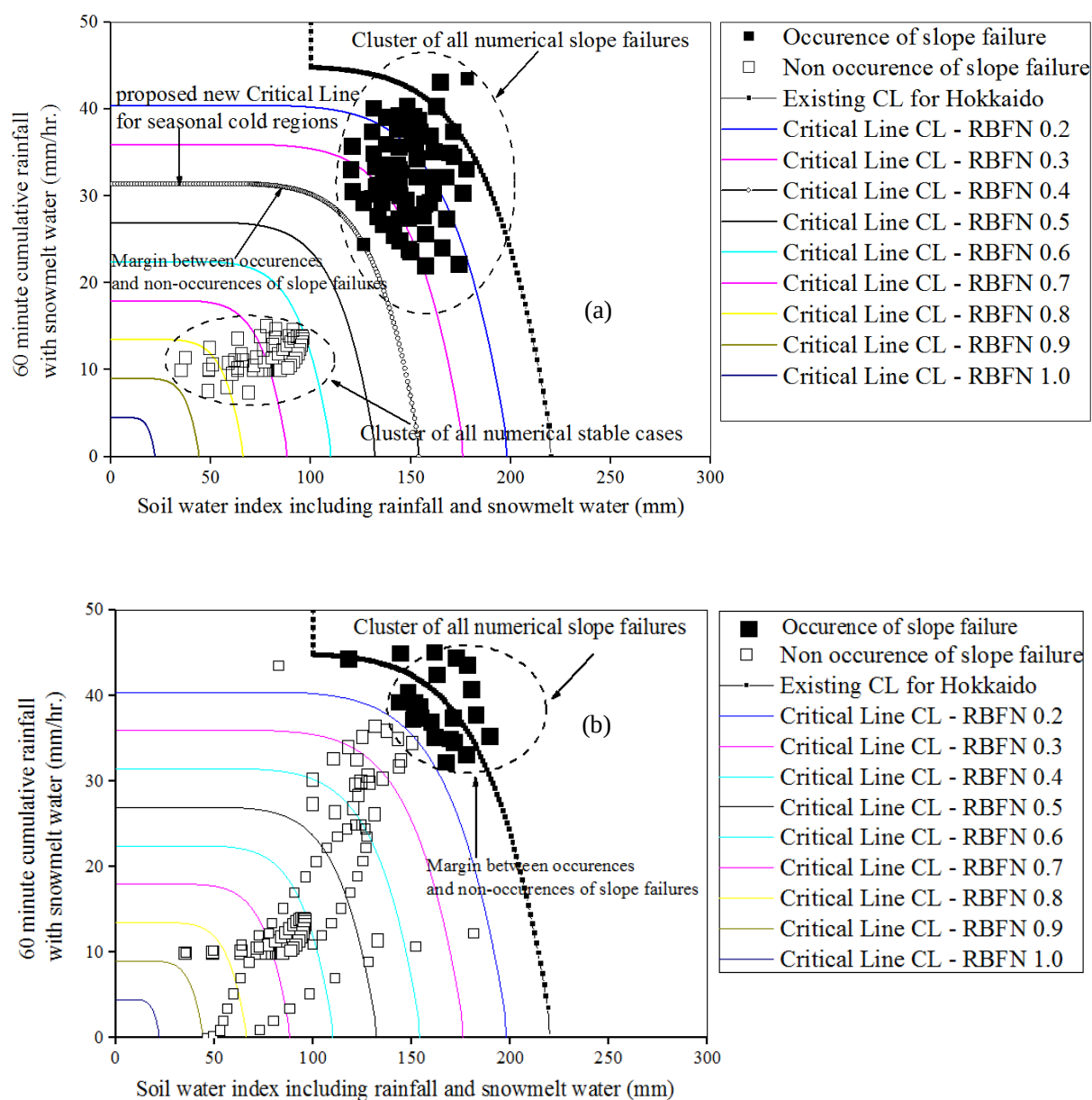
Figure 23 Possible revisions of the Critical Line designated for Hokkaido
