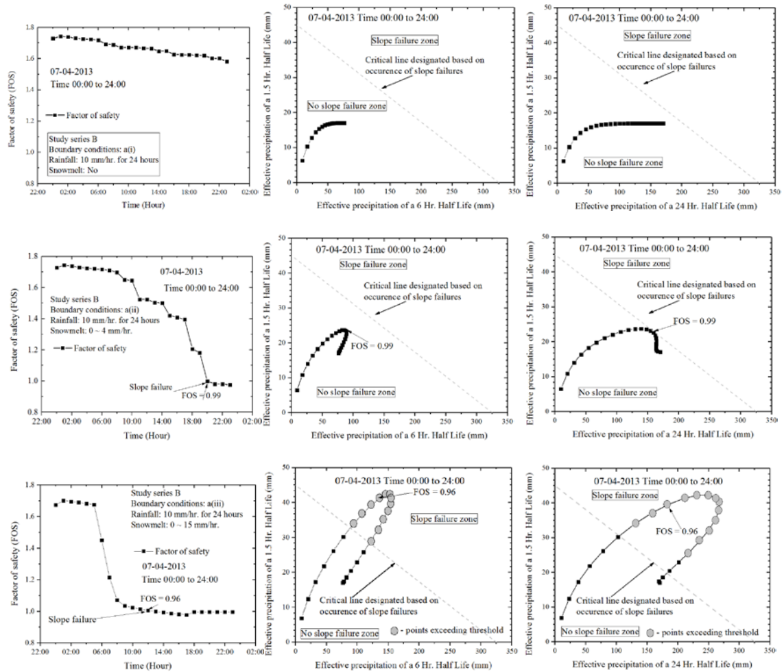
Figure 19 Comparison of Factor of safety, Effective Precipitation index 6 hours half-life and 24 hours half-life for study series B with 45° slope angle, 5 m slope height, 10 mm/hr. rainfall with two different snowmelt rates
