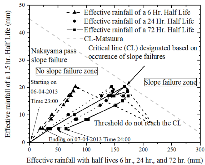
Figure 8 Plot of Effective rainfall index with half-life 1.5 hours (y axis) and half-lives 6 Hours, 24 Hours and 72 hours in (x axis) for the case of Nakayama pass slope failure.
