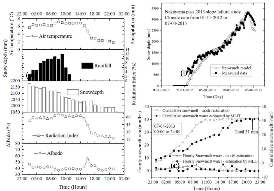
Figure 11 Estimation of snowmelt water using snowmelt model (a) climate data for Nakayama pass slope failure on 07-04-2013, (b) comparison of estimated and measured change in snow depth and (c) comparison of estimated snowmelt water on 07-04-2013.
