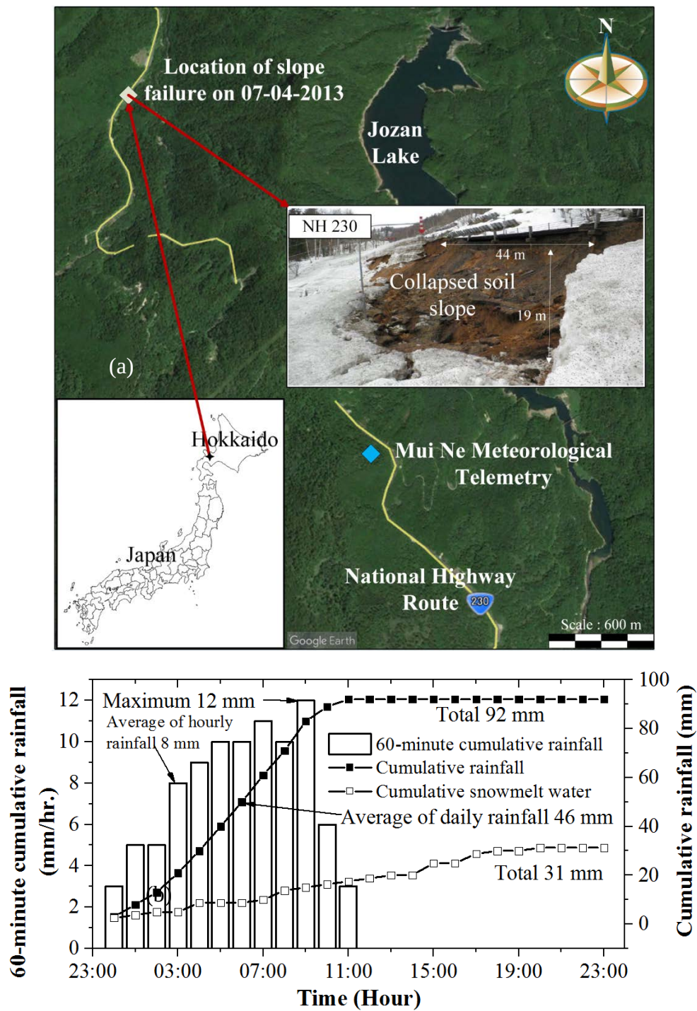
Figure. 1 (a) Locations of slope failure and meteorological telemetry along National Highway Route 230 and panoramic view of the slope failure (adapted from Hokkaido regional development bureau, 2014) and (b) Rainfall and snowmelt recorded on 07-04-2013 at Mui Ne meteorological telemetry
