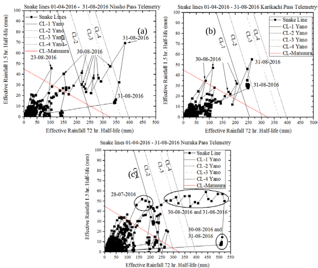
Figure 9 Snake lines plotted for the data recorded from (a) Nissho Pass, (b) Karikachi Pass and (c) Nozuka Pass Telemetries
