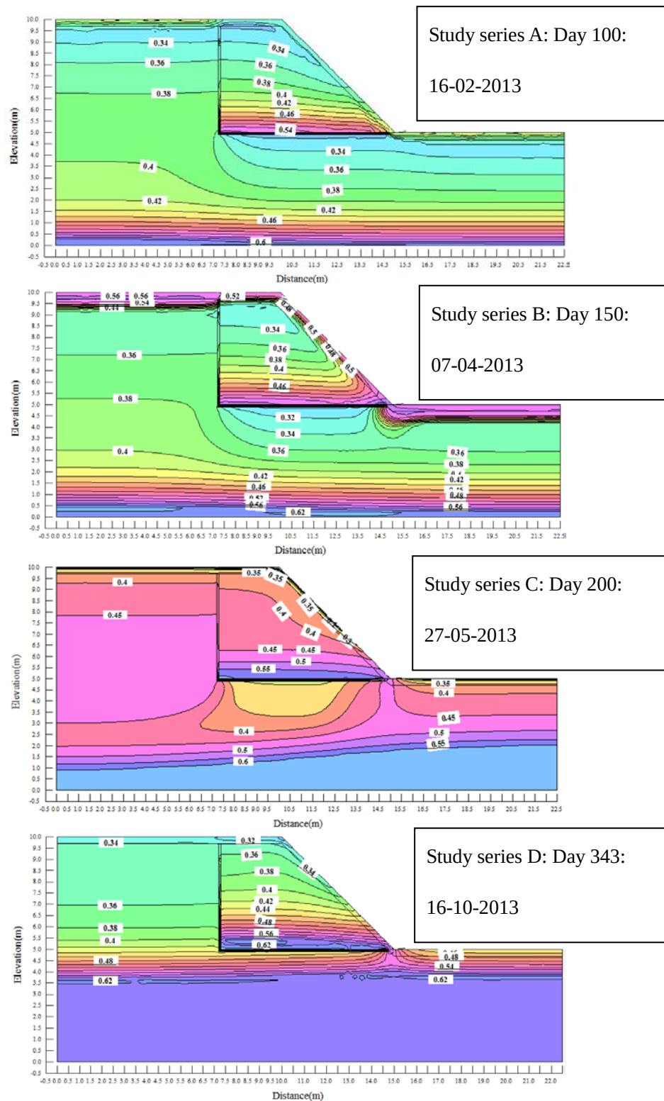
Figure 13 Initial volumetric water content ( \text{m}^3/\text{m}^3 ) distributions during four different seasons
