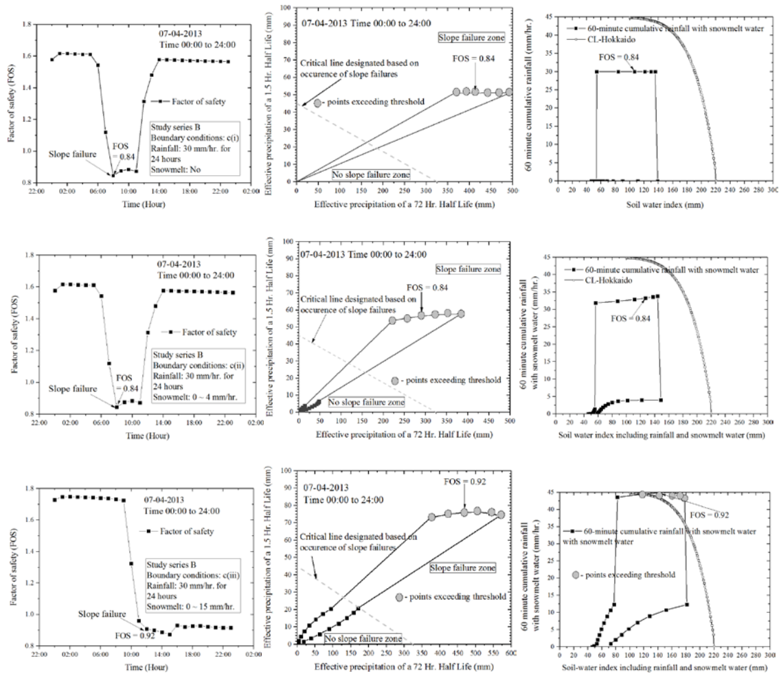
Figure 18 Factor of safety, Effective Precipitation index and Soil Water Index with 45° slope angle,
