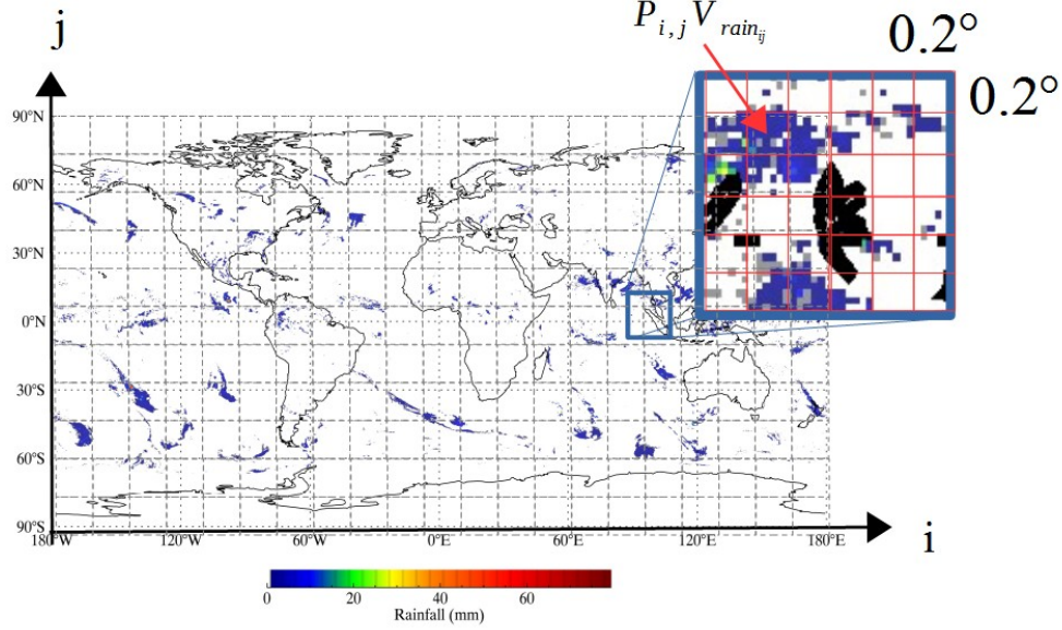
Figure 4.3: Example of the rainfall data provided by the GPM on June 4, 2014, which was used to calculate the upward electric current to the ionosphere.
