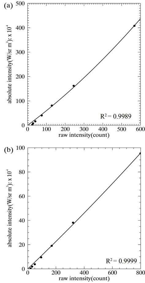
Fig. B1. The variation of the absolute and relative intensities for (a) LSI-1 and (b) LSI-2.
