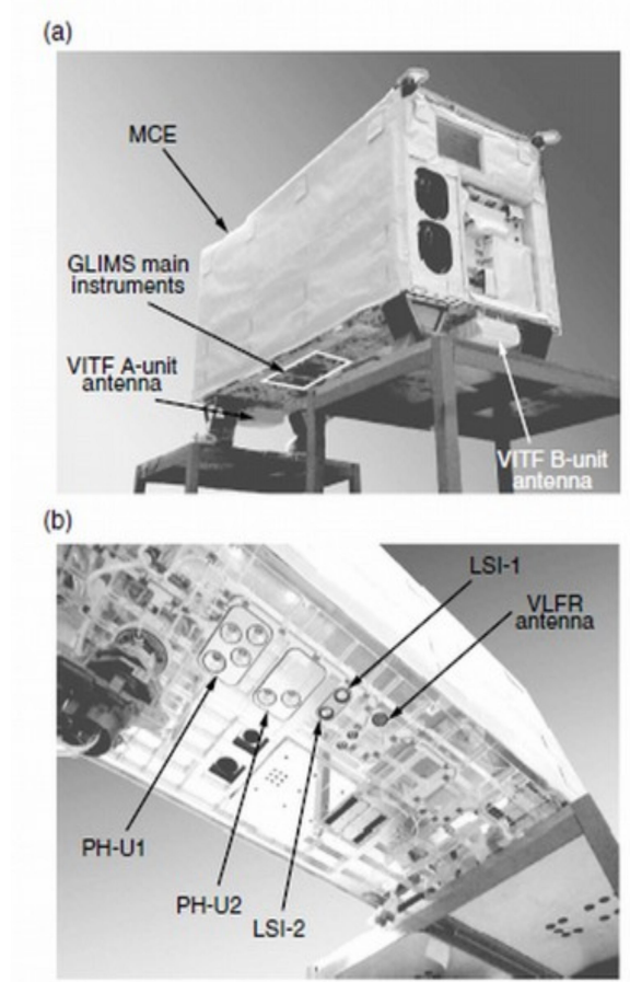
Figure 2.1: JEM-GLIMS optical instruments (PHs and LSI) and electromagnetic waves receiver (VLFR) (Sato, 2015).
