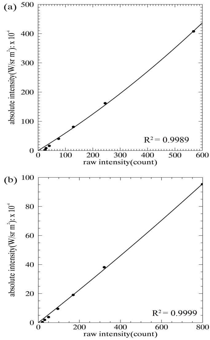
Figure A.2: The variation of the absolute and relative intensities for (a) LSI-1 and (b) LSI-2) Bandholnopparat et al. (2019).
