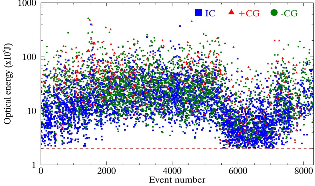
Figure B.1: Optical energy distribution of lightning events detected by JEM-GLIMS optical instruments in the wavelength range of 400 - 1000 nm.
