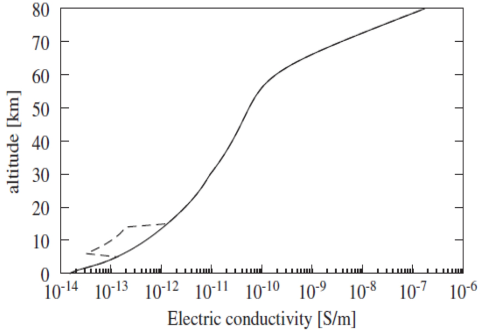
Figure 1.6: Electric conductivity profile of the air ( \sigma(z) ) for calculating the values of resistance in the global electric circuit (Rycroft et al., 2007).
