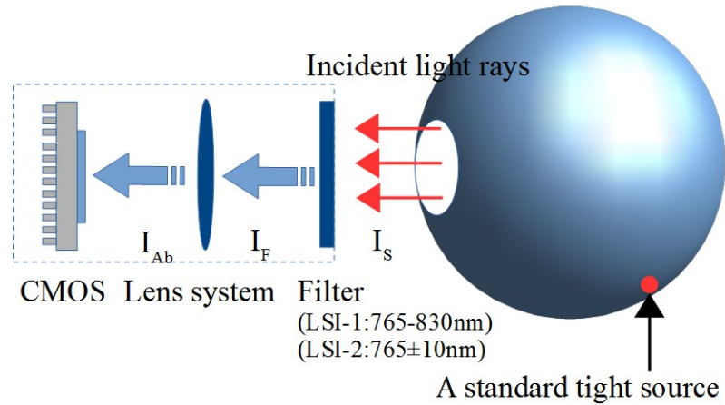
Figure A.1: Schimetic diagram for calibrating the LSI-1 and LSI-2 cameras.
