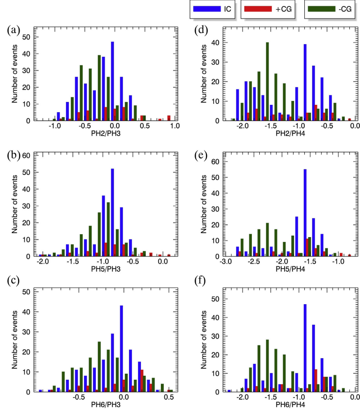
Fig. 6. Histograms of the logarithmic PH intensity ratio. The blue, red and green bars show the ratio of PH2/PH3, PH5/PH3, PH6/PH3, PH2/PH4, PH5/PH4, PH6/PH4 of IC, +CG, and -CG discharges, respectively.
