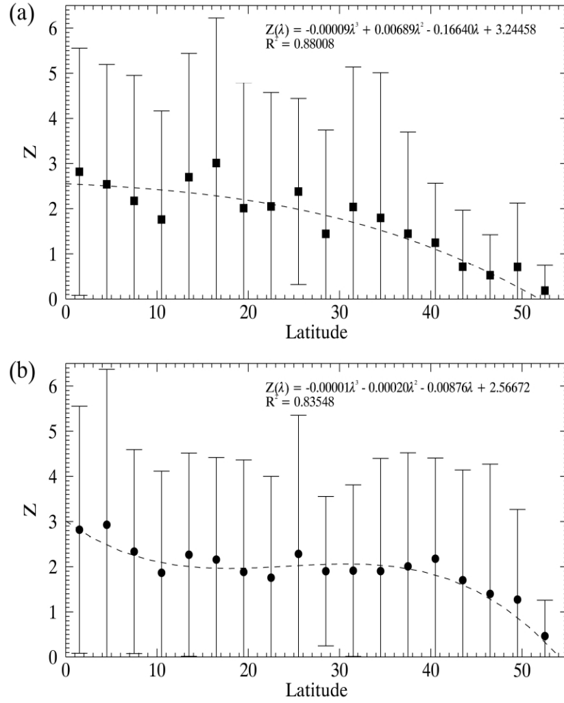
Figure 3.14: Latitudinal dependences of the Z-ratio in the northern hemisphere. (b) Same as (a) except for the southern hemisphere. In these figures, the zonal-mean Z-ratio values are calculated every 3^\circ latitudinal range and plotted. Vertical bars at each data point represent the \pm 1\sigma of Z-ratio values
