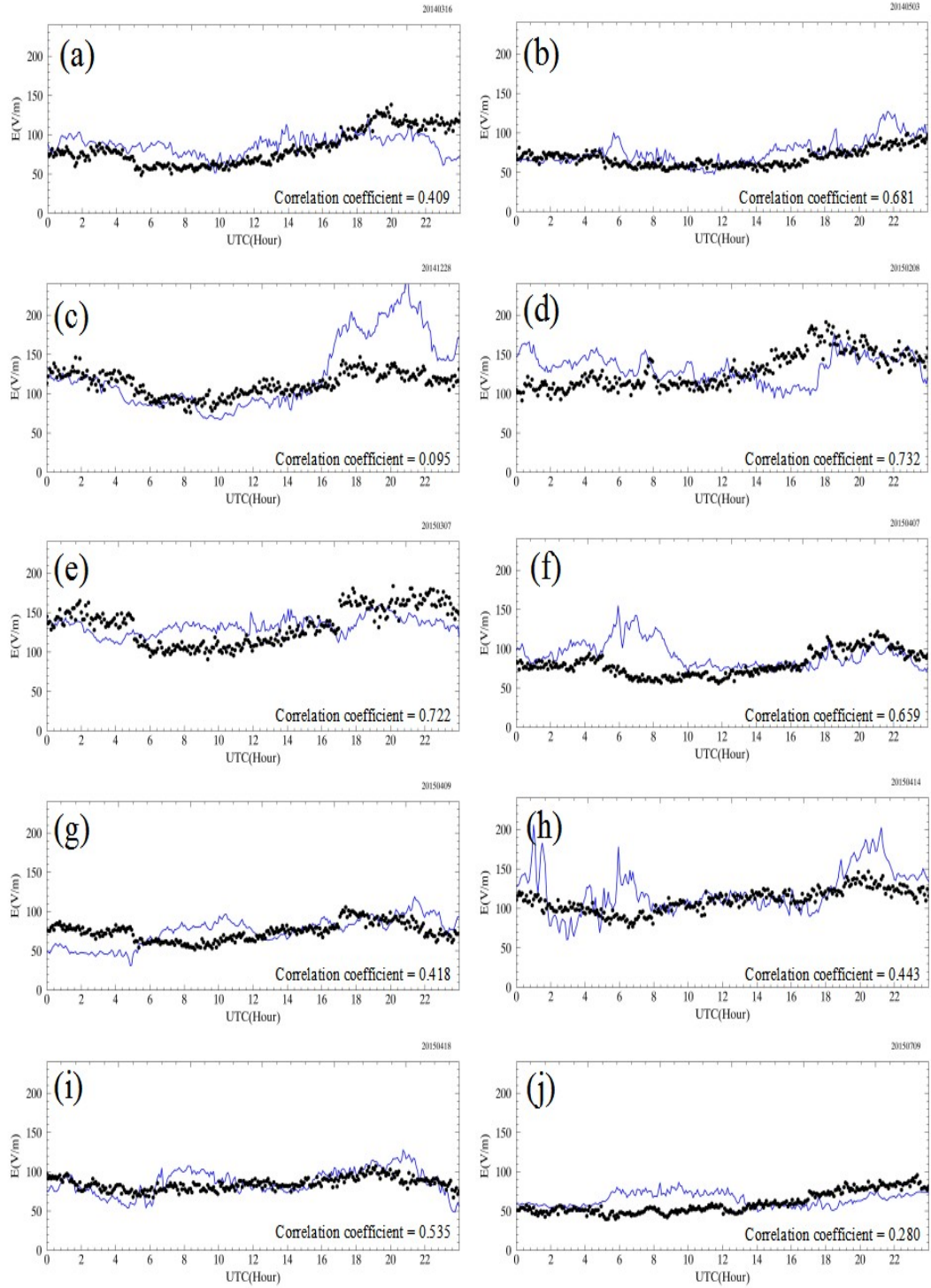
Figure 5.14: Comparison between the estimated fair-weather electric field (black dot) and observed fair-weather electric field (blue line) at the Reading Station, located in the United Kingdom.
