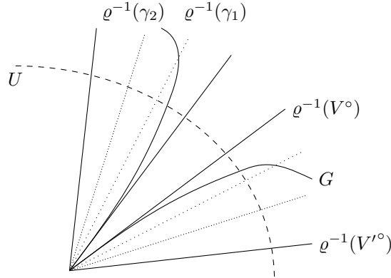
Figure 3: Geometrical relations in X \times X
