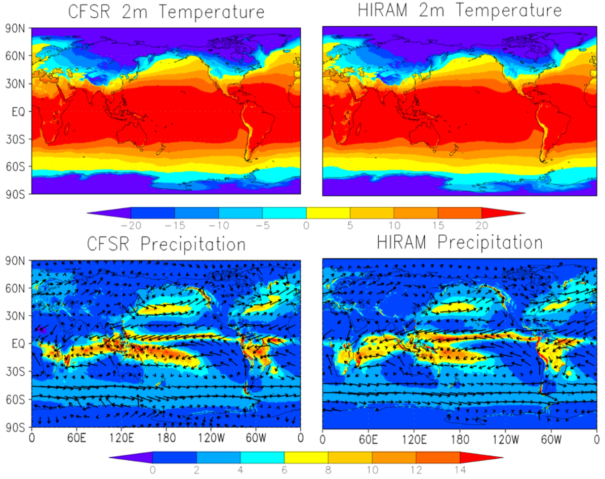
Figure 3.1: Mean pattern of 2m surface air temperature (°C in top) and precipitation (mm/day in bottom) in winter (DJF) season produced using CFSR (left panel) and HIRAM simulation (right panel) overlaid with mean wind vectors at 925 hPa.
