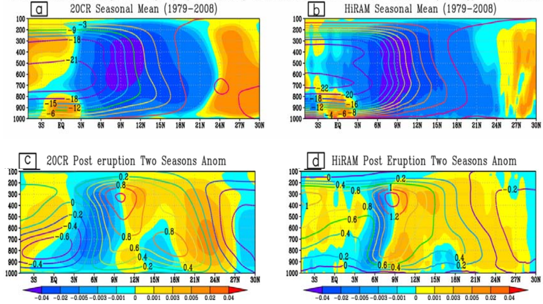
Figure 5.1: Zonal-mean omega (vertical velocity in shaded colors; Pa/s) and zonal-mean meridional mass stream function (in contours; 10^8 kg/s) mean pattern (a, b) calculated using 1979-2008 period and post-eruption two summer season averaged anomaly pattern following both the El Chichón and Pinatubo eruptions (c, d) from 20th century NOAA reanalysis (left) and HiRAM model at 25 km (right panel). The positive (negative) shaded values in color bar represent the sinking (rising) branch of HC.
