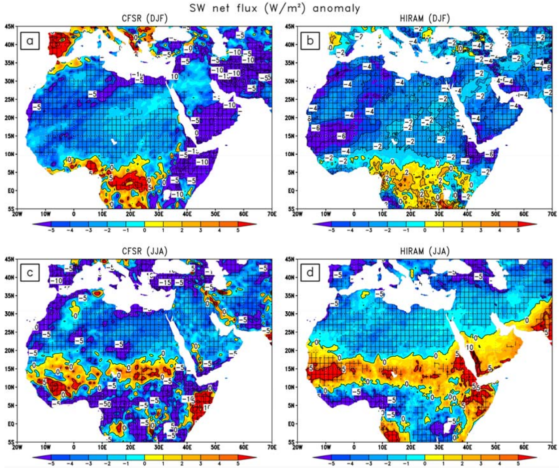
Figure 4.2: Seasonal (DJF and JJA) two-year anomalies of solar net flux ( \text{W/m}^2 ) composites following the El Chichón and Pinatubo explosive eruptions, calculated for winter using a) CFSR and b) HiRAM outputs, and for summer using c) CFSR and d) HiRAM outputs. Hatching shows the statistically significant areas with at least 95% confidence level examined by bootstrapping with replacement test.
