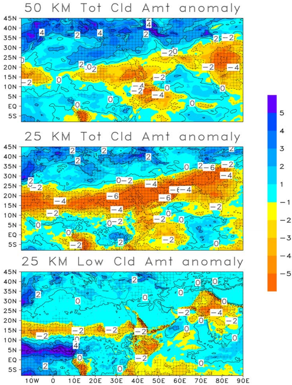
Figure 5.6: Total cloud contents anomaly (%) composite for post-eruption two summer seasons following El Chichón and Pinatubo eruptions using HiRAM at 50 km (top panel), at 25 km (middle panel) and low cloud contents anomaly using HiRAM at 25 km (bottom panel). Hatching shows the areas where the cloud contents anomaly is significant at 95% confidence level.
