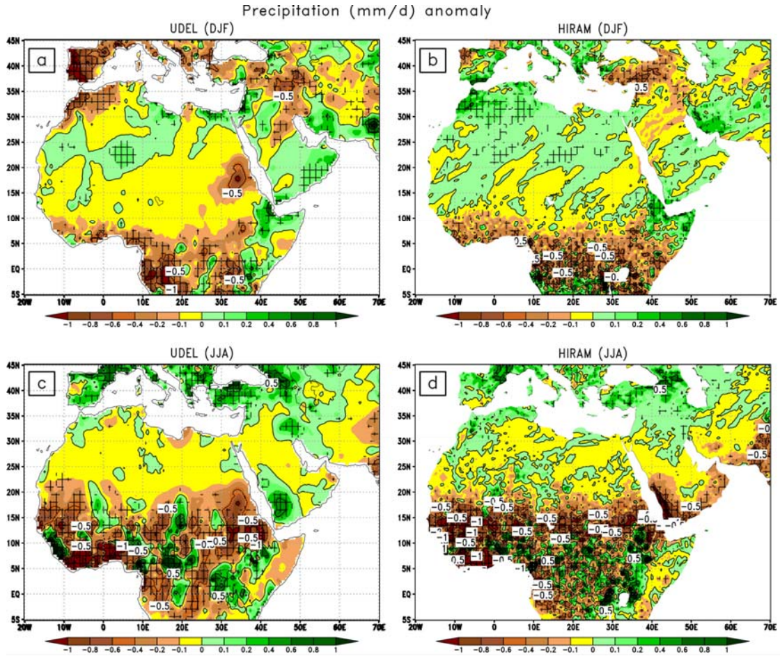
Figure 4.4: Same as Figure 4.3, but for precipitation anomaly (mm/day).
