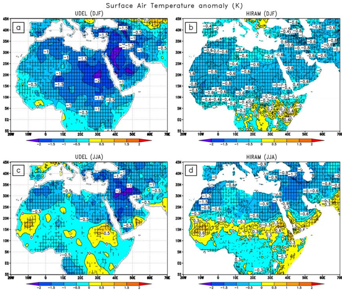
Figure 4.3: Seasonal (DJF and JJA) two-year anomalies of surface air temperature (K) composites following the El Chichón and Pinatubo explosive eruptions, calculated for winter using a) UDEL observations, b) HiRAM output, and for summer using c) UDEL observations, d) HiRAM output. Hatching shows the statistically significant areas with at least 95% confidence level examined by bootstrapping with replacement test.
