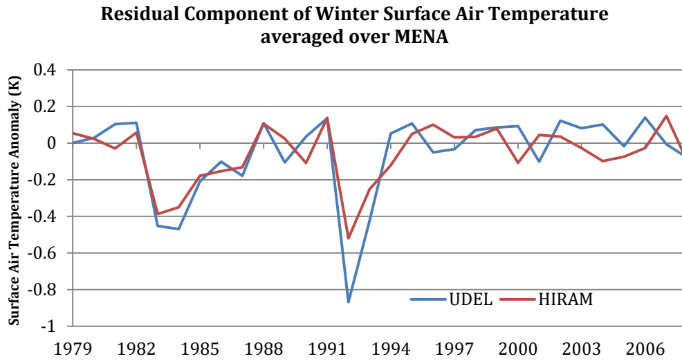
Figure 4.20: Time series of the residual component in winter (DJF) surface air temperature averaged over the MENA region (20°W-70°E, 5°S-45°N).
