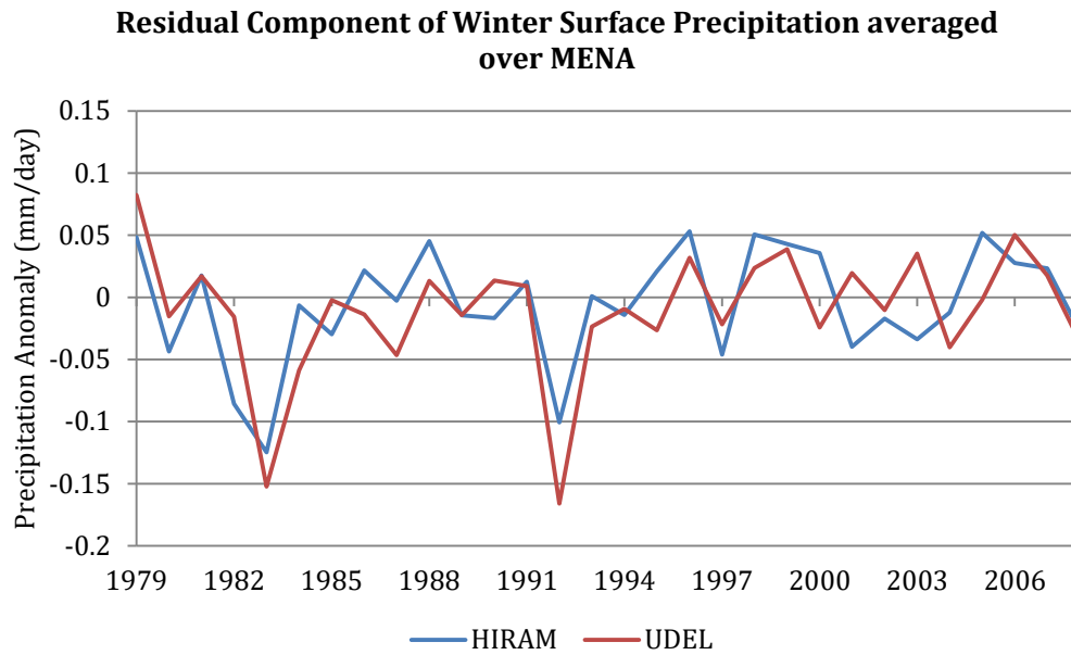
Figure 4.21: Time series of the residual component in winter (DJF) surface precipitation averaged over the MENA region (20°W-70°E, 5°S-45°N).
