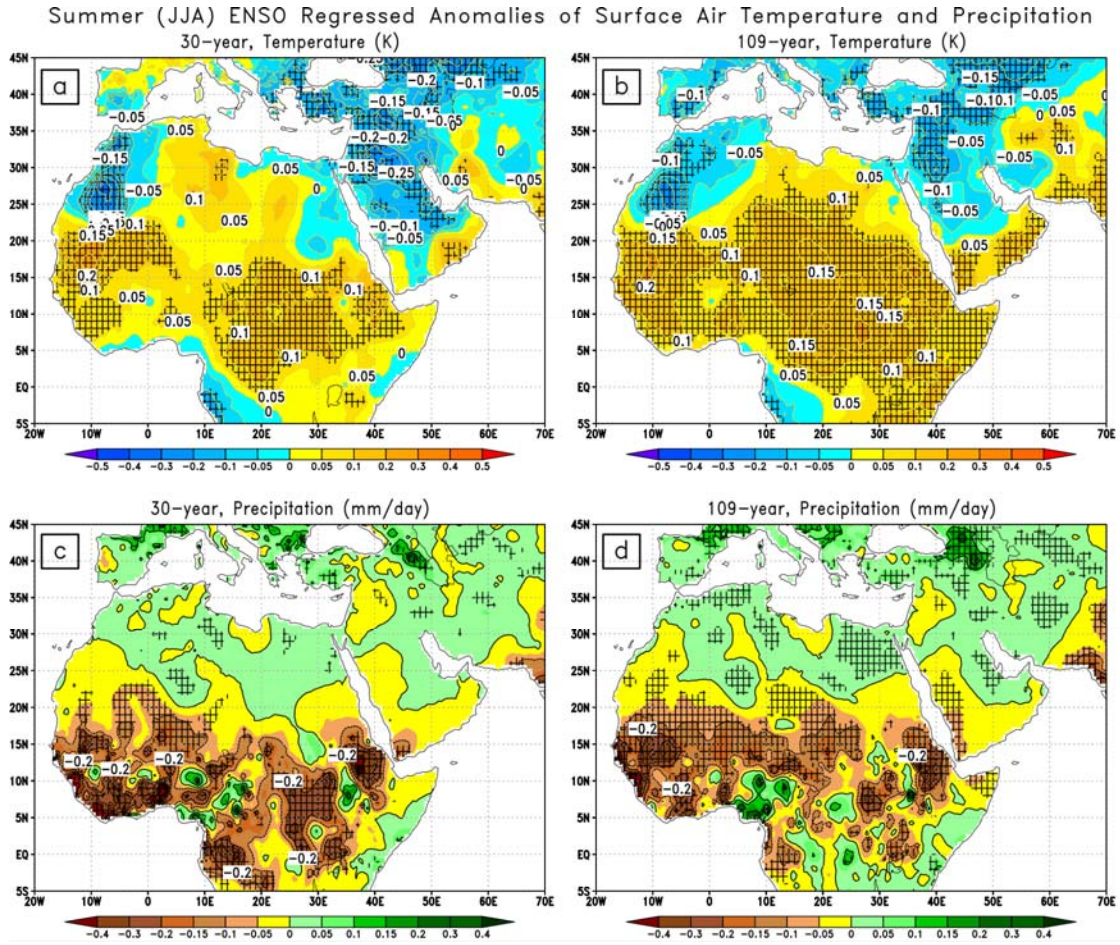
Figure 4.14: Anomalies of ENSO-regressed surface air-temperature (K) and precipitation (mm/day) composited for two summer (JJA) seasons following both the El Chichón and Pinatubo eruptions. The temperature composites are calculated using a) UDEL 30-year period, b) UDEL 109-year period, and precipitation composites using c) UDEL 30-year period, d) UDEL 109-year period. Hatching shows the statistically significant areas with at least 95% confidence level examined by bootstrapping with replacement test.
