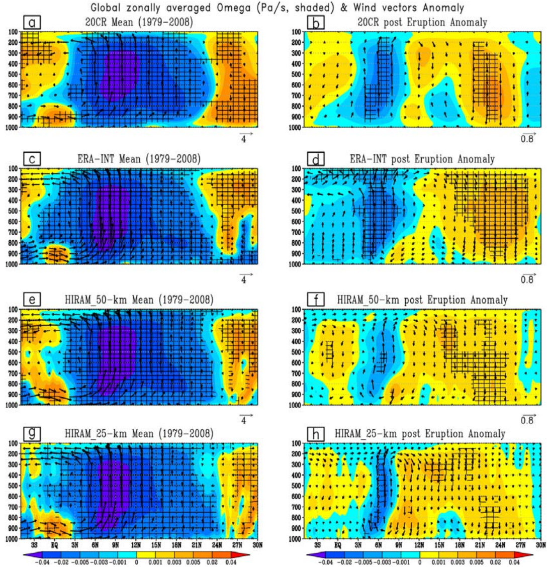
Figure 5.2: Mean (left panel) and anomaly (right panel) of zonal-mean Omega (vertical velocity in shaded colors; Pa/s) with overlaid zonal-mean wind vectors ( v ; -100 \times \Omega ) [m/s; 100 \times \text{Pa/s} ] in the latitude-pressure plane. The mean pattern (calculated using the 1979–2008 period) is shown using a) 20CR, c) ERA-Interim, e) HiRAM at 50 km and g) HiRAM at 25 km and the post-eruption (following both the El Chichón and Pinatubo) two summer seasons averaged anomaly pattern is shown using b) 20CR, d) ERA-Interim, f) HiRAM at 50 km and h) HiRAM at 25 km. Positive shaded values in color bar represent sinking motion whereas negative values represent the rising branch of HC. Hatching shows the areas where the mean and anomaly pattern is significant at 95% confidence interval.
