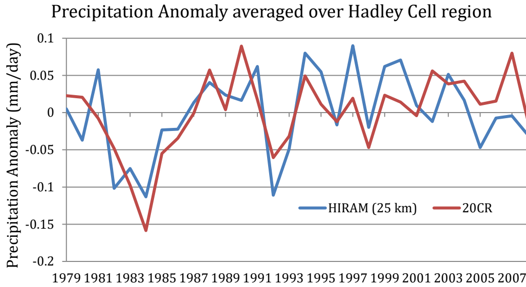
Figure 5.7: Summer (JJA) precipitation anomaly (mm/d), after removing ENSO contribution through simple linear regression using Nino3.4 index as input predictor, averaged over the Hadley Cell region (0-360° E, 3°S-35° N).
