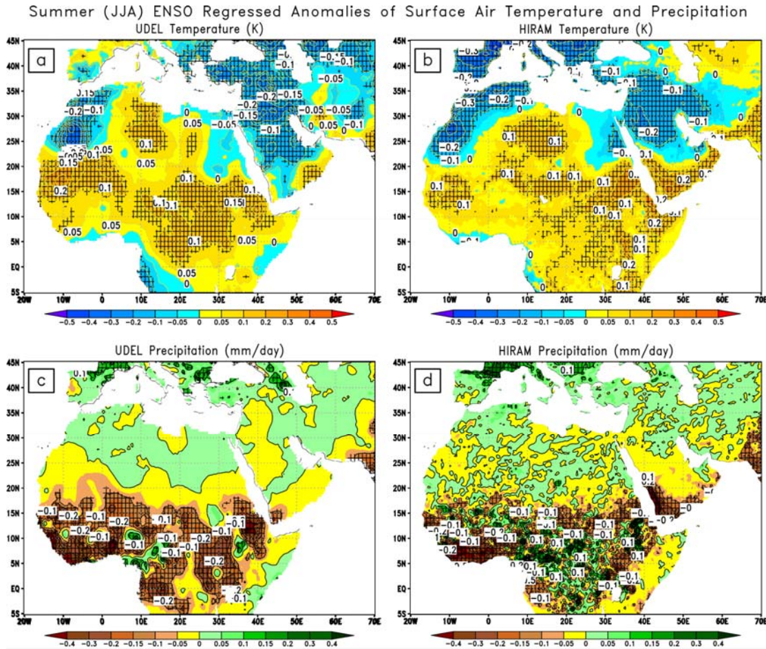
Figure 4.9: Anomalies of ENSO-regressed surface air temperature (K) and precipitation (mm/day) composited over two summer (JJA) seasons after both the El Chichón and Pinatubo eruptions. The temperature composites are calculated using a) UDEL observations, b) HiRAM output, and precipitation composites using c) UDEL observations, d) HiRAM output. Hatching shows the statistically significant areas with at least 95% confidence level examined by bootstrapping with replacement test.
