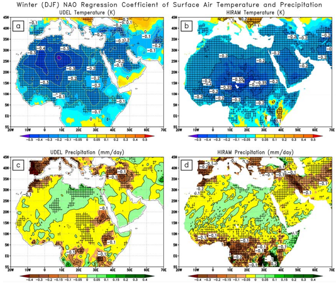
Figure 3.7: Winter (DJF) NAO regression coefficient with surface air-temperature (K) calculated using a) UDEL 30-year period, b) Model 30-year period, and with precipitation (mm/day) calculated using c) UDEL 30-year period, d) model 30-year period. Hatching shows the statistically significant areas with at least 95% confidence level.
