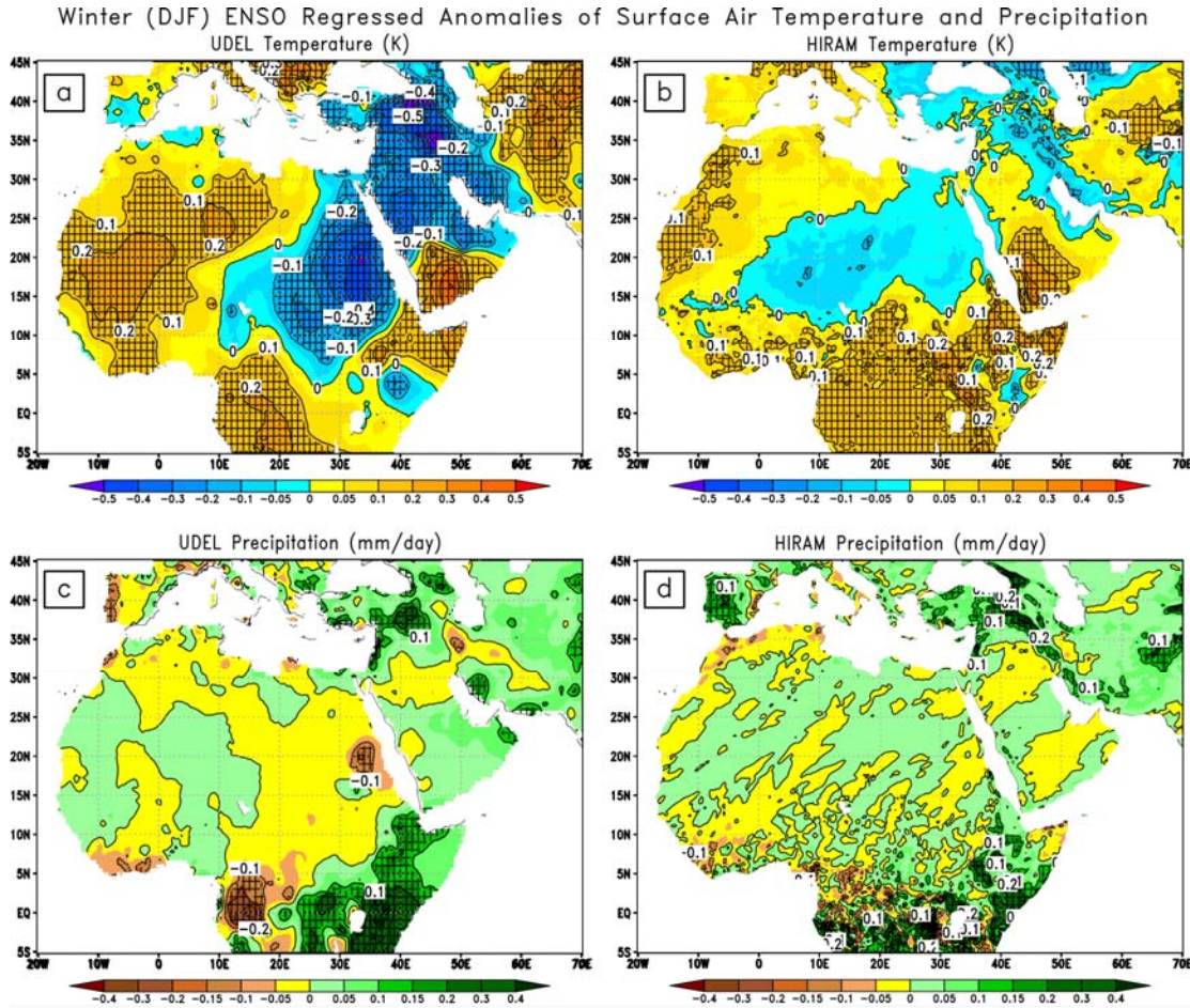
Figure 4.6: Anomalies of ENSO-regressed surface air temperature (K) and precipitation (mm/day) composited over two winter (DJF) seasons after both the El Chichón and Pinatubo eruptions. The temperature composites are calculated using a) UDEL observations, b) HiRAM output, and precipitation composites using c) UDEL observations, d) HiRAM output. Hatching shows the statistically significant areas with at least 95% confidence level examined by bootstrapping with replacement test.
