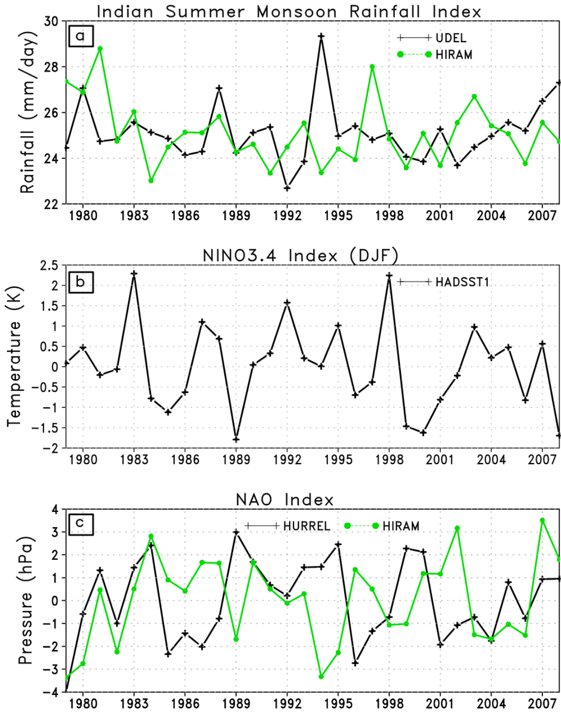
Figure 3.2: Time series of predictors (not standardized) from the observations and HiRAM used in the regression analysis in both seasons a) Indian Monsoon Rainfall Index, which shows the total summer rainfall computed over the entire Indian region b) NINO3.4/DJF, c) NAO Index of Hurrell (1995).
