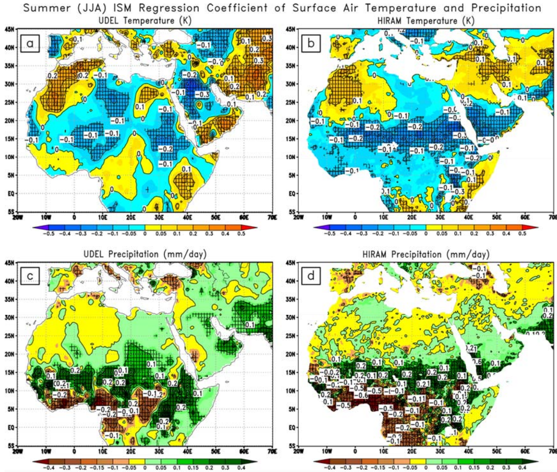
Figure 3.10: Summer (JJA) ISM regression coefficient of surface air-temperature (K) calculated using a) UDEL 30-year period, b) Model 30-year period, and with precipitation (mm/day) calculated using c) UDEL 30-year period, d) model 30-year period. Hatching shows the statistically significant areas with at least 95% confidence level.
