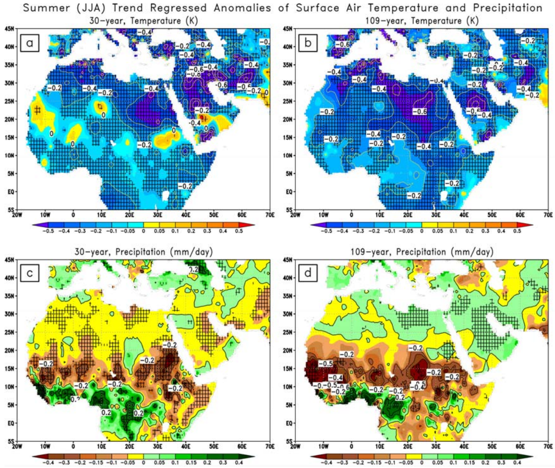
Figure 4.17: Anomalies of trend-component-regressed surface air-temperature (K) and precipitation (mm/day) composited for two summer (JJA) seasons following both the El Chichón and Pinatubo eruptions. The temperature composites are calculated using a) UDEL 30-year period, b) UDEL 109-year period, and precipitation composites using c) UDEL 30-year period, d) UDEL 109-year period. Hatching shows the statistically significant areas with at least 95% confidence level examined by bootstrapping with replacement test.
