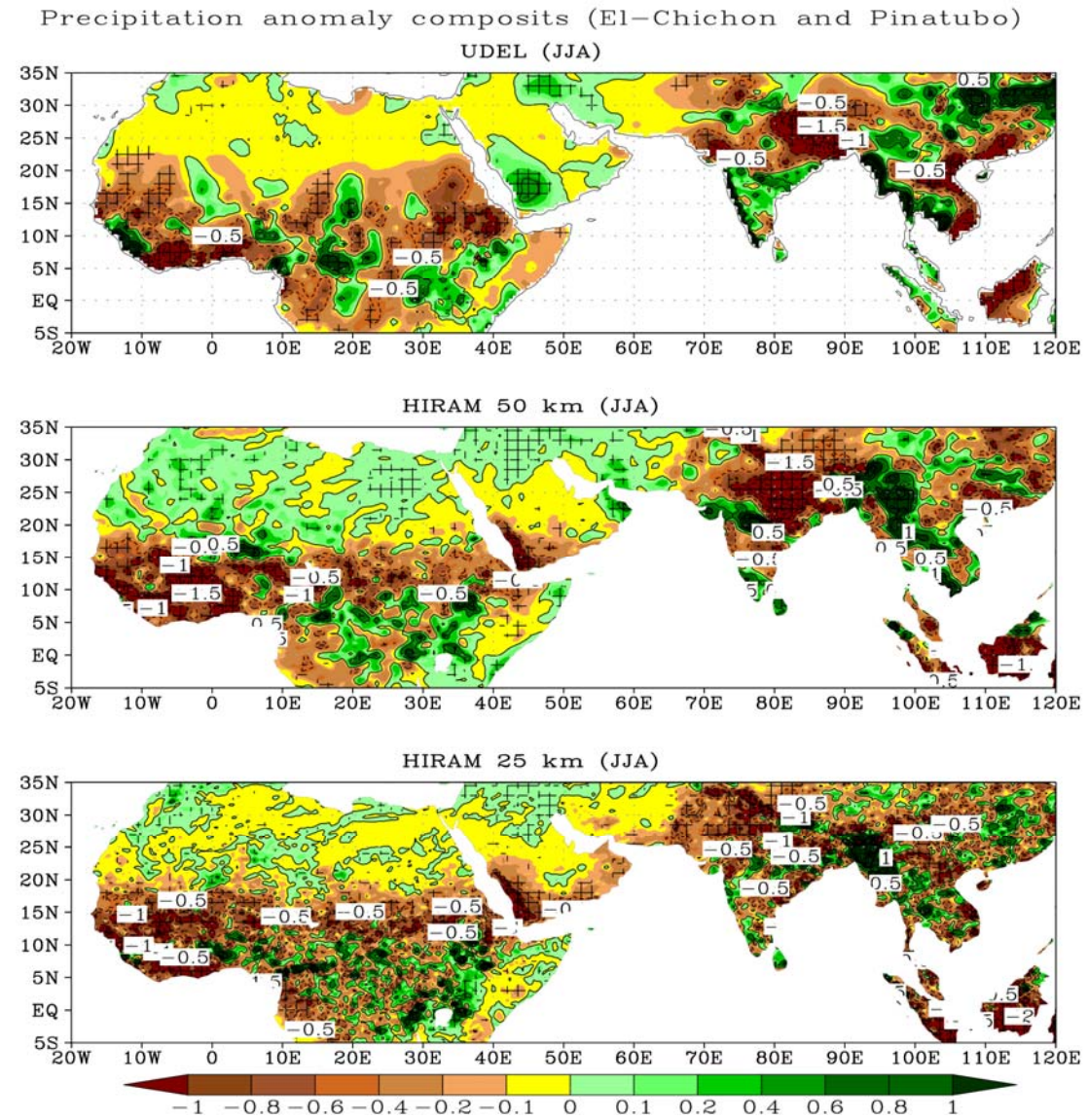
Figure 5.5: Composite precipitation anomaly (mm/d) for post-eruption (i.e., El Chichón and Pinatubo) two summer seasons using UDEL (top panel), HiRAM at 50 km (middle panel) and HiRAM at 25 km (bottom panel). Hatching shows the areas where the precipitation anomaly is significant at 95% confidence level.
