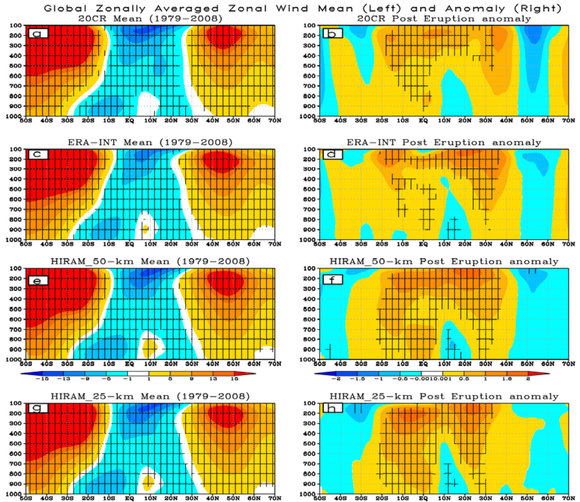
Figure 5.3: Global zonally averaged zonal wind (m/s) mean pattern using a) 20CR, c) ERA-Interim, e) HiRAM at 50 km, and g) HiRAM at 25 km and anomaly response (averaged for two summer seasons following both the eruptions) using b) 20CR, d) ERA-Interim, f) HiRAM at 50 km, and h) HiRAM at 25 km. Mean response is calculated using 1979-2008 period after excluding two summer seasons following both the eruptions and anomaly for both the eruptions is calculated using this mean. Hatching shows the areas where the mean and anomaly pattern is significant at 95% confidence interval.
