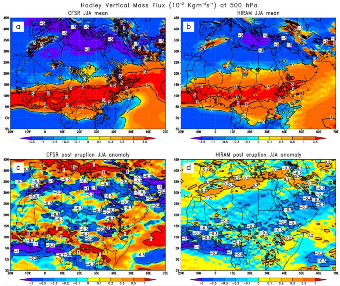
Figure 4.5: Summer (JJA) total vertical regional Hadley Cell mass flux M_\Phi (positive upward, 10^{-3} \text{ kg m}^{-2} \text{ s}^{-1} ) averaged over the period 1979-2008 (excluding post-eruption years) using a) CFSR, b) HiRAM outputs, and two-year composited anomalies of M_\Phi ( 10^{-3} \text{ kg m}^{-2} \text{ s}^{-1} ) following the El Chichón and Pinatubo eruptions calculated using c) CFSR, d) HiRAM outputs.
