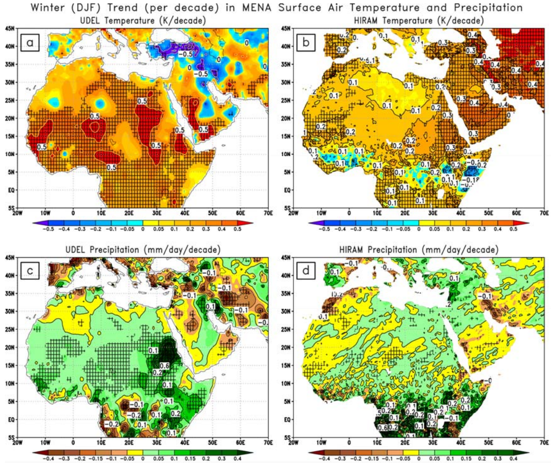
Figure 3.3: The spatial distributions of the trends (per decade) of winter (DJF) temperature over the period of 1979-2008 using (a) UDEL, (b) HiRAM output and trend in Precipitation using (c) UDEL and (d) HiRAM output. Hatching indicates statistically significant decadal trends at 95% confidence level that is computed using two-tailed student t-test.
