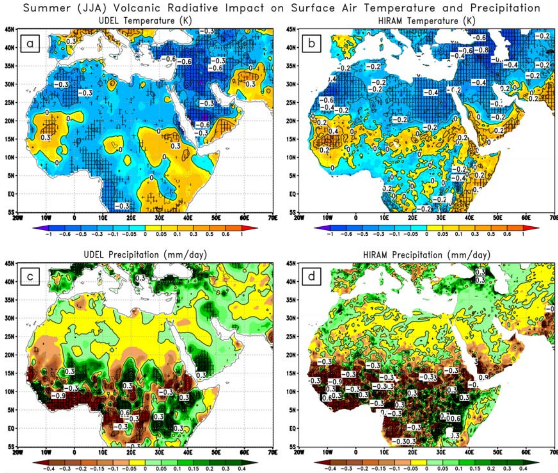
Figure 4.11: Summer (JJA) anomalies of surface air temperature (K) and precipitation (mm/day) regressed on the residual term (volcanic effect) composited for two winter seasons following both the El Chichón and Pinatubo eruptions. The temperature composites are calculated using a) UDEL observations, b) HiRAM output, and precipitation composites using c) UDEL observations, d) HiRAM output. Hatching shows the statistically significant areas with at least 95% confidence level examined by bootstrapping with replacement test.
