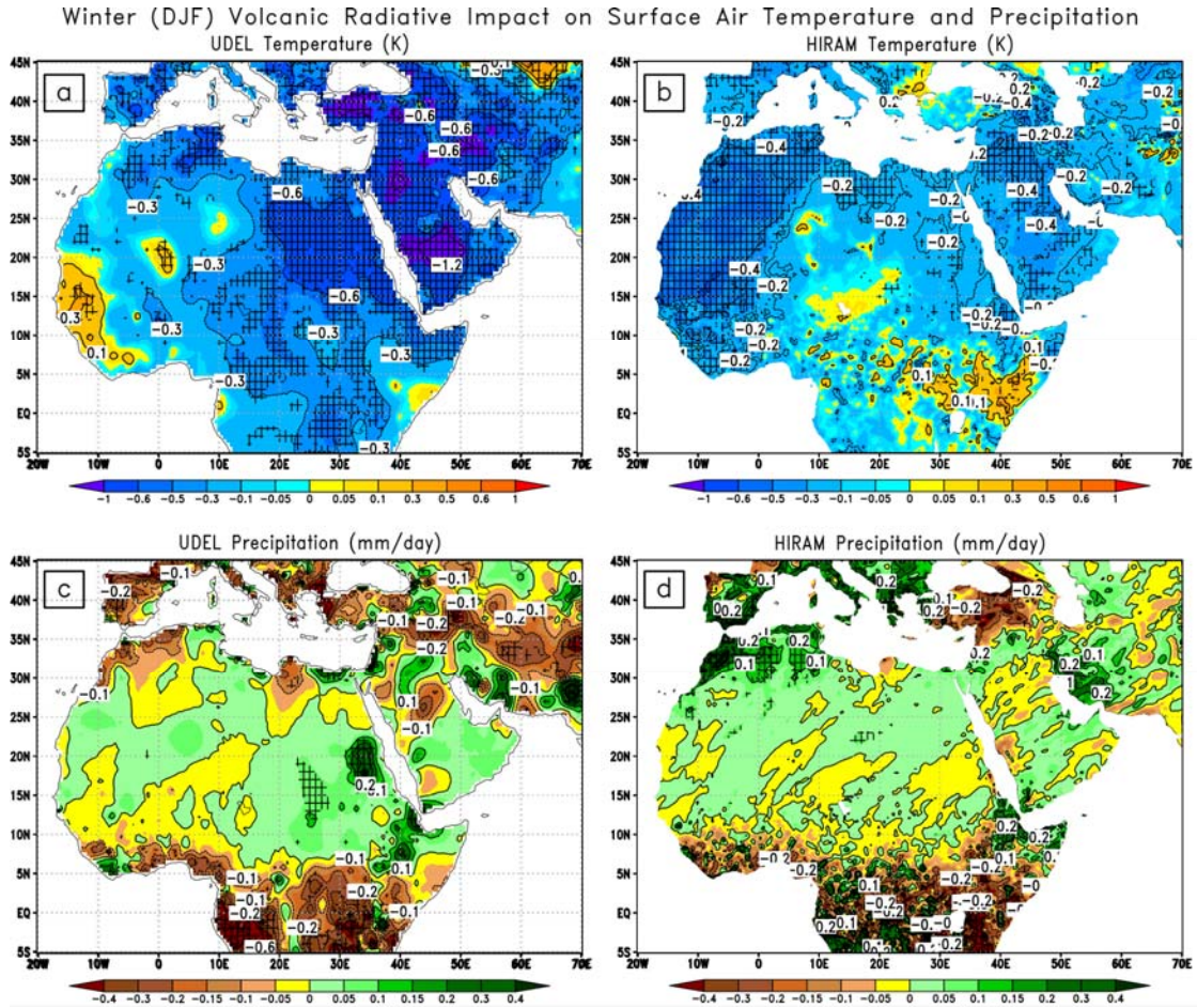
Figure 4.8: Winter (DJF) anomalies of surface air temperature (K) and precipitation (mm/day) regressed on the residual term (volcanic effect) composited for two winter seasons following both the El Chichón and Pinatubo eruptions. The temperature composites are calculated using a) UDEL observations, b) HiRAM output, and precipitation composites using c) UDEL observations, d) HiRAM output. Hatching shows the statistically significant areas with at least 95% confidence level examined by bootstrapping with replacement test.
