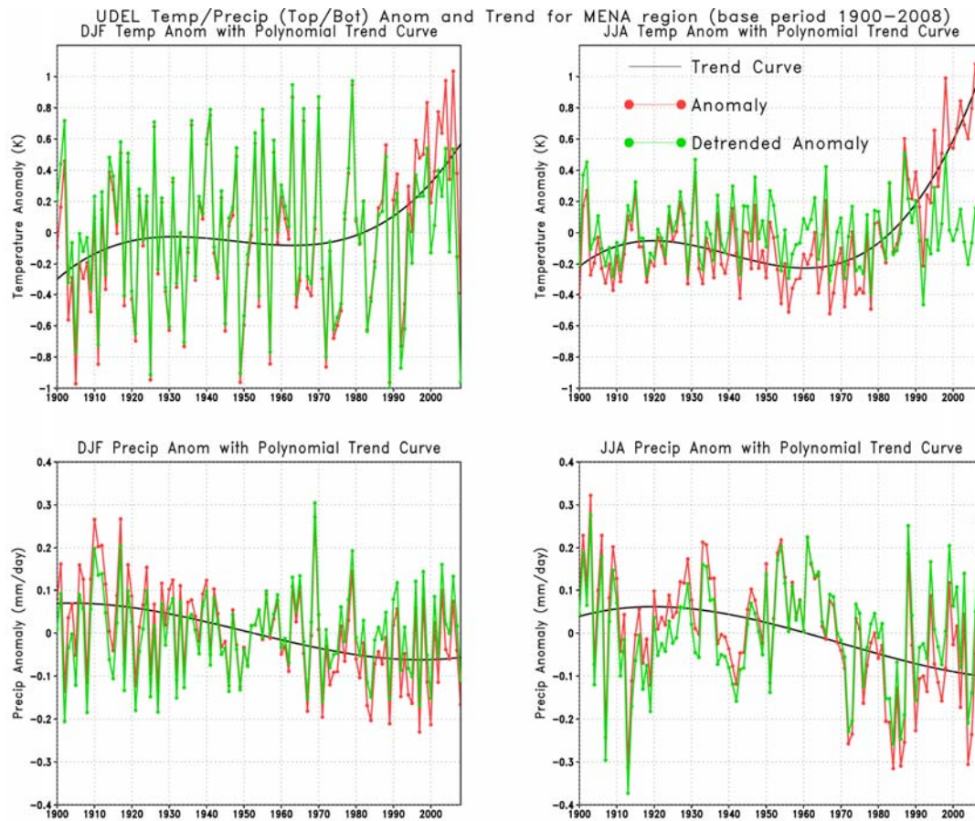
Figure 3.5: The polynomial trend curve for temperature/precipitation (top/bottom) fields in winter/summer (left/right) computed over MENA region over a longer period of 1900-2008. The anomalies of temperature and precipitation before (red curve) and after removing polynomial trend (green curve) are also shown.
