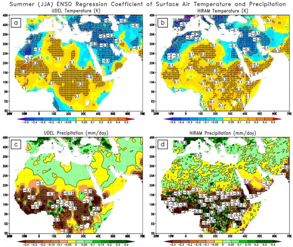
Figure 3.9: Summer (JJA) ENSO regression coefficient with surface air-temperature (K) calculated using a) UDEL 30-year period, b) Model 30-year period, and with precipitation (mm/day) calculated using c) UDEL 30-year period, d) model 30-year period. Hatching shows the statistically significant areas with at least 95% confidence level.
