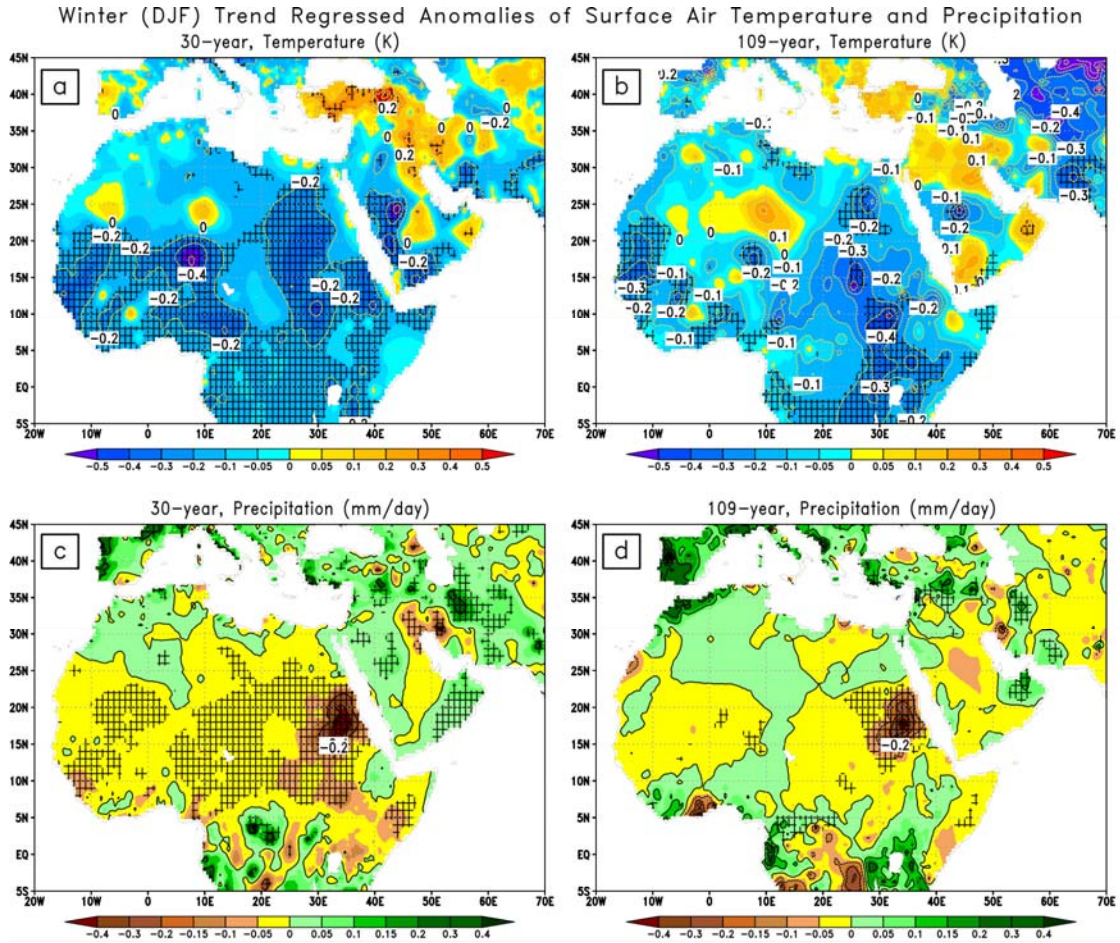
Figure 4.16: Anomalies of trend-component-regressed surface air temperature (K) and precipitation (mm/day) composited for two winter (DJF) seasons following both the El Chichón and Pinatubo eruptions. The temperature composites are calculated using a) UDEL 30-year period, b) UDEL 109-year period, and precipitation composites using c) UDEL 30-year period, d) UDEL 109-year period. Hatching shows the statistically significant areas with at least 95% confidence level examined by bootstrapping with replacement test.
