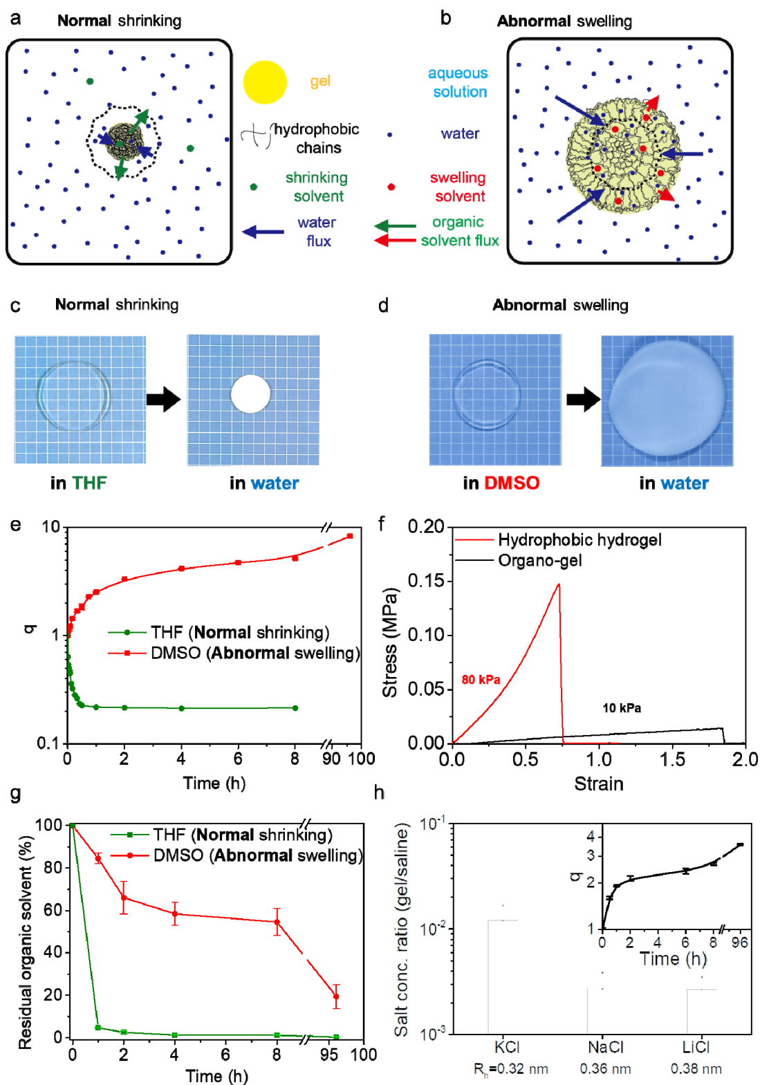
Figure 1 (a-b) Schematic illustration of organo-gels' volume change upon solvent exchange and the formation of "hydrophobic hydrogels". When organo-gels constructed from hydrophobic network pre-swelled in an omniphilic organic solvent are immersed in water, phase separation occurs. Depending on the relative affinity of the organic solvent to the polymer and water, normal shrinking (a) or abnormal swelling (b) of the organo-gel in water occurs (The dash line in figures illustrated the initial size of organo-gels). In the normal case, the diffusion of the organic solvent and
