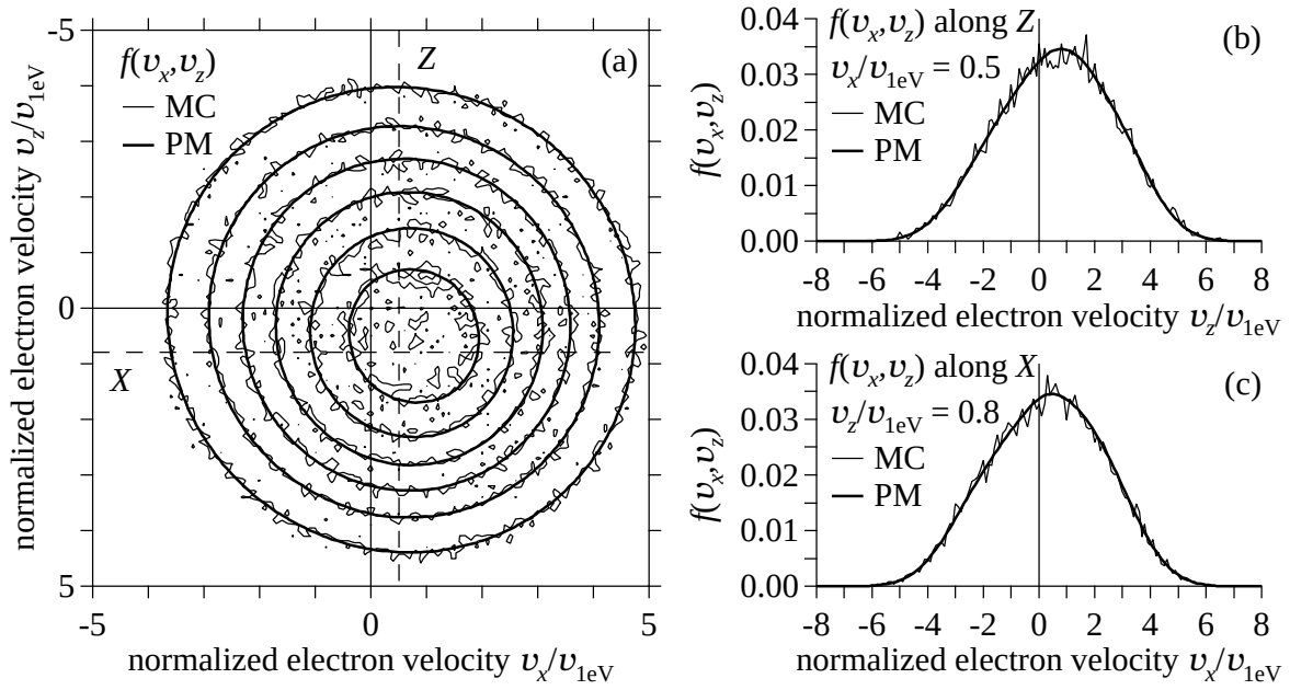
Figure 5. The EVDF in \text{SF}_6 at E/N = 1000 \text{ Td} and B/N = 1000 \text{ Hx} . (a) contours of f(v_x, v_z) from 0.005 to 0.030 in steps of 0.005, (b) f(v_x, v_z) along cross section Z at v_x/v_{1\text{eV}} = 0.5 , and (c) f(v_x, v_z) along cross section X at v_z/v_{1\text{eV}} = 0.8 . v_x and v_z are the velocity components in the directions of \mathbf{E} \times \mathbf{B} and -\mathbf{E} , respectively. f(v_x, v_z) has its peak at the intersection between X and Z.
