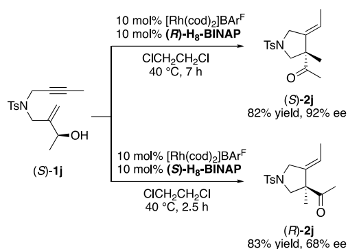
Scheme 4. Cyclization of ( S )- 1j with Rh + /( R )- or ( S )-H 8 -BINAP.
