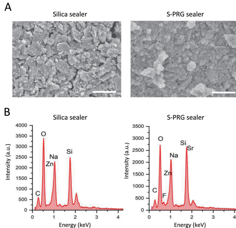
Fig. 1 Characterization of S-PRG and silica sealers. (A) SEM micrographs of S-PRG and silica sealers. Scale bar represents 10 µm. (B) EDX analysis of S-PRG and silica sealers. EDX, energy dispersive X-ray spectrometry; SEM, scanning electron microscopy; S-PRG, surface pre-reacted glass-ionomer.
