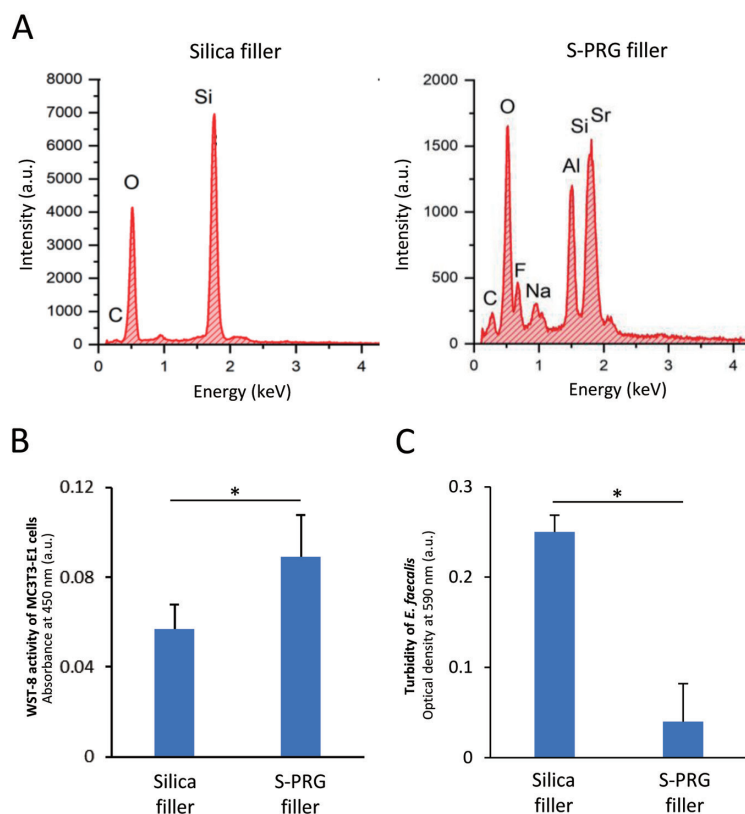
Fig. 5 Characterization of S-PRG and silica fillers. (A) EDX analysis of S-PRG and silica fillers. (B) WST-8 activity of MC3T3-E1 cells after 24-h incubation ( n=5 , mean \pm SD). * p<0.05 . (C) Turbidity of E. faecalis after 24-h incubation ( n=5 , mean \pm SD). * p<0.01 . EDX, energy dispersive X-ray spectrometry; S-PRG, surface pre-reacted glass-ionomer; WST-8, water-soluble tetrazolium salt-8.
