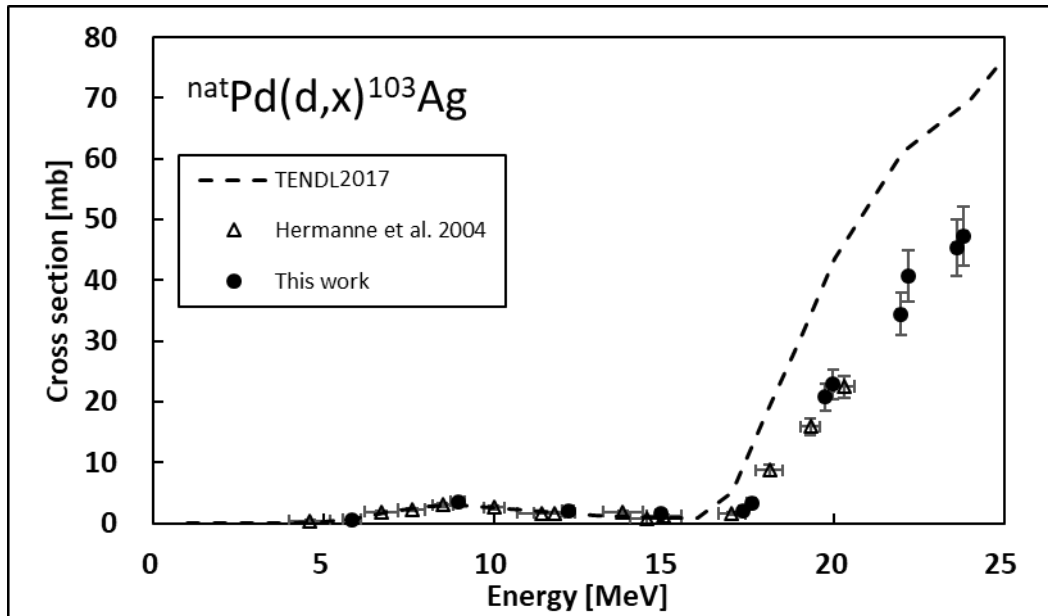
Fig. 2: The excitation function of the ^{nat}\text{Pd}(d,x)^{103}\text{Ag} reaction
