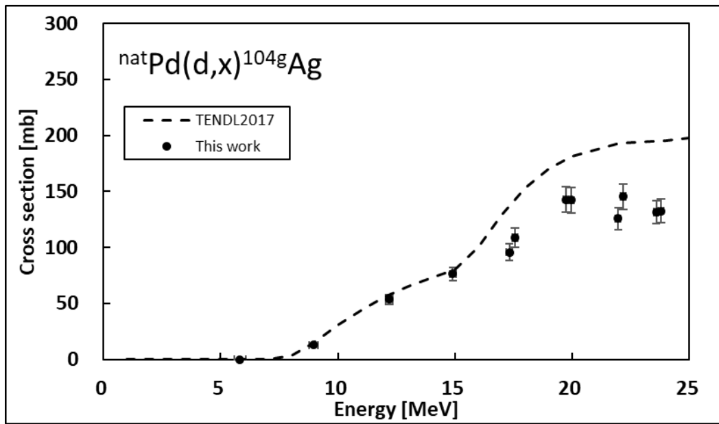
Fig. 3: The excitation function of the ^{nat}\text{Pd}(d,x)^{104g}\text{Ag} reaction
