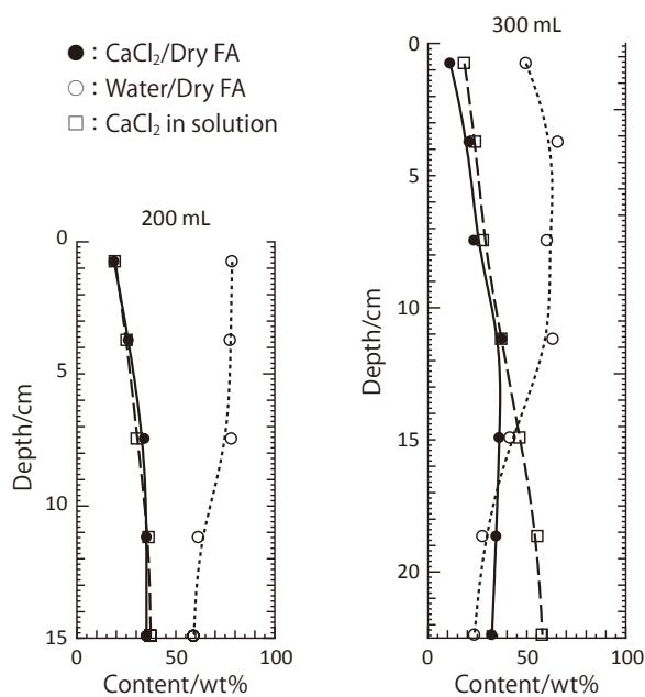
Fig. 7 Depth profiles of the contents of water and \text{CaCl}_2 for MSWI FA containing 30 wt% of \text{CaCl}_2 in 200 mL and 300 mL cylinders after 2000 hours moisture absorption at 50°C 90%RH
