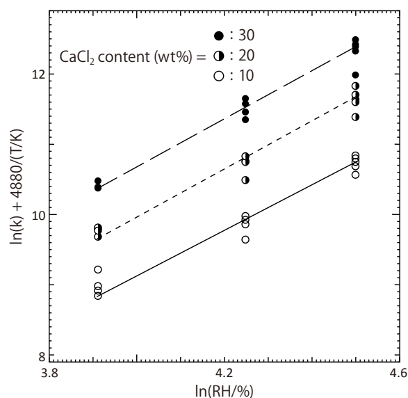
Fig. 12 Effects of relative humidity and \text{CaCl}_2 content on the rate constant k of moisture absorption
