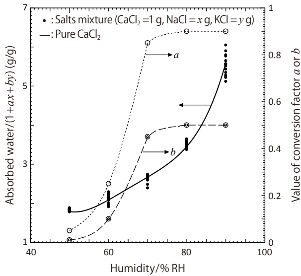
Fig. 15 Comparison of observed moisture absorption capacities of the mixtures of \text{CaCl}_2 , \text{NaCl} and \text{KCl} (solid circles) with those derived from Eq. (6) (solid curve)
