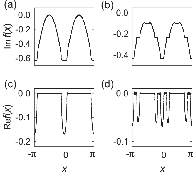
FIG. 5. Profile of Eq. (30) for the type I [(a) and (c)] and the type II [(b) and (d)] breathing chimera corresponding to Figs. 2 and 4, respectively. [(a), (b)] The imaginary part denotes the average frequency. [(c), (d)] The real part denotes the linear stability against a small local perturbation, where it is negative in stable coherent regions and zero in neutral incoherent regions. All figures are depicted by computing z_k(x) and Y_k(x) for k \in [-5, 5] obtained by the numerical simulation of Eq. (3).
