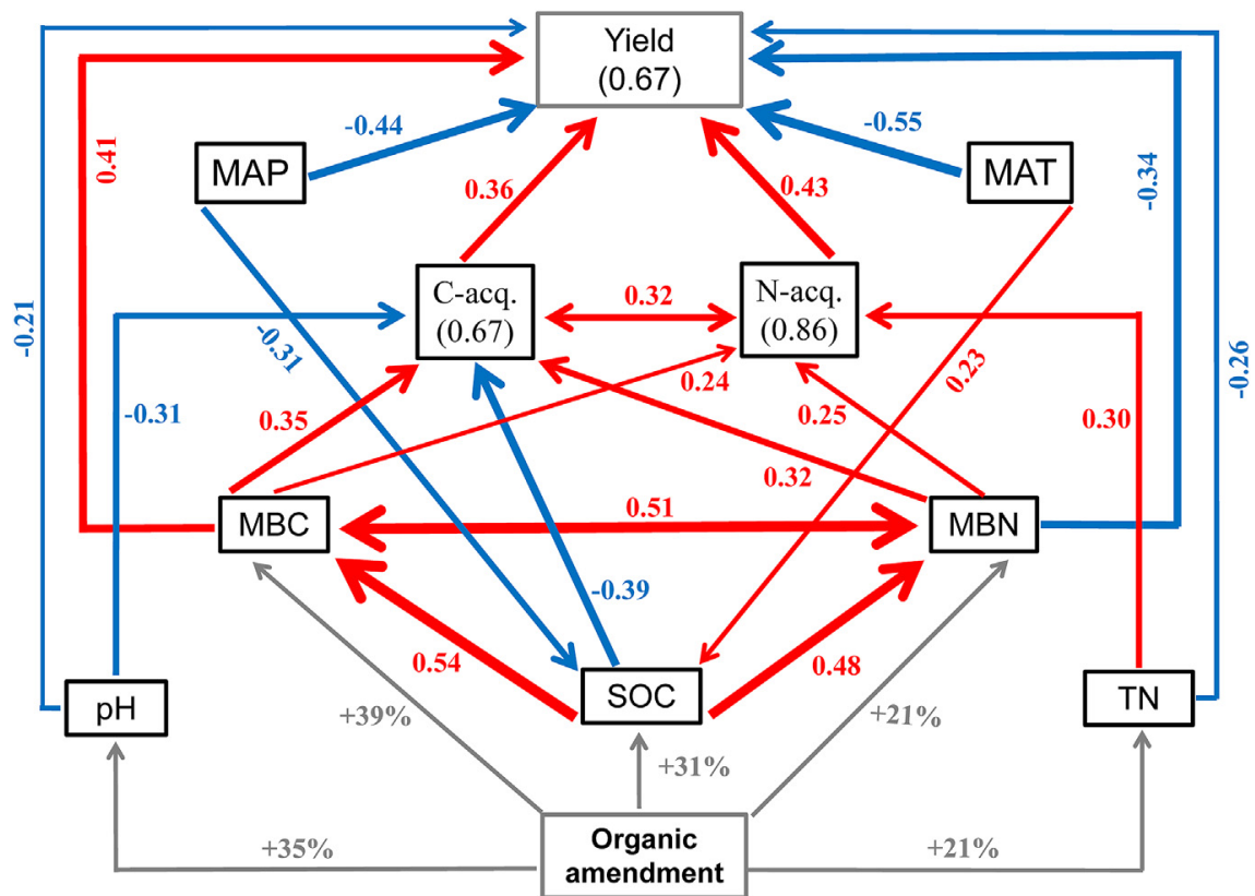
Figure 2.4. Structural equation model (SEM) showing the direct and indirect effects of climatic (MAP and MAT), soil physicochemical factors (SOC, TN, and pH), microbial biomass (MB) pools and soil enzyme activities on crop yields under organic amendments. The red and blue arrows represent significantly positive ( p < 0.05 ) and negative ( p < 0.05 ) relationships, respectively. The grey arrows show the effects of organic amendment on soil physicochemical properties and MB pools (TN, SOC, pH, MBC, and MBN) - the percentage next to grey arrows denote the relative effect of organic to mineral-only fertilization on a given variable. Numbers next to red and blue arrows denote for path coefficients between different variables and the thickness of the arrows represent the magnitude of these effects. Figure abbreviations denote for: soil organic carbon (SOC), soil total nitrogen (TN), C-acquisition enzyme activity (C-acq), N-acquisition enzyme activity (N-acq), mean annual temperature (MAT), mean annual precipitation (MAP), microbial biomass carbon (MBC), and microbial biomass nitrogen (MBN). (Source: Luo et al., 2018)
