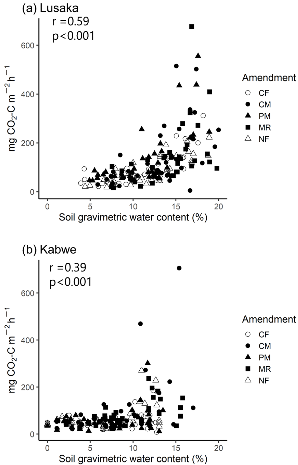
Figure 5.3. Relationship between CO 2 emission rates and soil moisture at (a) Lusaka site and (b) Kabwe site. CF: chemical fertilizer amendment, CM: cattle manure amendment, PM: poultry manure amendment, MR: maize residue amendment, and NF: no fertilizer amendment.
