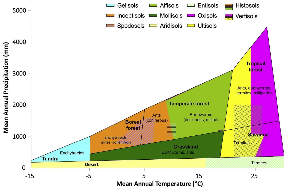
Figure 2.2. Abiotic and biotic factors constituting soil quality in the soils of the world (Source: Bünemann et al., 2018)
