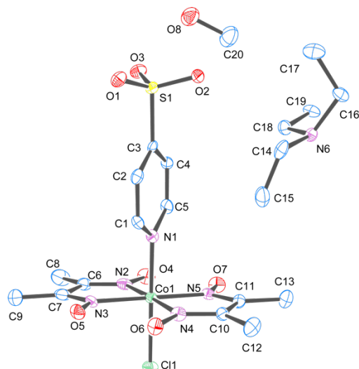
Fig. 2 ORTEP drawing of the molecular structure of \text{HNEt}_3[\text{Co}^{\text{III}}\text{Cl}(\text{Hdmg})_2(4\text{-pySO}_3)] \cdot \text{CH}_3\text{OH} showing 50% probability thermal ellipsoids and the atom-numbering scheme.
