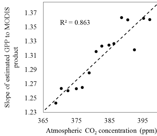
Fig. S4 Relationship between the slopes of the estimated GPP to MODIS product and atmospheric CO 2 concentration.
