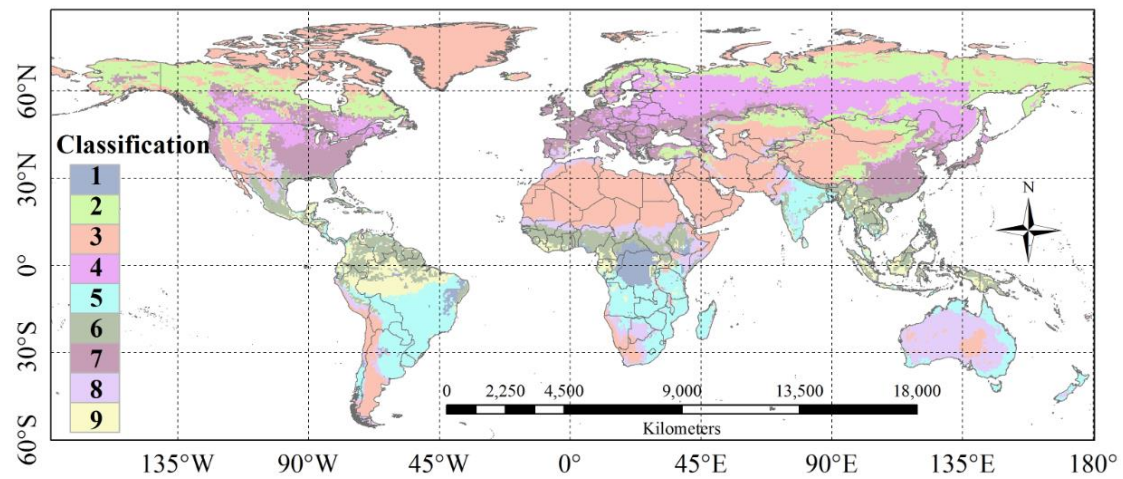
Fig. 5 The spatial distribution of classes on variations in GPP during the period 1982-2015.
