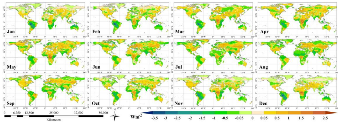
Fig. S7 The monthly spatial distributions of linear trends in radiation during the period 1982-2015.
