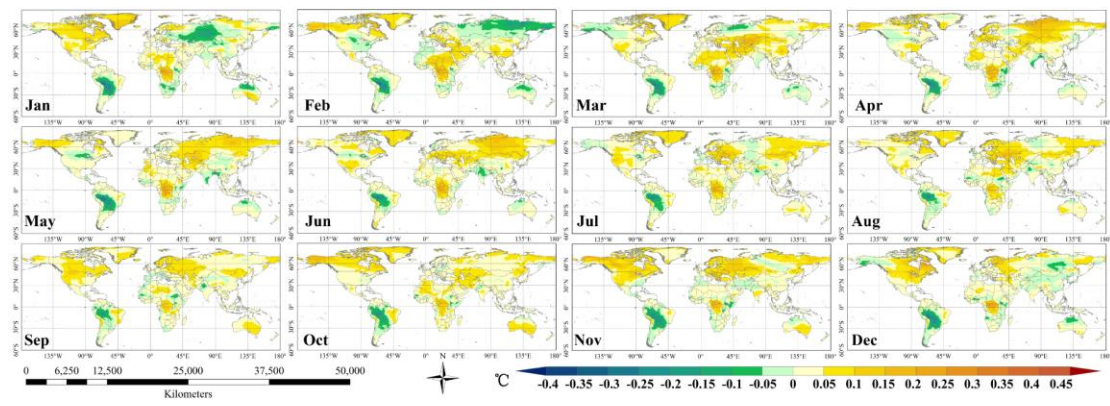
Fig. S9 The monthly spatial distributions of linear trends in temperature during the period 1982-2015.
