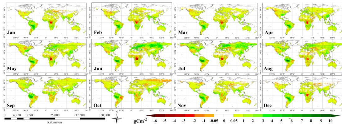
Fig. S5 The monthly spatial distributions of linear trends in GPP during the period 1982-2015.
