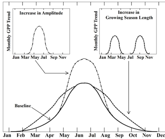
Fig. 2 Schematic showing monthly trends in GPP in response to an increase in the amplitude if the GPP annual cycle (dashed-dotted curve) and an increase in the length of the growing season (dashed curve) occurred from a baseline GPP annual cycle (solid curve).
