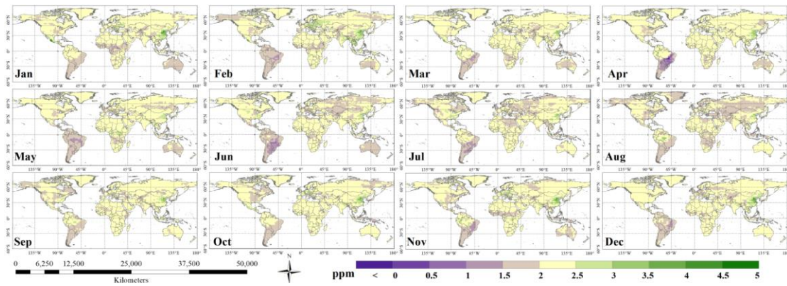
Fig. S6 The monthly spatial distributions of linear trends in atmospheric CO 2 concentrations during the period 1982-2015.
