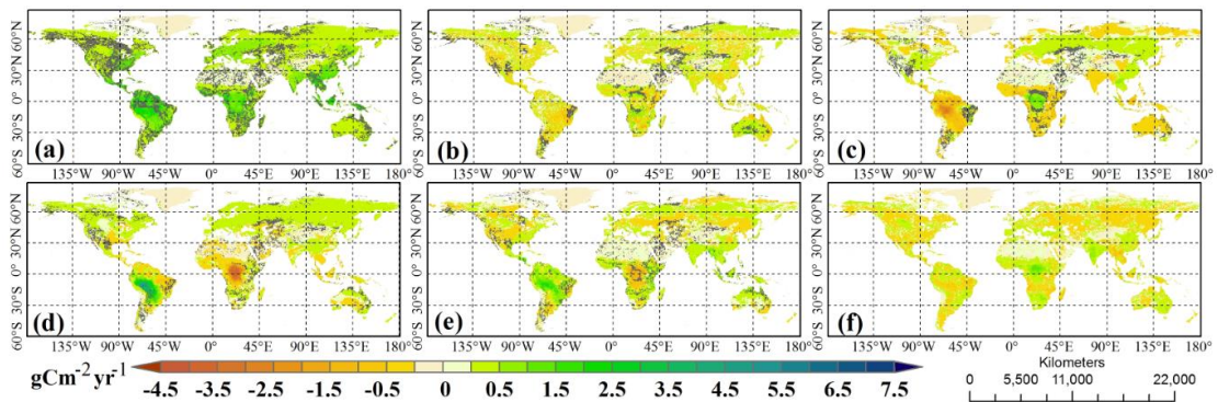
Fig. 4 Spatial distribution of the trends in GPP due to (a) increases in atmospheric CO_2 concentration, (b) land-cover change, (c) solar radiation changes, (d) temperature changes, (e) changes in water conditions, and (f) their nonlinear interactions or non-attributed. The pixels ((a) to (e)) that are not satisfied at p\_value < 0.1 are drawn in gray.
