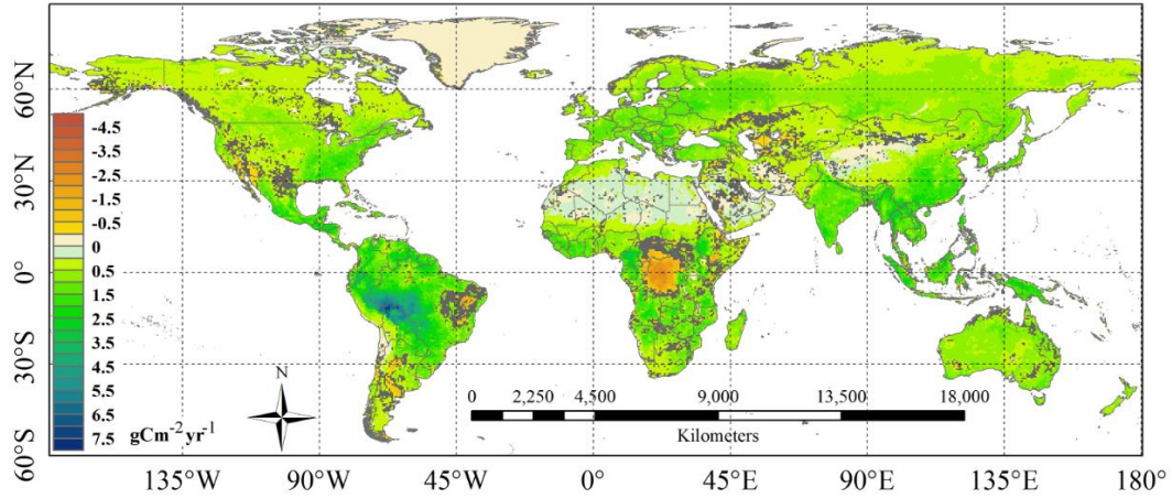
Fig. 3 The spatial distribution of linear trends in GPP during the period 1982-2015. The pixels that are not satisfied at p\_value < 0.1 are drawn in gray.
