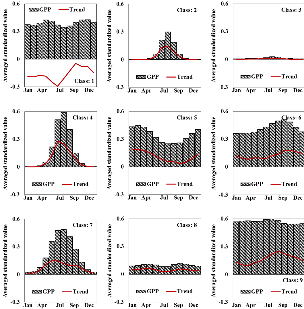
Fig. 6 Characteristics of the annual cycle of the growing season distribution and GPP trends associated with each class.
