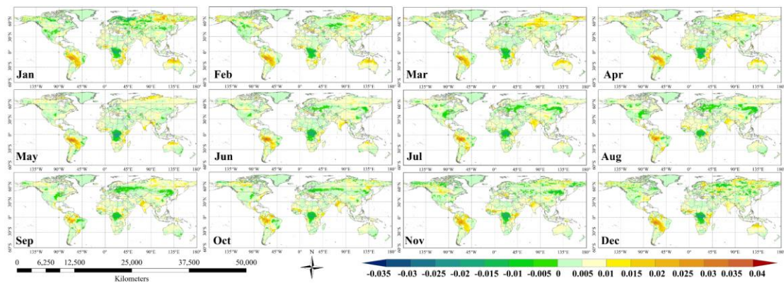
Fig. S8 The monthly spatial distributions of linear trends in water conditions during the period 1982-2015.
