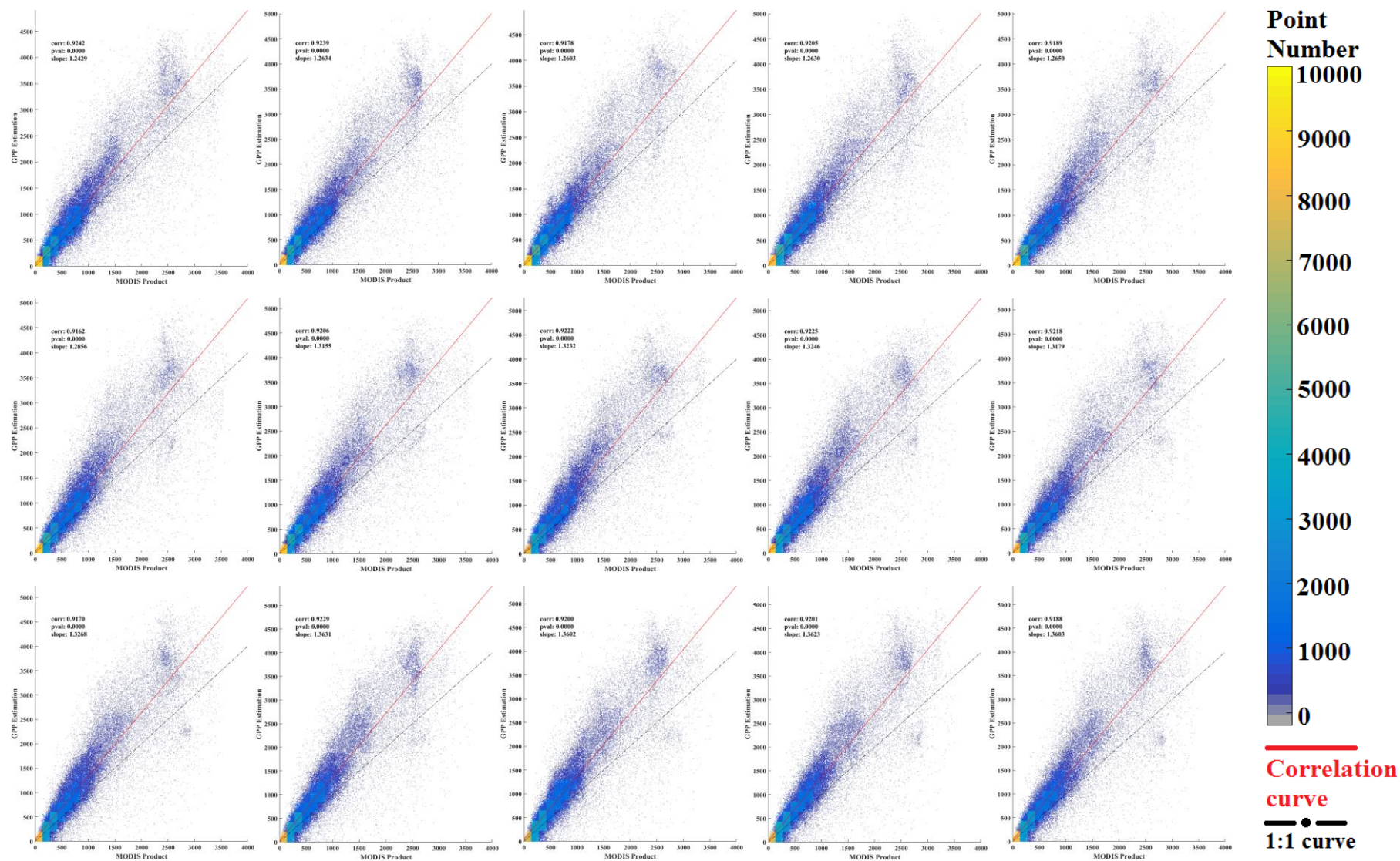
Fig. S3 Scatter plots of estimated GPP values ( y axis) vs. MODIS Product ( x axis) from 1982 to 2011. Only pixels over vegetated areas are shown. The parameters of the linear regression line in all panels are shown in Table S1.
