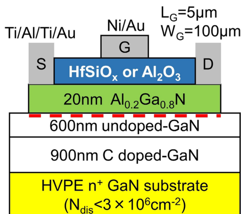
FIG. 1. Schematic illustration of the \text{AlGaN}/\text{GaN} MOS HEMT with \text{HfSiO}_x or \text{Al}_2\text{O}_3 as a gate dielectric.
