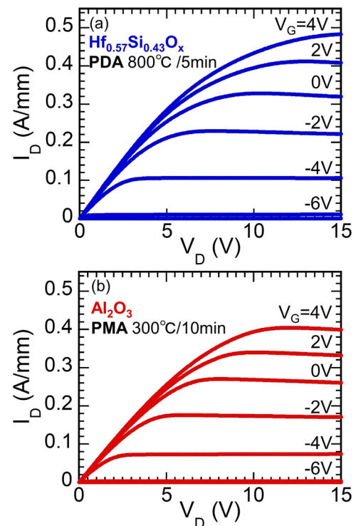
FIG. 3. Typical drain I - V characteristics of MOS HEMTs with (a) \text{HfSiO}_x and (b) \text{Al}_2\text{O}_3 gates.
