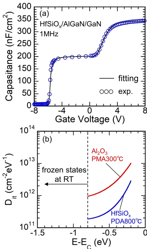
FIG. 6. (a) The best fitting result to experimental C-V plots (1 MHz). (b) Interface state density ( D_{it} ) distributions at HfSiO x /AlGa 0.3 N and Al 2 O 3 /AlGa 0.3 N interfaces extracted from the fitting result.
