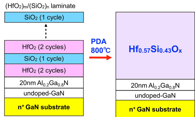
FIG. 2. Deposition procedure of the (\text{HfO}_2)_m/(\text{SiO}_2)_n laminate and formation of the \text{HfSiO}_x layer after PDA at 800^\circ\text{C} .
