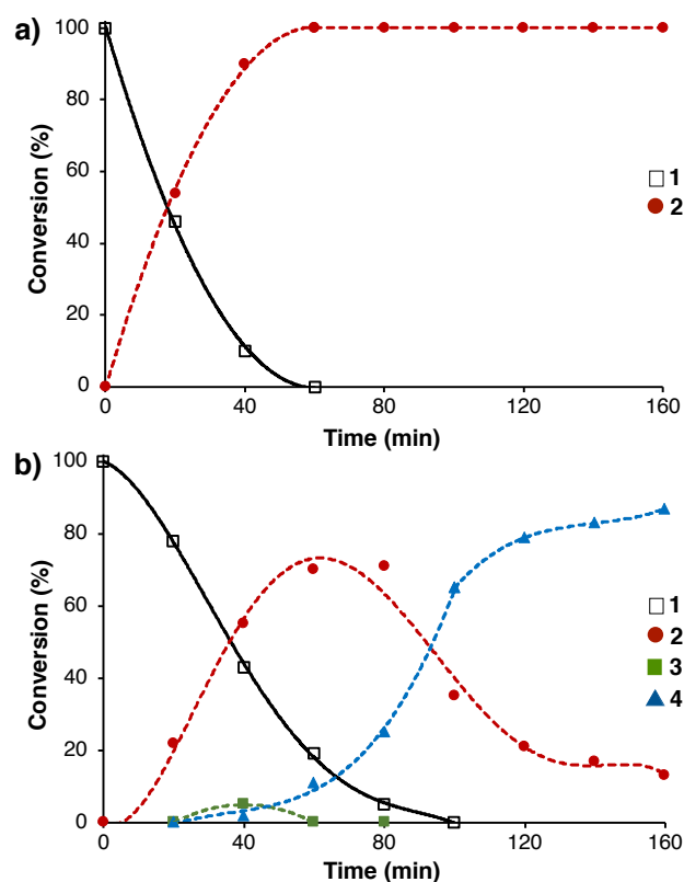
Figure 1. Time courses of transfer hydrogenation of 1a . a) 1a (0.2 mmol), [\text{IrCl}(\text{cod})_2] (1 mol% Ir), DCyPE (1 mol%), 1,4-dioxane (1 mL), 120 °C (Teflon ® -sealed screw vial). b) 1a (0.2 mmol), [\text{IrCl}(\text{cod})_2] (4 mol% Ir), DCyPE (4 mol%), 2-propanol (1 mL), 60 °C (Teflon ® -sealed screw vial).
