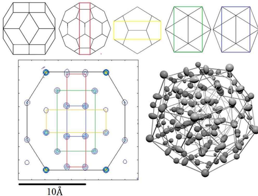
Figure 37. The Bergman cluster in the i-ZnMgHf F-type QC is composed of five shells: (from left) rhombic triacontahedron, soccer-ball polyhedral, dodecahedron, icosahedron and inner icosahedron. The
