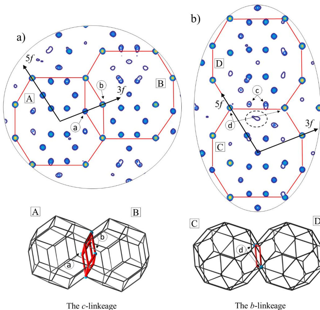
Figure 20. a) The section through the c -linkage occurring in the structure of i-ZnMgTm with RTH clusters marked with a red line. The 3D visualization is provided. Atoms ‘a’ (‘b’) are co-shared by the #5 shell of cluster ‘B’ (‘A’) and #3 shell of cluster ‘A’ (‘B’); b) The section through the b -linkage occurring in the structure. The indication of the split atomic sites ‘c’ is made.
