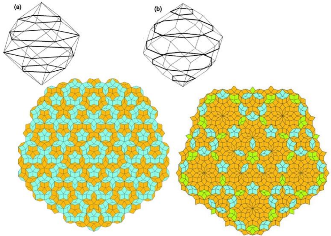
Figure 4. The General Penrose Tiling constructed for the shift parameter equal to 0, that constitutes a simple Penrose Tiling (a)) and for shift equal to 0.5 (b)). The shift parameter defines the position of the section planes through a 3D that is embedded in the perpendicular space of the decagonal quasicrystal. Source: figure based on the images found in [123, 122]
