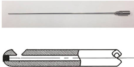
FIGURE 1: Photograph of the MK01 cannula and of the shape of the open orifice. The distal side of the opening orifice is curved just proximal to the equator line of the spherical tip so that the opening orifice does not appear from the inserting trajectory view.
