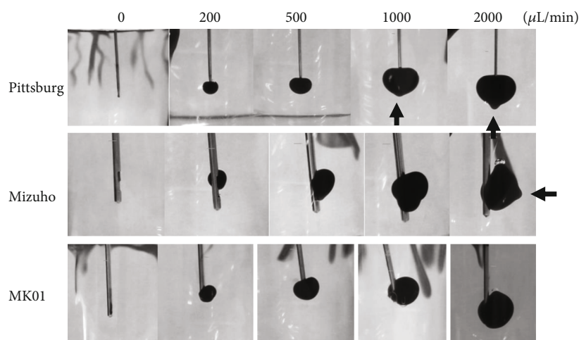
FIGURE 5: Colored saline injected in the gel imitating the brain. The Pittsburgh and Mizuho needles showed jet flow prominence (arrow) at 2000 \mu\text{L}/\text{min} (arrow), while MK01 did not cause protuberance.
