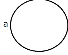
Figure 3 : Trivial knots
