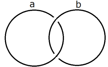
Figure 2 : Hopf link
