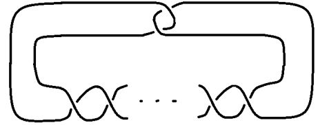
Figure 5 : Twist knots
