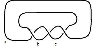
Figure 1 : T(2, 3)
