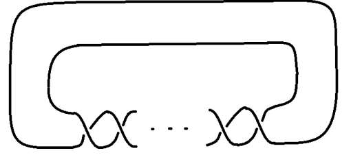
Figure 4 : Torus knots
