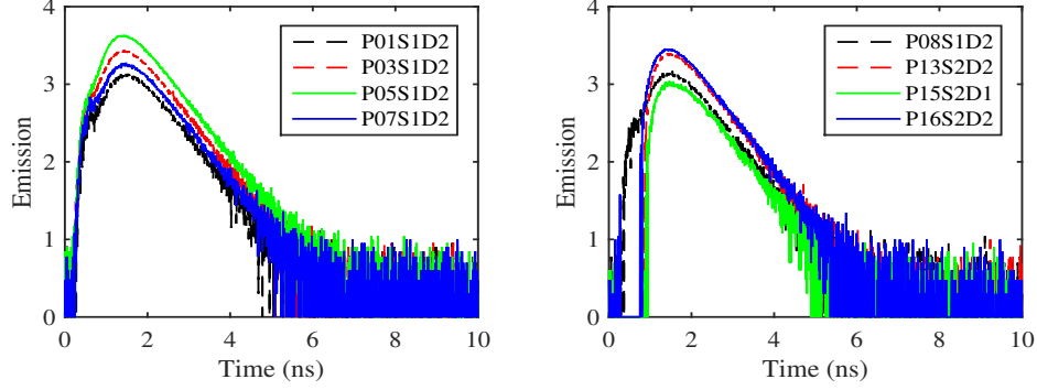
FIGURE 7.6: TPSFs (the logarithm value) with the position of holder at P1, P3, P5, P7, P8, P13, P15 and P16.
