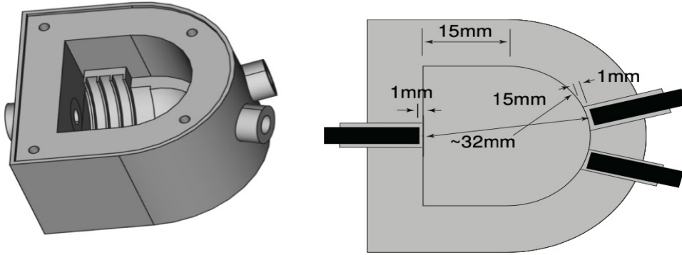
FIGURE 7.2: The IRF measurement adapter. The adapter holds some attenuation filters and a small diffuser to homogenize the light.
