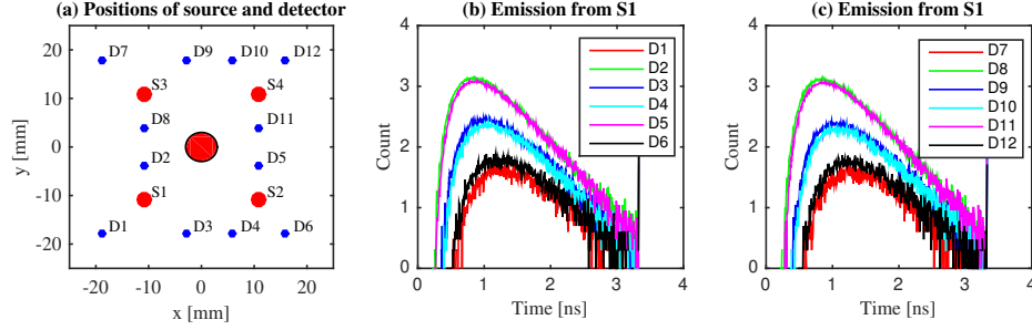
FIGURE 4.4: (a) The positions of four sources (small red circles) and twelve detectors (small blue points). The big red circle is the projection of spherical target to the boundary. (b), (c) are the TPSFs (the logarithm value) to different detectors corresponding to source S_1 .
