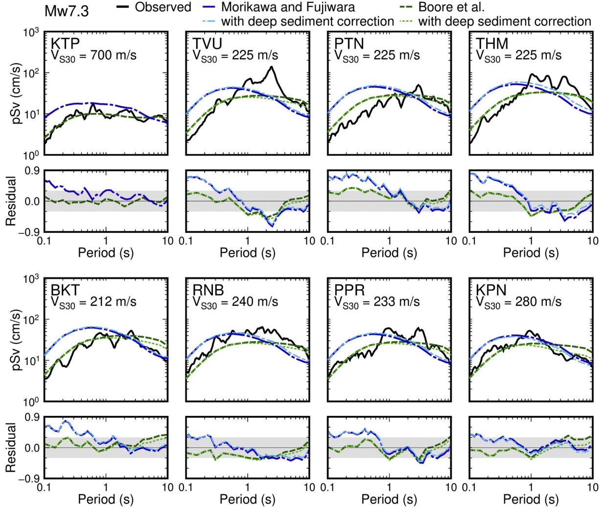
Fig. 4. Comparison of observed pseudo-velocity response spectra of event 5 ( M_w 7.3) and the corresponding records predicted by the two GMPEs [12,13] (upper) and residuals ( \log [\text{pre}/\text{obs}] ) (lower). Predicted values are shown also in the case that amplification by deep sedimentary layer is corrected.
