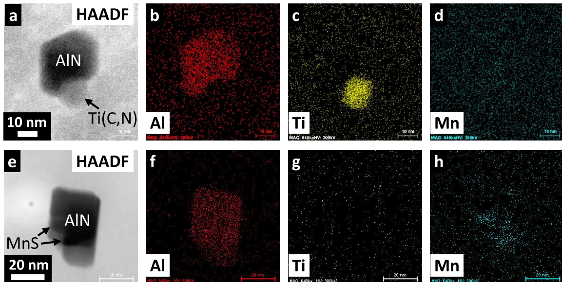
Fig. 4. HAADF-STEM images and corresponding STEM-EDS mapping of the as-received sample. (Online version in color.)
