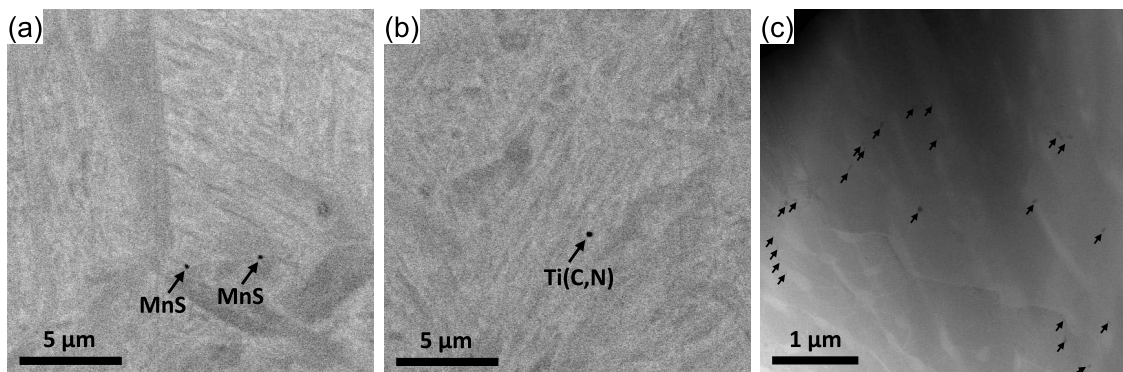
Fig. 3. (a, b) SEM images and (c) HAADF-STEM image of the as-received sample.
