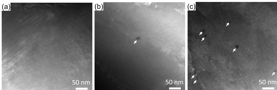
Fig. 7. HAADF-STEM observations of (a) solution-treated at 1300^\circ\text{C} , (b) 780^\circ\text{C} \times 1 after solution treatment, and (c) 780^\circ\text{C} \times 3 after solution treatment.
