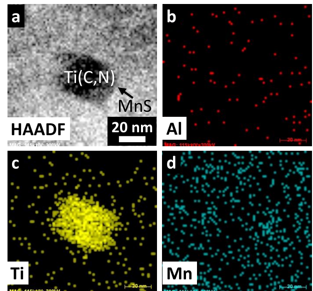
Fig. 5. (a) HAADF-STEM image and (b–d) corresponding STEM-EDS mapping of the sample solution-treated at 1 100°C. (Online version in color.)
