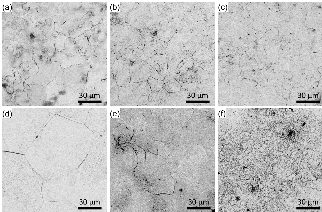
Fig. 2. SEM images of samples (a) as-received, (b) 780°C × 1, (c) 780°C × 3, (d) solution-treated at 1300°C, (e) 780°C × 1 after 1300°C solution treatment, and (f) 780°C × 3 after 1300°C solution treatment.
