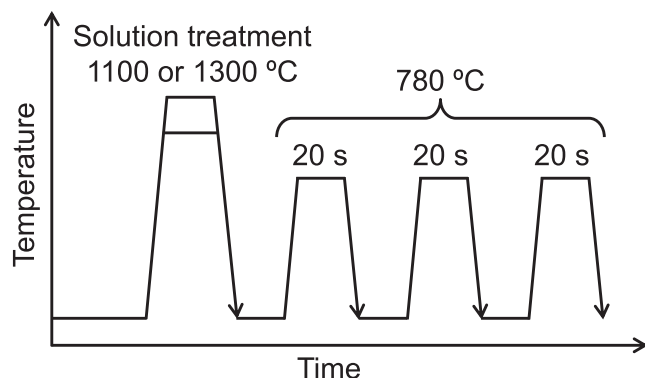
Fig. 1. Heat pattern of the cyclic heat treatment.
