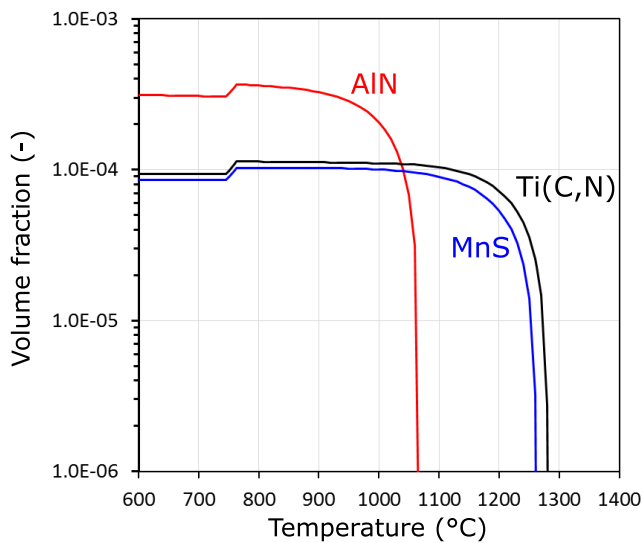
Fig. 6. Volume fraction of each precipitate determined by performing thermodynamic calculations. (Online version in color.)
