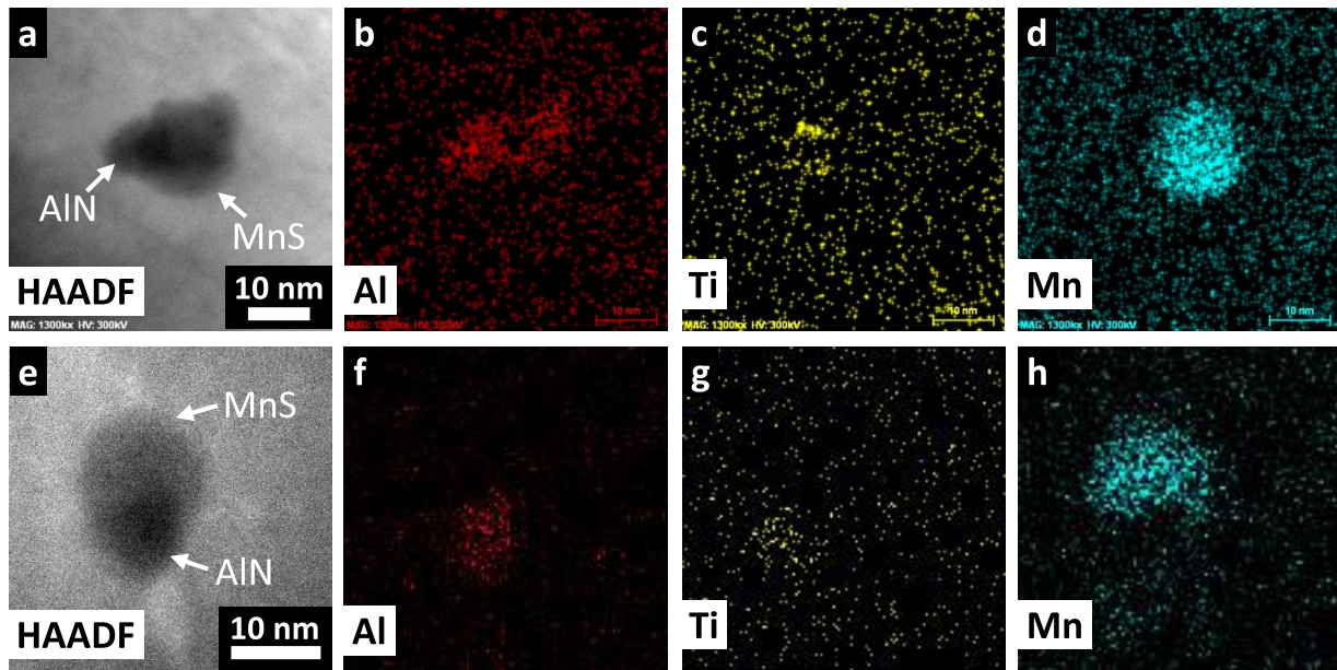
Fig. 8. HAADF-STEM images and corresponding STEM-EDS mapping for (a–d) 780°C × 1 after 1 300°C solution treatment and (e–h) 780°C × 3 after 1 300°C solution treatment. (Online version in color.)
