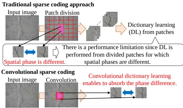
Figure 2 Difference between traditional sparse coding and convolutional sparse coding.
