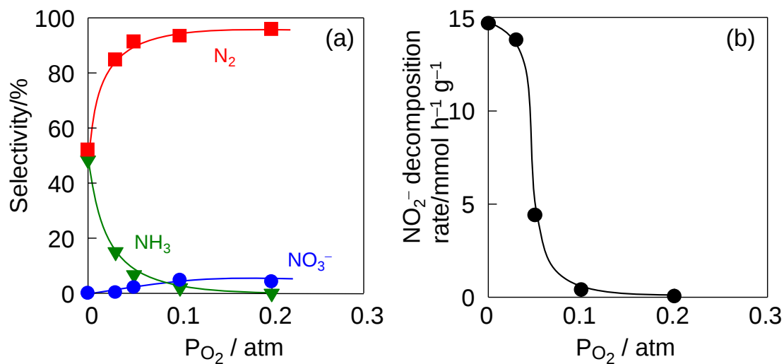
Figure 4 Influence of O_2 partial pressure on (a) selectivity and (b) NO_2^- decomposition rate for the catalytic hydrogenation of NO_2^- in water over Pt/Al_2O_3 . Reaction conditions: KNO_2 , 1.0 \text{ mmol dm}^{-3} ; volume of reaction solution, 100 \text{ cm}^3 ; total pressure, 1.0 \text{ atm} ; gas composition, H_2:CO_2:Ar:O_2 = 1:3:6-4:0-2 ; gas flow rate, 100 \text{ cm}^3 \text{ min}^{-1} ; and reaction temperature, 298 \text{ K} .
