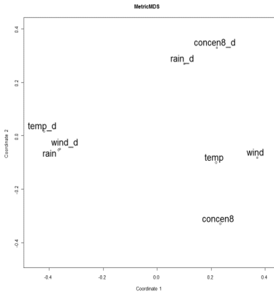
Fig.5.9 Cophenetic similarity distance between variables
