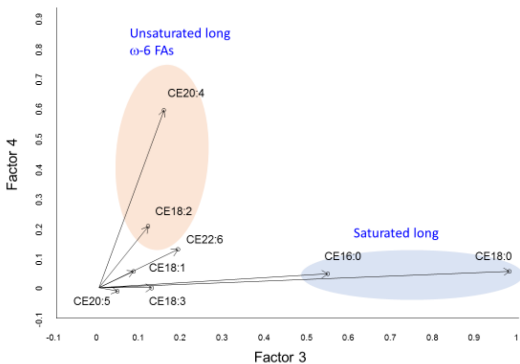
Fig.4.15 Result of CE dataset (factor analysis)
