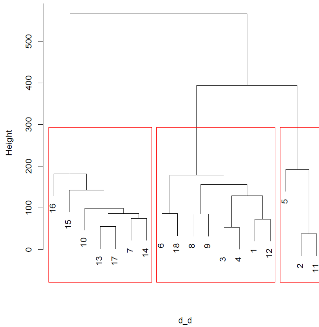
Fig.5.2 Clustering for milk concentration FA 8:0 derivatives
