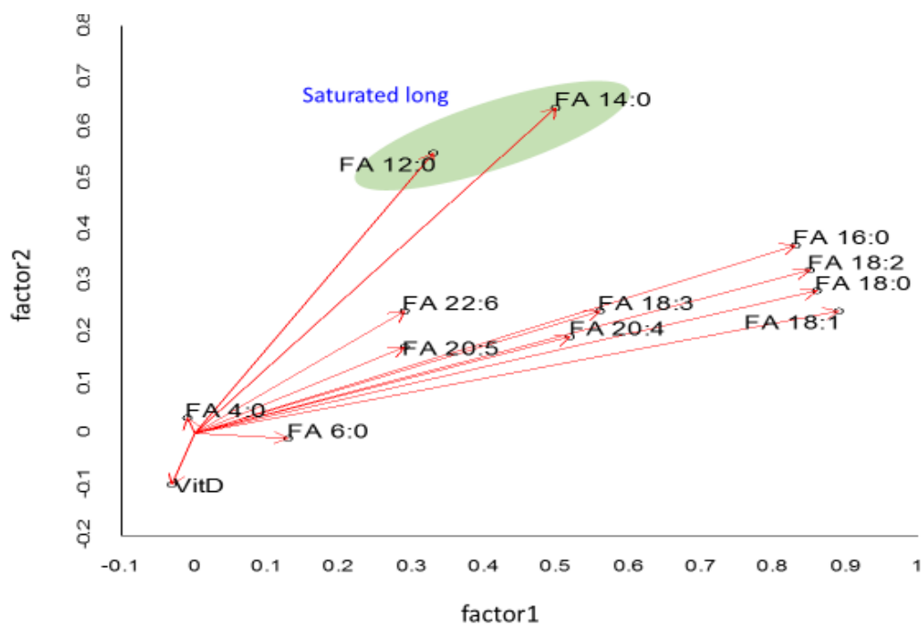
Fig.4.4 Result of free fatty acid dataset (factor analysis)
