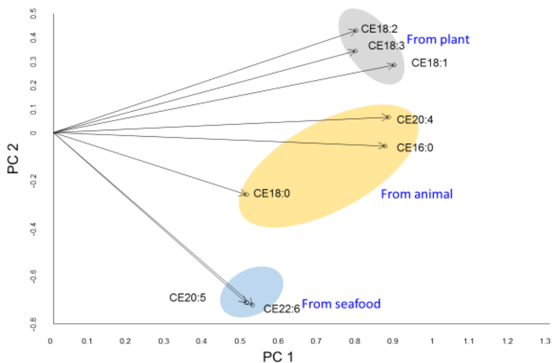
Fig.4.13 Result of CE dataset (PCA)
