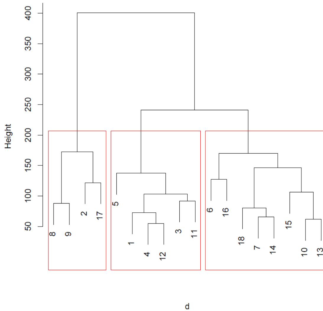
Fig.5.1 Clustering for milk concentration FA 8:0
