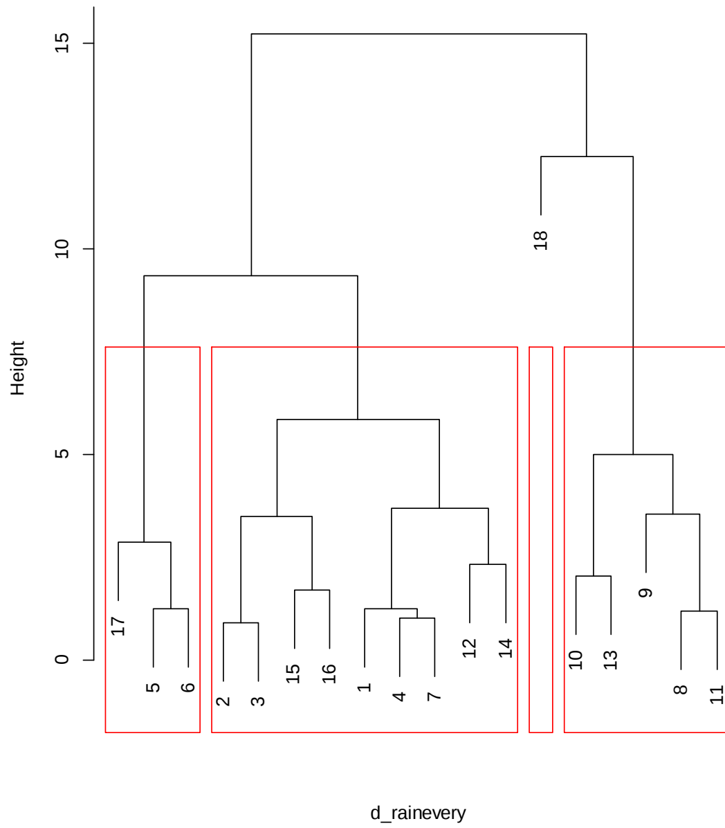
Fig.5.3 Clustering for sum of rain everyday
