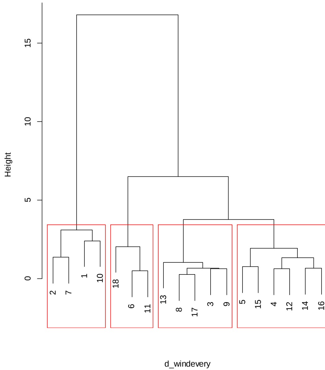
Fig.5.4 Clustering for wind speed everyday
