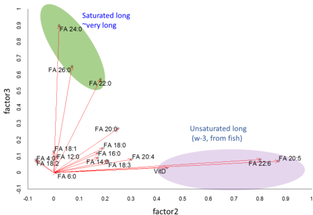
Fig.4.2 Result of total fatty acid dataset (factor analysis)
