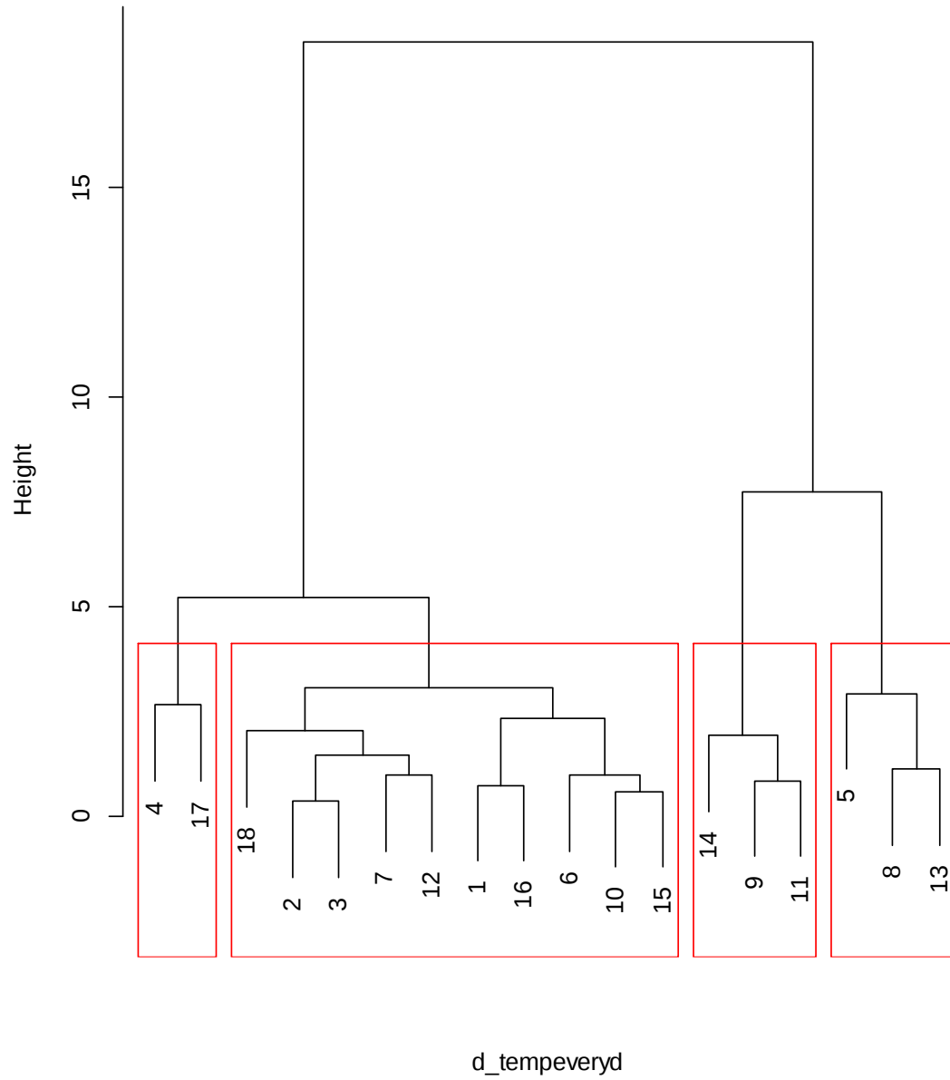
Fig.5.8 Clustering for average temperature everyday derivatives
