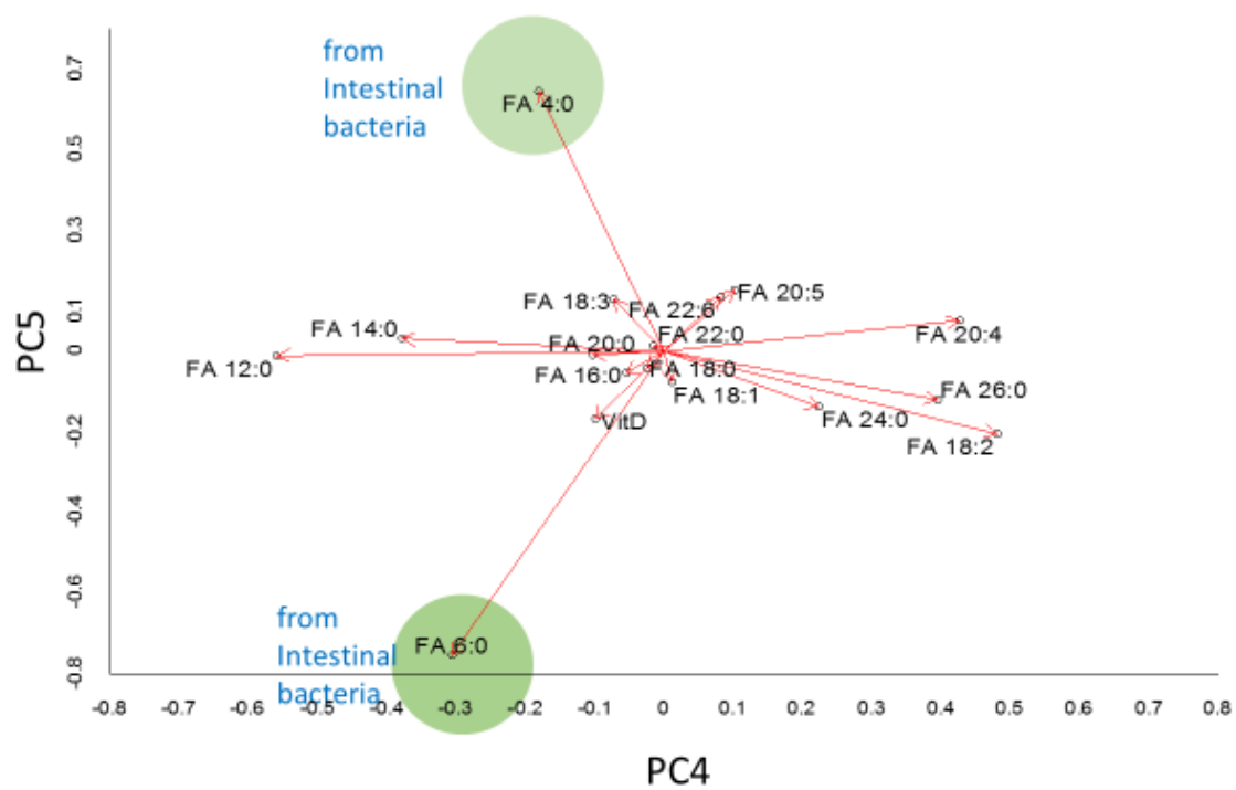
Fig.4.8 Result of total fatty acid dataset (PCA)
