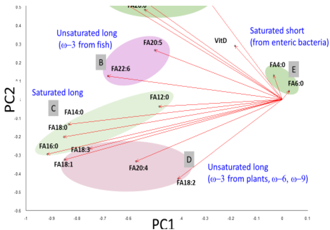
Fig.4.6 Result of total fatty acid dataset (PCA)
