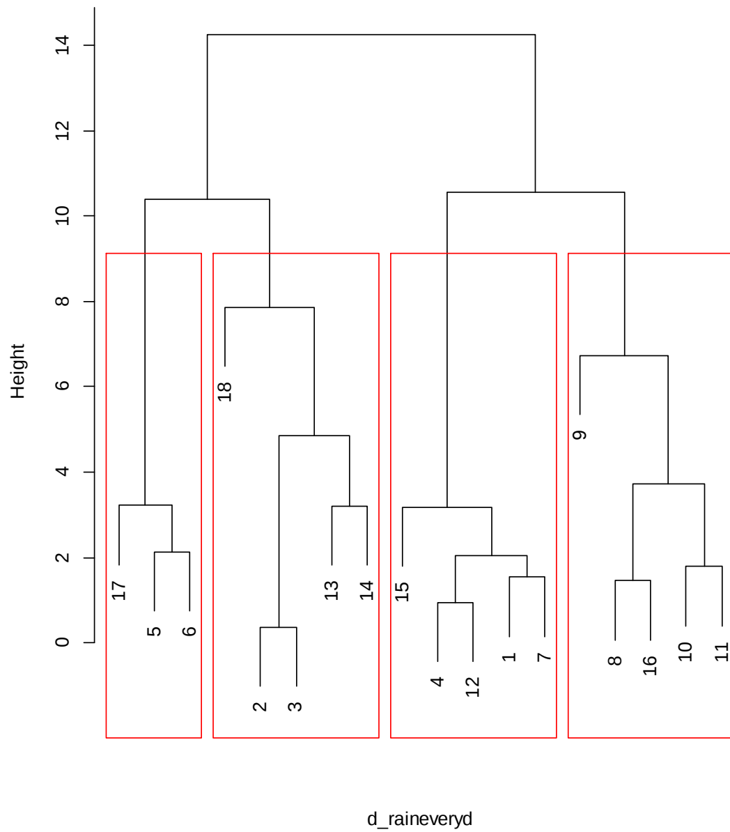
Fig.5.6 Clustering for sum of rain everyday derivatives
