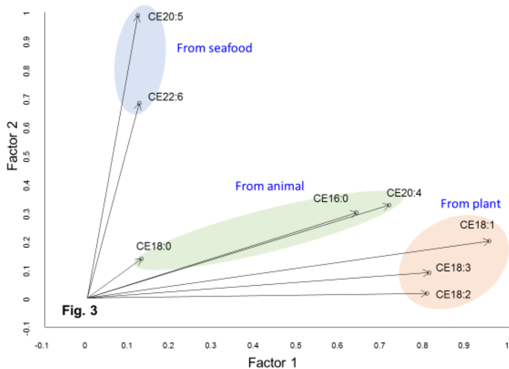
Fig.4.15 Result of CE dataset (factor analysis)
