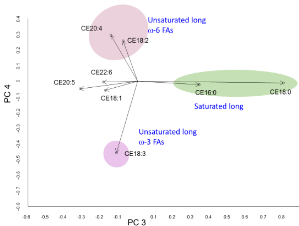
Fig.4.13 Result of CE dataset (PCA)
