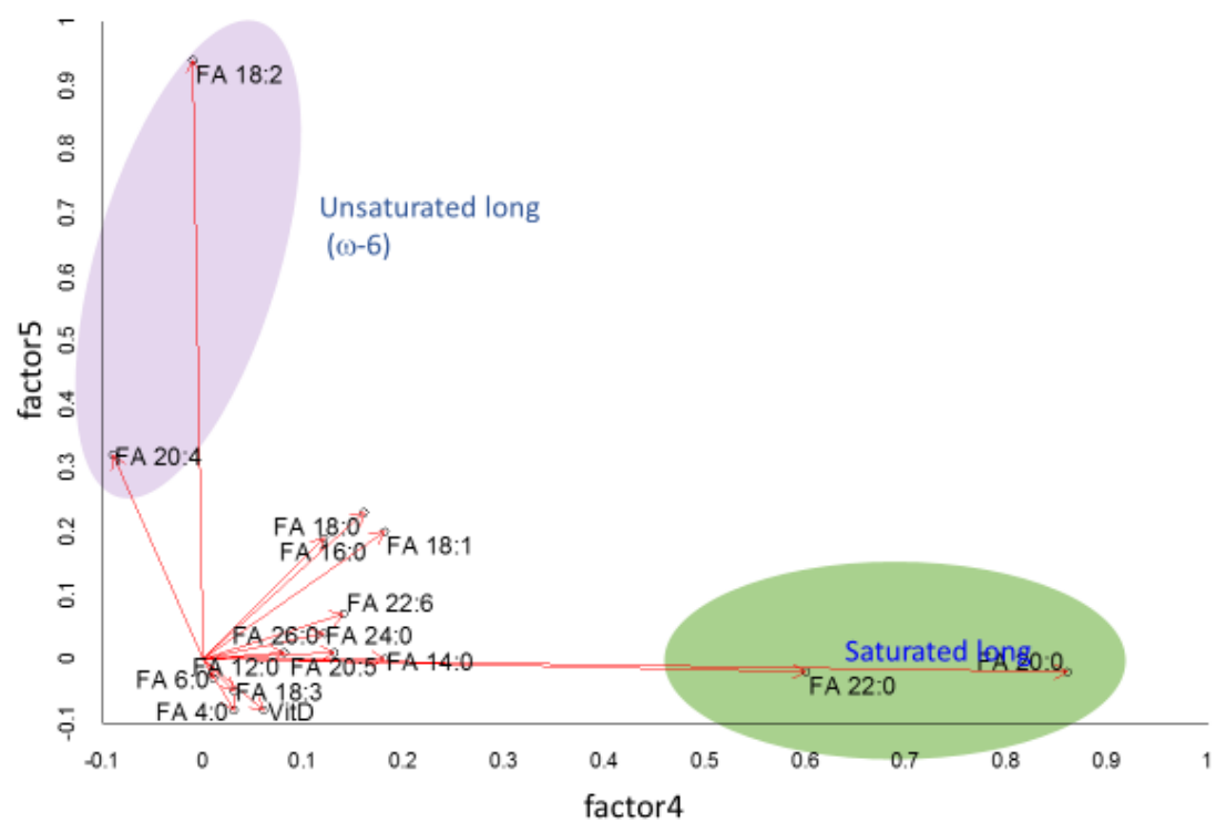
Fig.4.3 Result of total fatty acid dataset (factor analysis)
