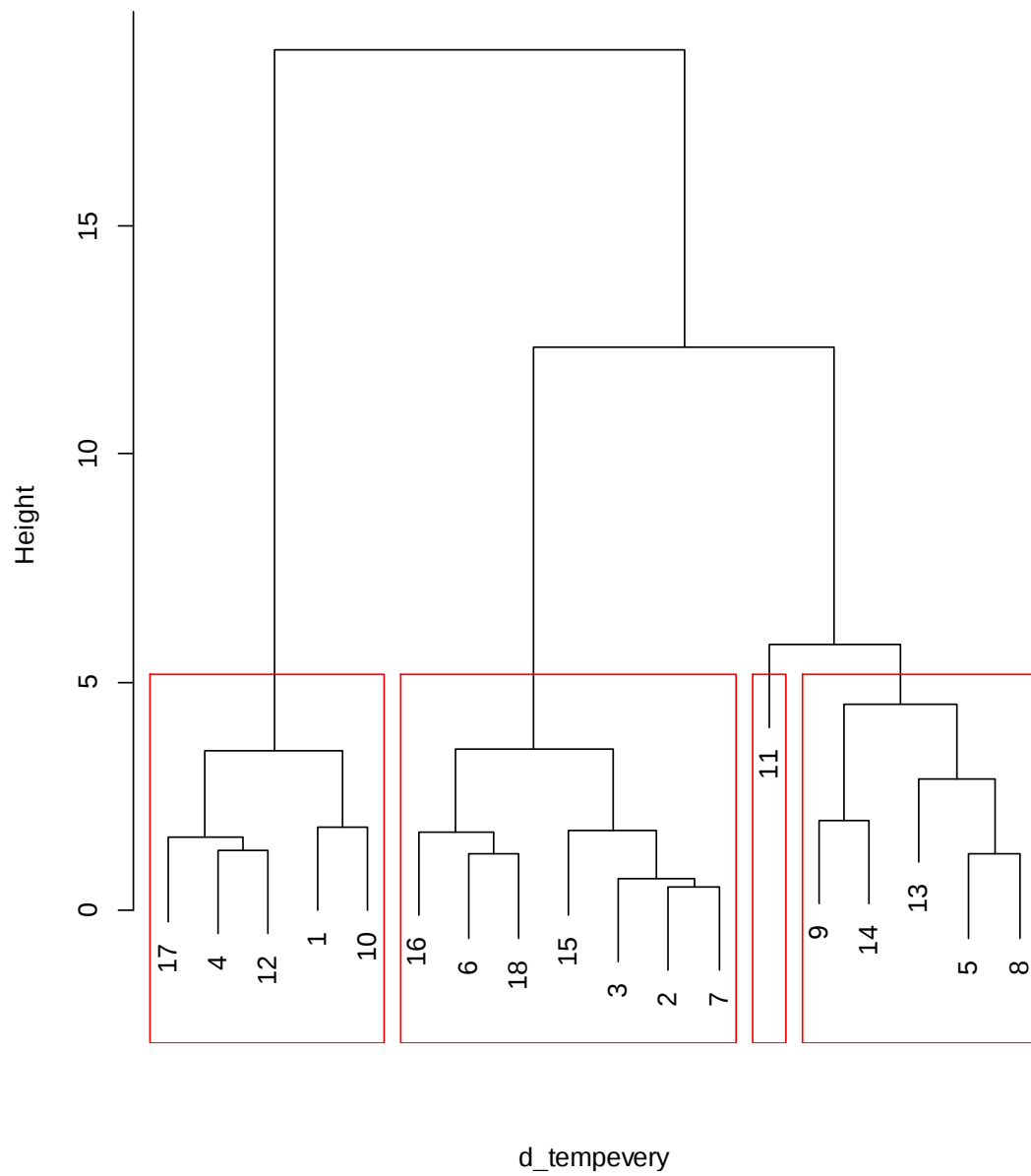
Fig.5.5 Clustering for average temperature everyday
