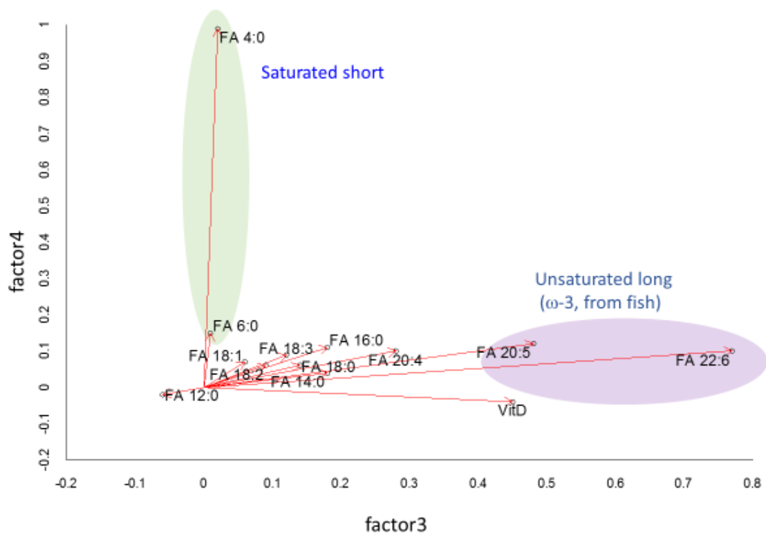
Fig.4.5 Result of free fatty acid dataset (factor analysis)
