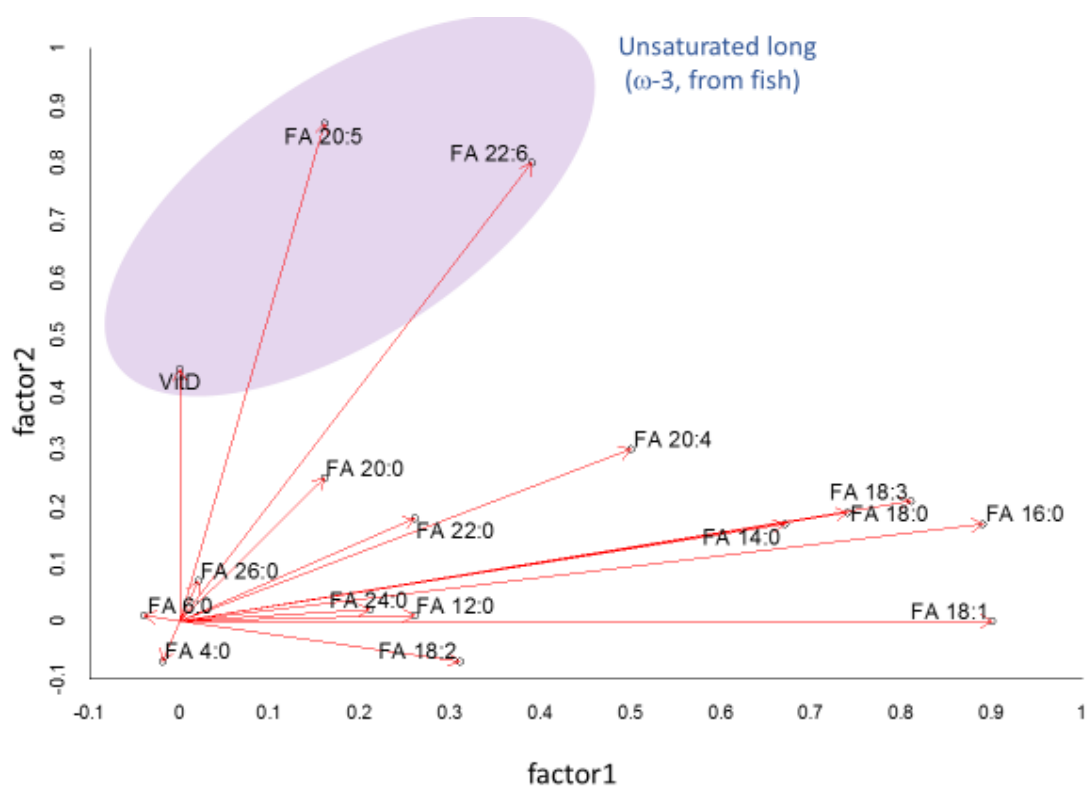
Fig.4.1 Result of total fatty acid dataset (factor analysis)
