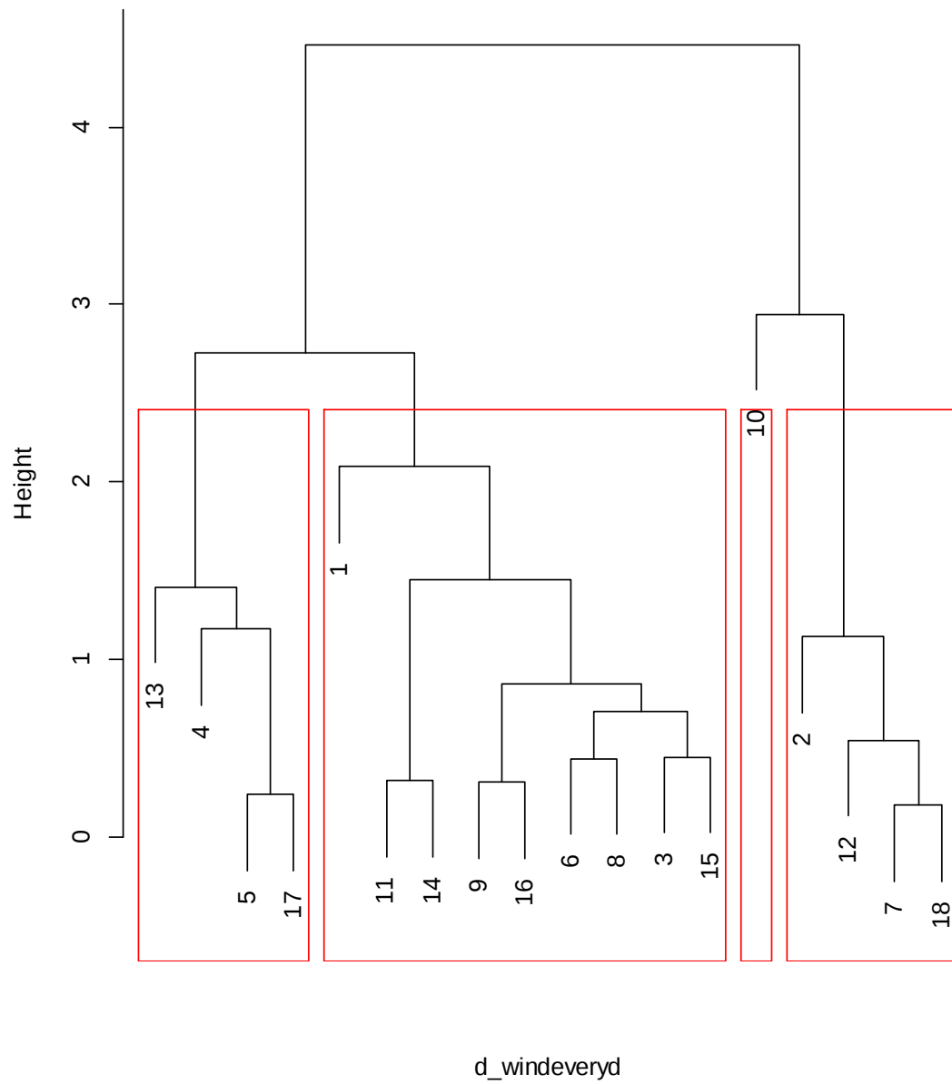
Fig.5.7 Clustering for wind speed everyday derivatives
