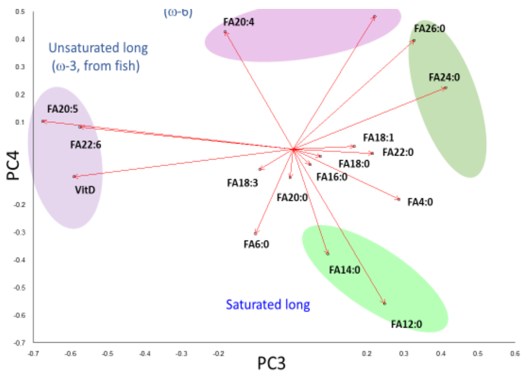
Fig.4.6 Result of total fatty acid dataset (PCA)
